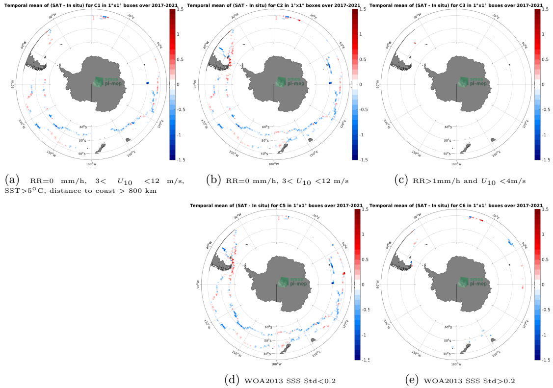
Figure 12: Temporal mean gridded over spatial boxes of size 1°x1° of \Delta SSS (SMAP SSS L3 v5 - 8-Day running (RSS) - TSG (GOSUD-Sailing-ship)) for 5 different subdatasets corresponding to:RR=0 mm/h, 3 < U_{10} < 12 m/s, SST>5°C, distance to coast > 800 km (a), RR=0 mm/h, 3 < U_{10} < 12 m/s (b), RR>1mm/h and U_{10} < 4 m/s (c), WOA2013 SSS Std<0.2 (d), WOA2013 SSS Std>0.2 (e).
