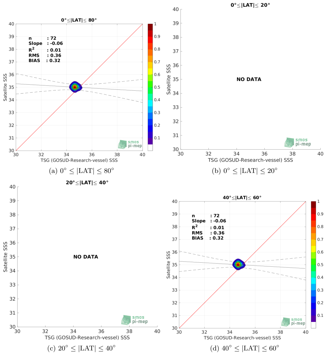
Figure 9: Contour maps of the concentration of SMAP SSS L3 v5 - 8-Day running (RSS) SSS (y-axis) versus TSG (GOSUD-Research-vessel) SSS (x-axis) at match-up pairs for different latitude bands. For each plot, the red line shows x=y . The black thin and dashed lines indicate a linear fit through the data cloud and the \pm 95\% confidence levels, respectively. The number match-up pairs n , the slope and R^2 coefficient of the linear fit, the root mean square (RMS) and the mean bias between satellite and in situ data are indicated for each latitude band in each plots.
