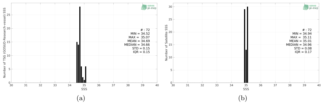
Figure 2: Histograms of SSS from TSG (GOSUD-Research-vessel) (a) and SMAP SSS L3 v5 - 8-Day running (RSS) (b) considering all match-up pairs per bins of 0.1 over the Roaring Forties and Furious Fifties Pi-MEP region and for the full satellite product period.
