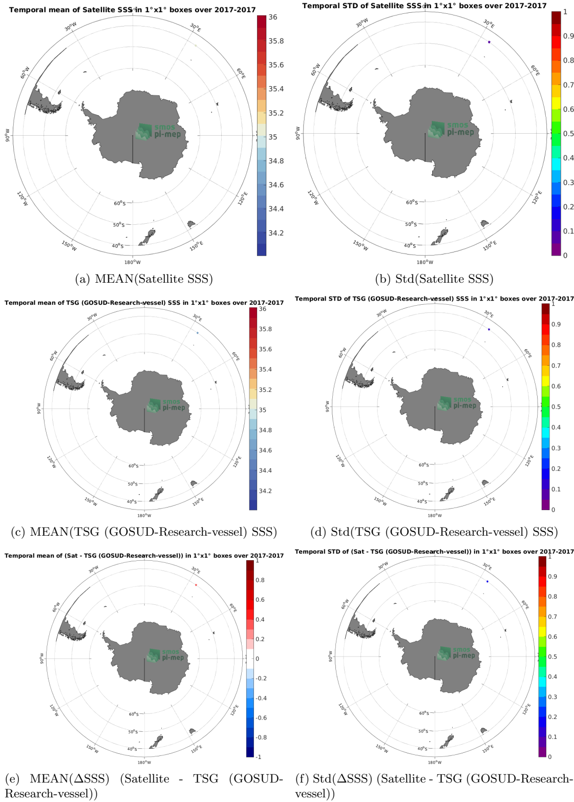
Figure 6: Temporal mean (left) and Std (right) of SSS from SMAP SSS L3 v5 - 8-Day running (RSS) (top), TSG (GOSUD-Research-vessel) (middle), and of \Delta SSS (Satellite - TSG (GOSUD-Research-vessel)). Only match-up pairs are used to generate these maps.
