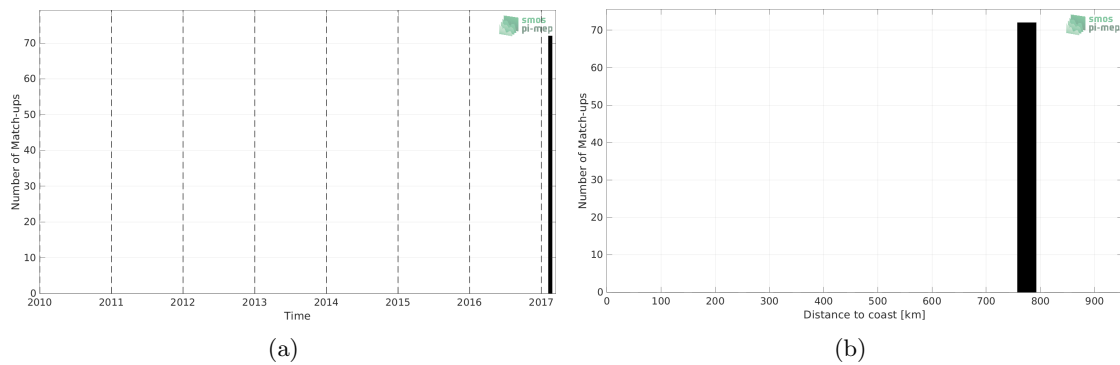
Figure 1: Number of match-ups between TSG (GOSUD-Research-vessel) and SMAP SSS L3 v5 - 8-Day running (RSS) SSS as a function of time (a) and as function of the distance to coast (b) over the Roaring Forties and Furious Fifties Pi-MEP region and for the full satellite product period.
