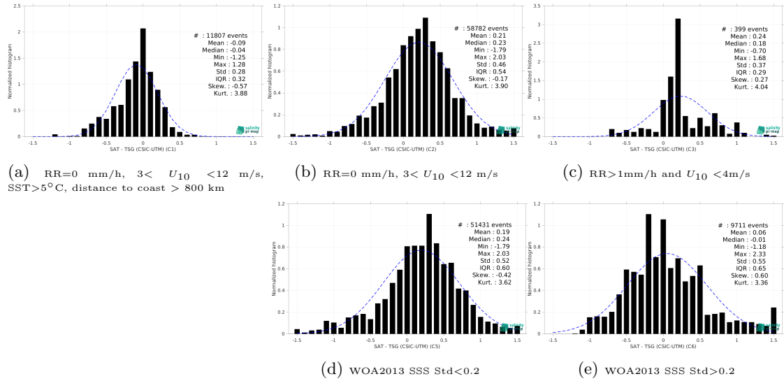
Figure 13: Normalized histogram of \Delta SSS (SMAP SSS L3 v5 - 8-Day running (RSS) - TSG (CSIC-UTM)) for 5 different subdatasets corresponding to: RR=0 mm/h, 3 < U_{10} < 12 m/s, SST>5°C, distance to coast > 800 km (a), RR=0 mm/h, 3 < U_{10} < 12 m/s (b), RR>1mm/h and U_{10} < 4 m/s (c), WOA2013 SSS Std<0.2 (d), WOA2013 SSS Std>0.2 (e).
