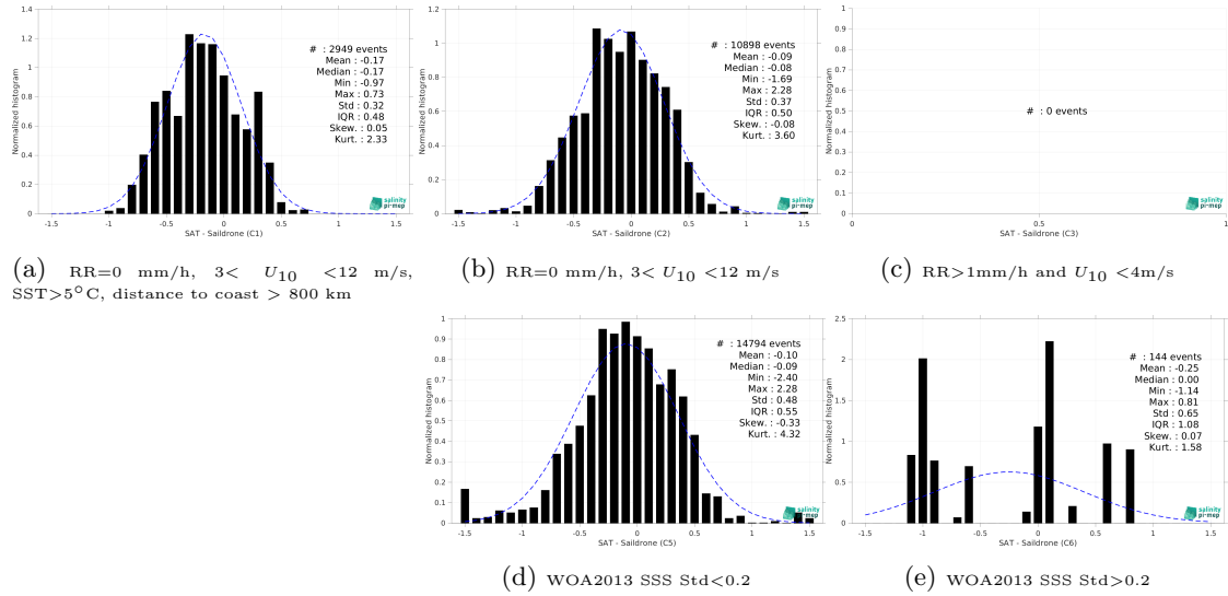
Figure 13: Normalized histogram of \Delta SSS (SMAP SSS L3 v5 - 8-Day running (RSS) - Saildrone) for 5 different subdatasets corresponding to: RR=0 mm/h, 3 < U_{10} < 12 m/s, SST > 5°C, distance to coast > 800 km (a), RR=0 mm/h, 3 < U_{10} < 12 m/s (b), RR > 1mm/h and U_{10} < 4 m/s (c), WOA2013 SSS Std < 0.2 (d), WOA2013 SSS Std > 0.2 (e).
