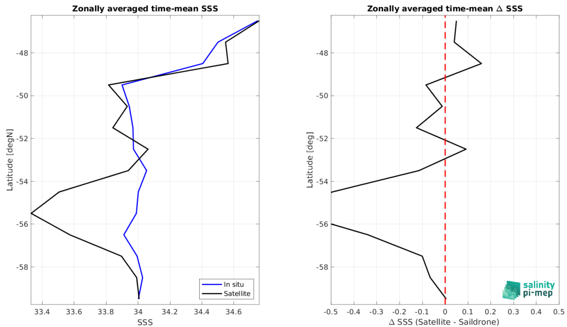
Figure 8: Left panel: Zonal mean SSS from SMAP SSS L3 v5 - 8-Day running (RSS) satellite product (black) and from Sairdron (blue). Right panel: Zonal mean of \Delta SSS (Satellite - Sairdron) for all the collected Pi-MEP match-up pairs estimated over the full satellite product period.
