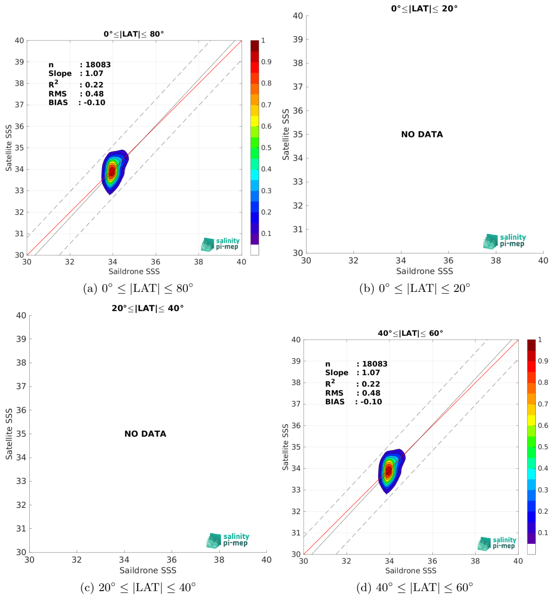
Figure 9: Contour maps of the concentration of SMAP SSS L3 v5 - 8-Day running (RSS) SSS (y-axis) versus Saildrone SSS (x-axis) at match-up pairs for different latitude bands. For each plot, the red line shows x=y . The black thin and dashed lines indicate a linear fit through the data cloud and the \pm 95\% confidence levels, respectively. The number match-up pairs n , the slope and R^2 coefficient of the linear fit, the root mean square (RMS) and the mean bias between satellite and in situ data are indicated for each latitude band in each plots.
