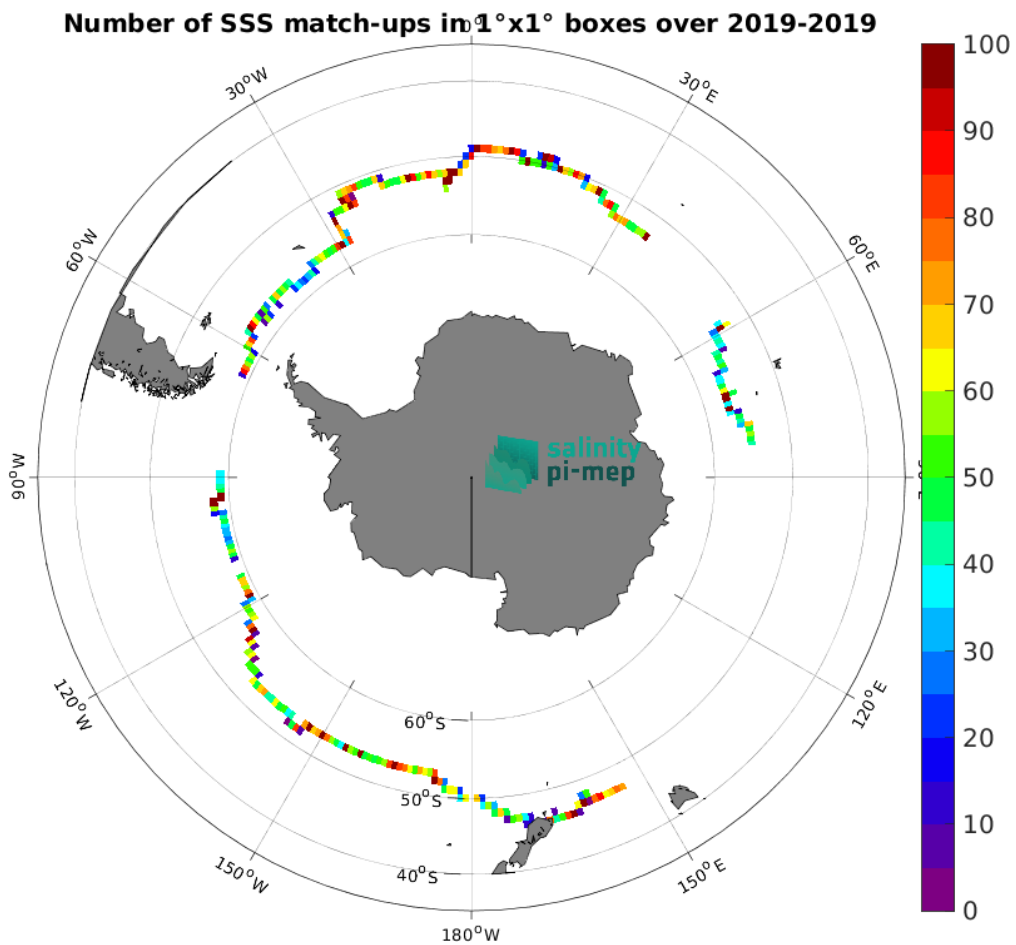
Figure 4: Number of SSS match-ups between Saildrone SSS and the SMAP SSS L3 v5 - 8-Day running (RSS) SSS product for the Roaring Forties and Furious Fifties Pi-MEP region over 1^\circ \times 1^\circ boxes and for the full satellite product period.
