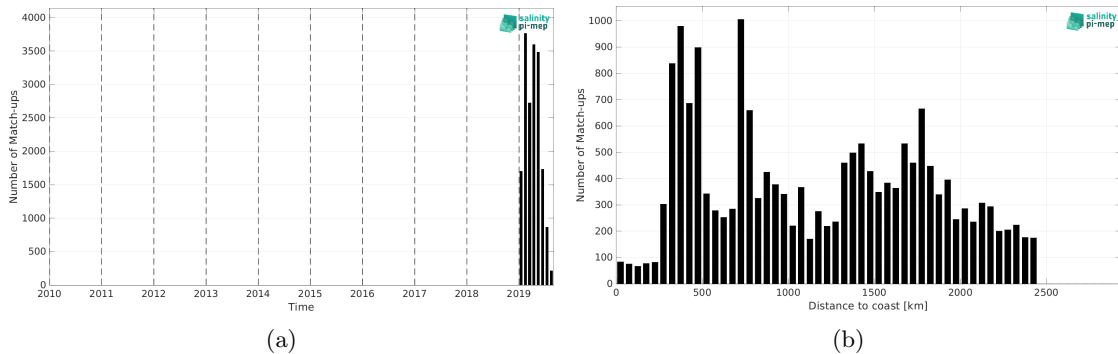
Figure 1: Number of match-ups between Saildrone and SMAP SSS L3 v5 - 8-Day running (RSS) SSS as a function of time (a) and as function of the distance to coast (b) over the Roaring Forties and Furious Fifties Pi-MEP region and for the full satellite product period.
