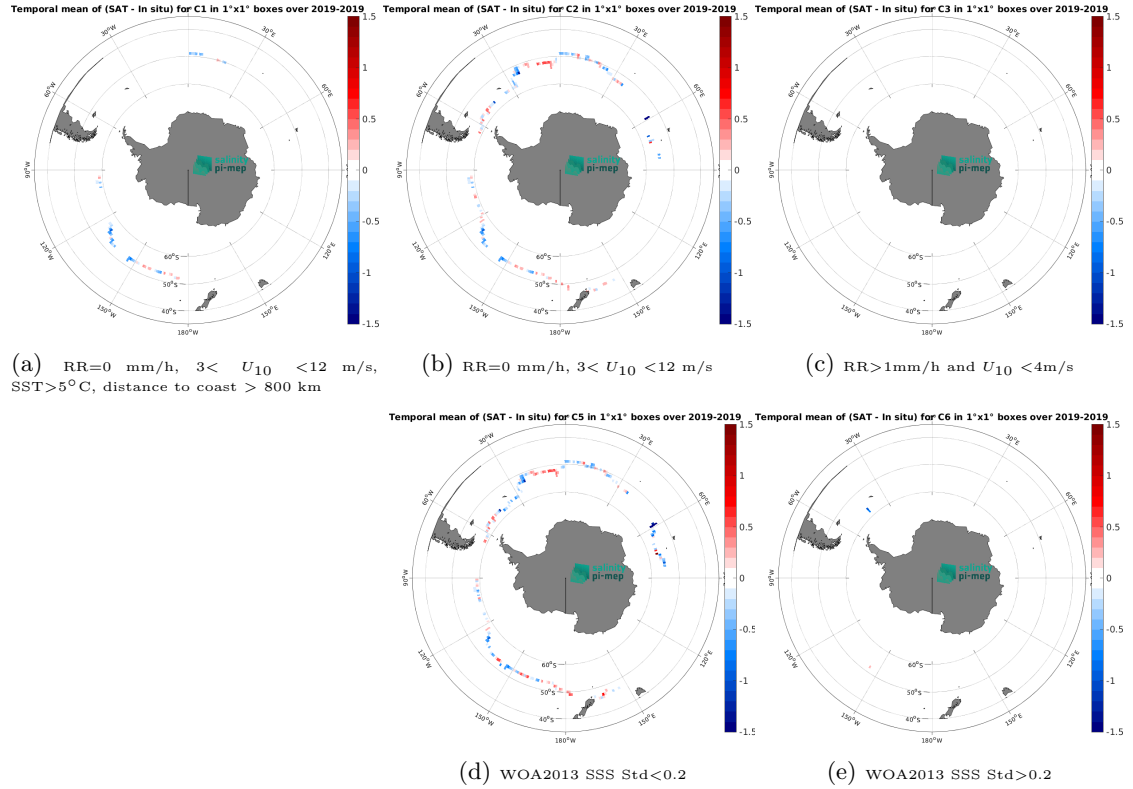
Figure 12: Temporal mean gridded over spatial boxes of size 1^{\circ}\times 1^{\circ} of \Delta\text{SSS} (SMAP SSS L3 v5 - 8-Day running (RSS) - Saildrone) for 5 different subdatasets corresponding to:RR=0 mm/h, 3 < U_{10} < 12 m/s, SST > 5^{\circ}\text{C} , distance to coast > 800 km (a), RR=0 mm/h, 3 < U_{10} < 12 m/s (b), RR > 1 mm/h and U_{10} < 4 m/s (c), WOA2013 SSS Std < 0.2 (d), WOA2013 SSS Std > 0.2 (e).
