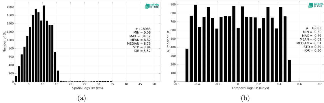
Figure 5: Histograms of the spatial (a) and temporal (b) lags between the location/time of the Saildrone measurement and the date of the corresponding SMAP SSS L3 v5 - 8-Day running (RSS) SSS pixel.
