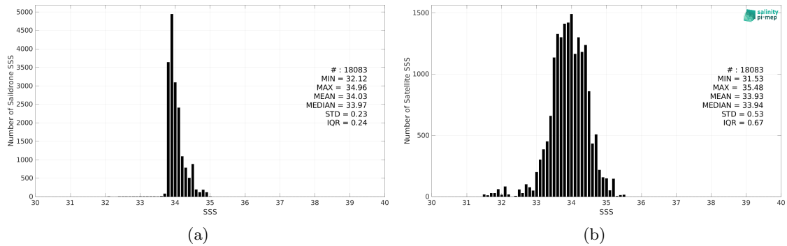
Figure 2: Histograms of SSS from Saildrone (a) and SMAP SSS L3 v5 - 8-Day running (RSS) (b) considering all match-up pairs per bins of 0.1 over the Roaring Forties and Furious Fifties Pi-MEP region and for the full satellite product period.
