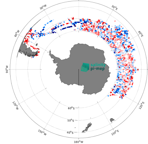
(e) MEAN( \Delta SSS) (Satellite - Marine mammals)
