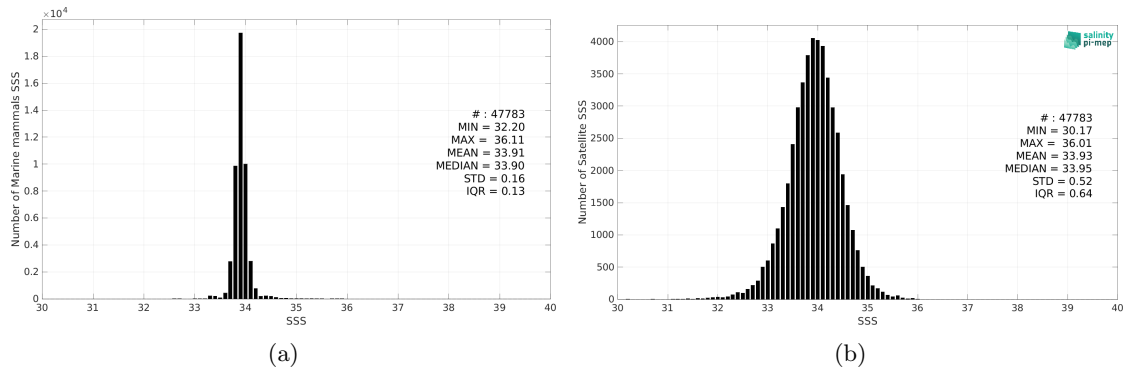
Figure 2: Histograms of SSS from Marine mammals (a) and SMAP SSS L3 v5 - 8-Day running (RSS) (b) considering all match-up pairs per bins of 0.1 over the Roaring Forties and Furious Fifties Pi-MEP region and for the full satellite product period.
