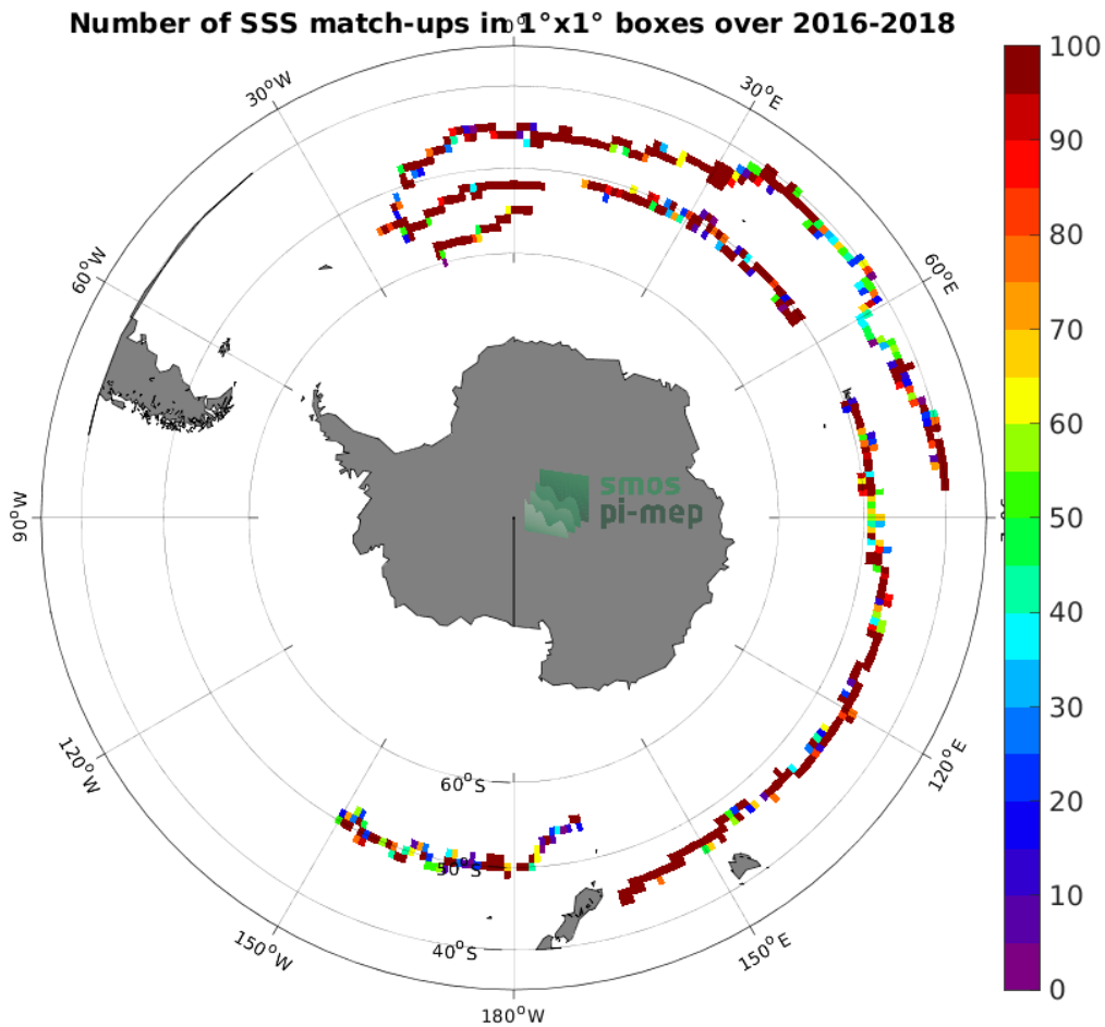
Figure 3: Number of SSS match-ups between Surface drifters SSS and the SMAP SSS L3 v5 - 8-Day running (RSS) SSS product for the Roaring Forties and Furious Fifties Pi-MEP region over 1^\circ \times 1^\circ boxes and for the full satellite product period.
