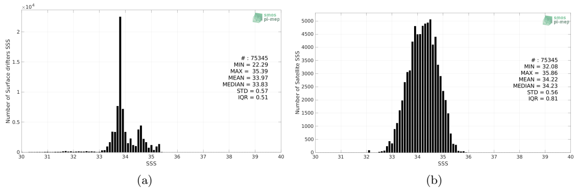
Figure 2: Histograms of SSS from Surface drifters (a) and SMAP SSS L3 v5 - 8-Day running (RSS) (b) considering all match-up pairs per bins of 0.1 over the Roaring Forties and Furious Fifties Pi-MEP region and for the full satellite product period.
