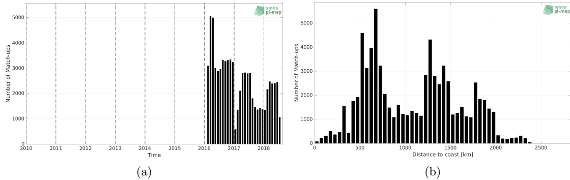
Figure 1: Number of match-ups between Surface drifters and SMAP SSS L3 v5 - 8-Day running (RSS) SSS as a function of time (a) and as function of the distance to coast (b) over the Roaring Forties and Furious Fifties Pi-MEP region and for the full satellite product period.
