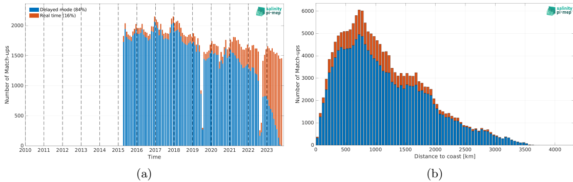
Figure 1: Number of match-ups between Argo and SMAP SSS L3 v5 - 8-Day running (RSS) SSS as a function of time (a) and as function of the distance to coast (b) over the Roaring Forties and Furious Fifties Pi-MEP region and for the full satellite product period.
