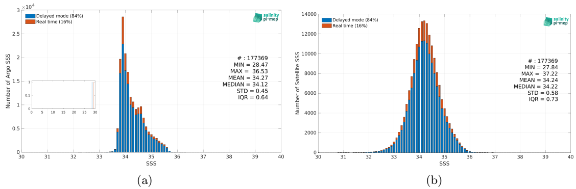
Figure 2: Histograms of SSS from Argo (a) and SMAP SSS L3 v5 - 8-Day running (RSS) (b) considering all match-up pairs per bins of 0.1 over the Roaring Forties and Furious Fifties Pi-MEP region and for the full satellite product period.
