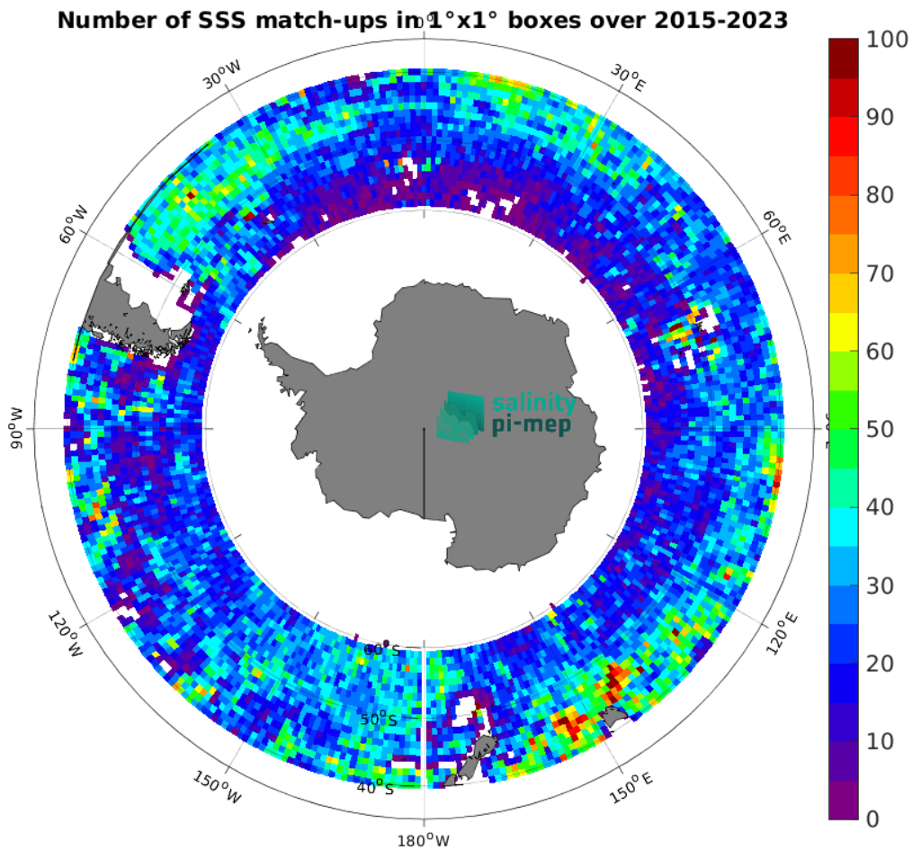
Figure 4: Number of SSS match-ups between Argo SSS and the SMAP SSS L3 v5 - 8-Day running (RSS) SSS product for the Roaring Forties and Furious Fifties Pi-MEP region over 1^\circ \times 1^\circ boxes and for the full satellite product period.
