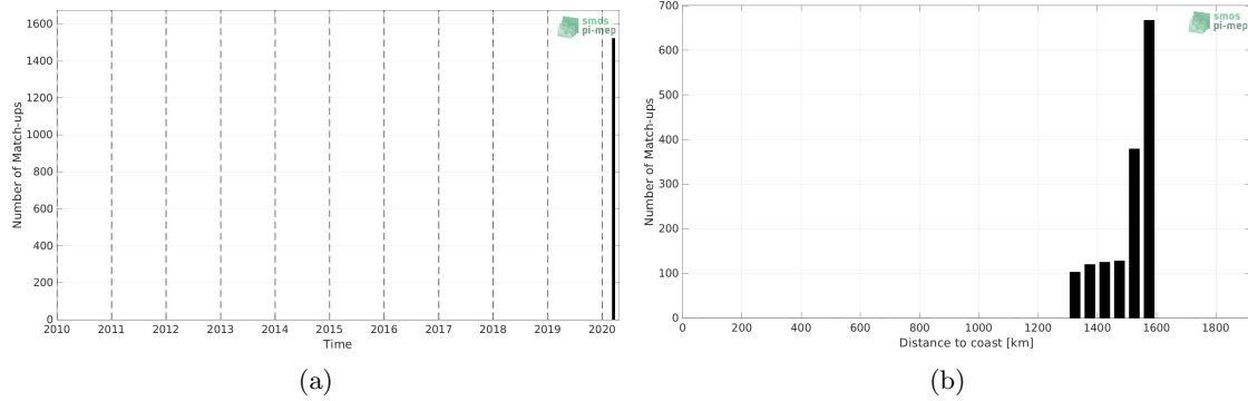
Figure 1: Number of match-ups between TSG (SAMOS) and SMAP SSS L3 v5 - Monthly (RSS) SSS as a function of time (a) and as function of the distance to coast (b) over the Roaring Forties and Furious Fifties Pi-MEP region and for the full satellite product period.
