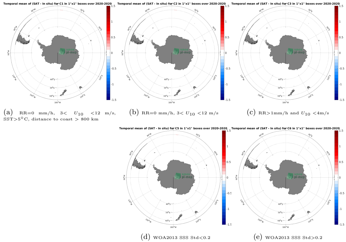
Figure 12: Temporal mean gridded over spatial boxes of size 1^{\circ}\times 1^{\circ} of \Delta\text{SSS} (SMAP SSS L3 v5 - Monthly (RSS) - TSG (SAMOS)) for 5 different subdatasets corresponding to:RR=0 mm/h, 3 < U_{10} < 12 m/s, SST >5^{\circ}\text{C} , distance to coast > 800 km (a), RR=0 mm/h, 3 < U_{10} < 12 m/s (b), RR >1 mm/h and U_{10} < 4 m/s (c), WOA2013 SSS Std <0.2 (d), WOA2013 SSS Std >0.2 (e).
