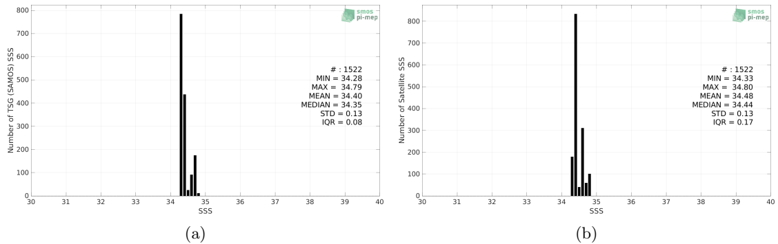
Figure 2: Histograms of SSS from TSG (SAMOS) (a) and SMAP SSS L3 v5 - Monthly (RSS) (b) considering all match-up pairs per bins of 0.1 over the Roaring Forties and Furious Fifties Pi-MEP region and for the full satellite product period.
