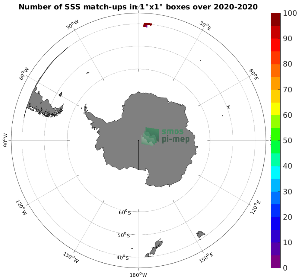
Figure 4: Number of SSS match-ups between TSG (SAMOS) SSS and the SMAP SSS L3 v5 - Monthly (RSS) SSS product for the Roaring Forties and Furious Fifties Pi-MEP region over 1^\circ \times 1^\circ boxes and for the full satellite product period.
