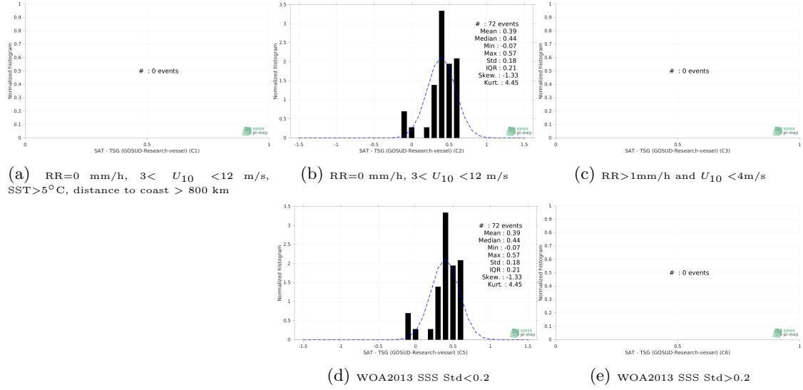
Figure 13: Normalized histogram of \Delta SSS (SMAP SSS L3 v5 - Monthly (RSS) - TSG (GOSUD-Research-vessel)) for 5 different subdatasets corresponding to: RR=0 mm/h, 3 < U_{10} < 12 m/s, SST >5^{\circ}\text{C} , distance to coast > 800 km (a), RR=0 mm/h, 3 < U_{10} < 12 m/s (b), RR >1 mm/h and U_{10} < 4 m/s (c), WOA2013 SSS Std <0.2 (d), WOA2013 SSS Std >0.2 (e).
