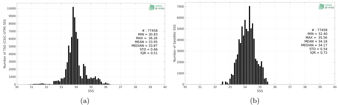
Figure 2: Histograms of SSS from TSG (CSIC-UTM) (a) and SMAP SSS L3 v5 - Monthly (RSS) (b) considering all match-up pairs per bins of 0.1 over the Roaring Forties and Furious Fifties Pi-MEP region and for the full satellite product period.
