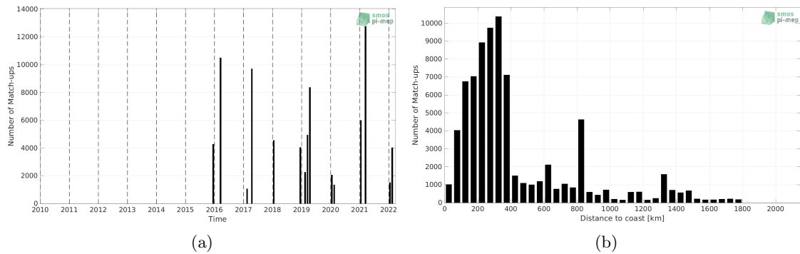
Figure 1: Number of match-ups between TSG (CSIC-UTM) and SMAP SSS L3 v5 - Monthly (RSS) SSS as a function of time (a) and as function of the distance to coast (b) over the Roaring Forties and Furious Fifties Pi-MEP region and for the full satellite product period.
