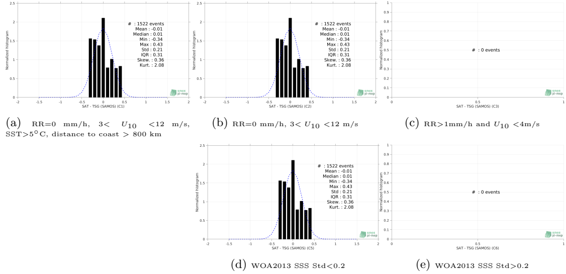
Figure 13: Normalized histogram of \Delta SSS (SMAP SSS L3 v4 - 8-Day running (RSS) - TSG (SAMOS)) for 5 different subdatasets corresponding to: RR=0 mm/h, 3 < U_{10} < 12 m/s, SST >5^{\circ} C, distance to coast > 800 km (a), RR=0 mm/h, 3 < U_{10} < 12 m/s (b), RR >1 mm/h and U_{10} < 4 m/s (c), WOA2013 SSS Std <0.2 (d), WOA2013 SSS Std >0.2 (e).
