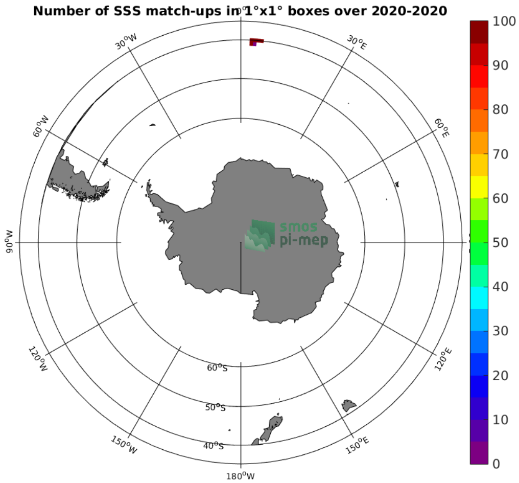
Figure 4: Number of SSS match-ups between TSG (SAMOS) SSS and the SMAP SSS L3 v4 - 8-Day running (RSS) SSS product for the Roaring Forties and Furious Fifties Pi-MEP region over 1^\circ \times 1^\circ boxes and for the full satellite product period.
