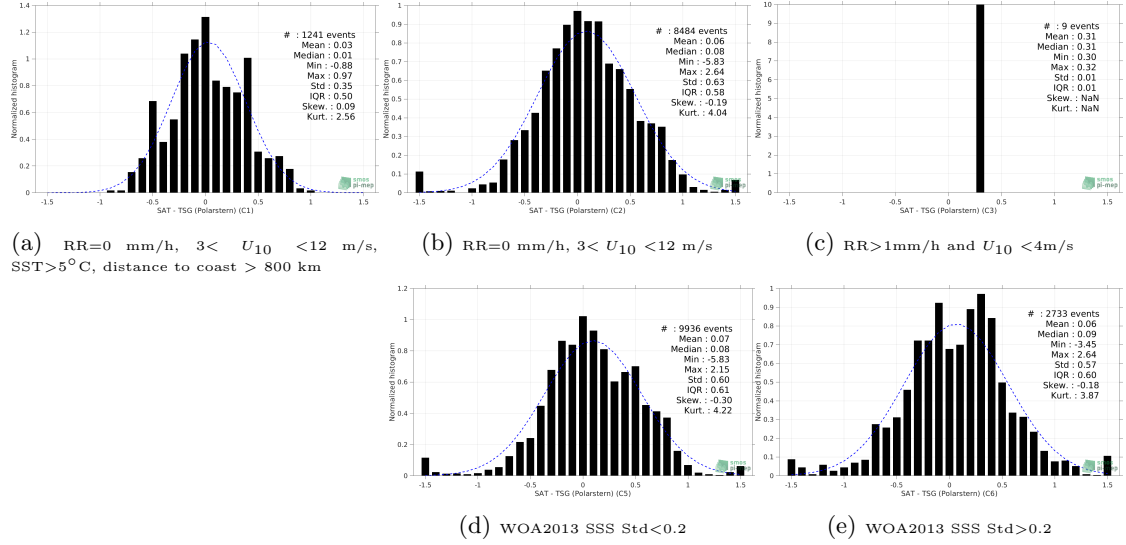
Figure 13: Normalized histogram of \Delta SSS (SMAP SSS L3 v4 - 8-Day running (RSS) - TSG (Polarstern)) for 5 different subdatasets corresponding to: RR=0 mm/h, 3 < U_{10} < 12 m/s, SST > 5°C, distance to coast > 800 km (a), RR=0 mm/h, 3 < U_{10} < 12 m/s (b), RR > 1mm/h and U_{10} < 4 m/s (c), WOA2013 SSS Std < 0.2 (d), WOA2013 SSS Std > 0.2 (e).
