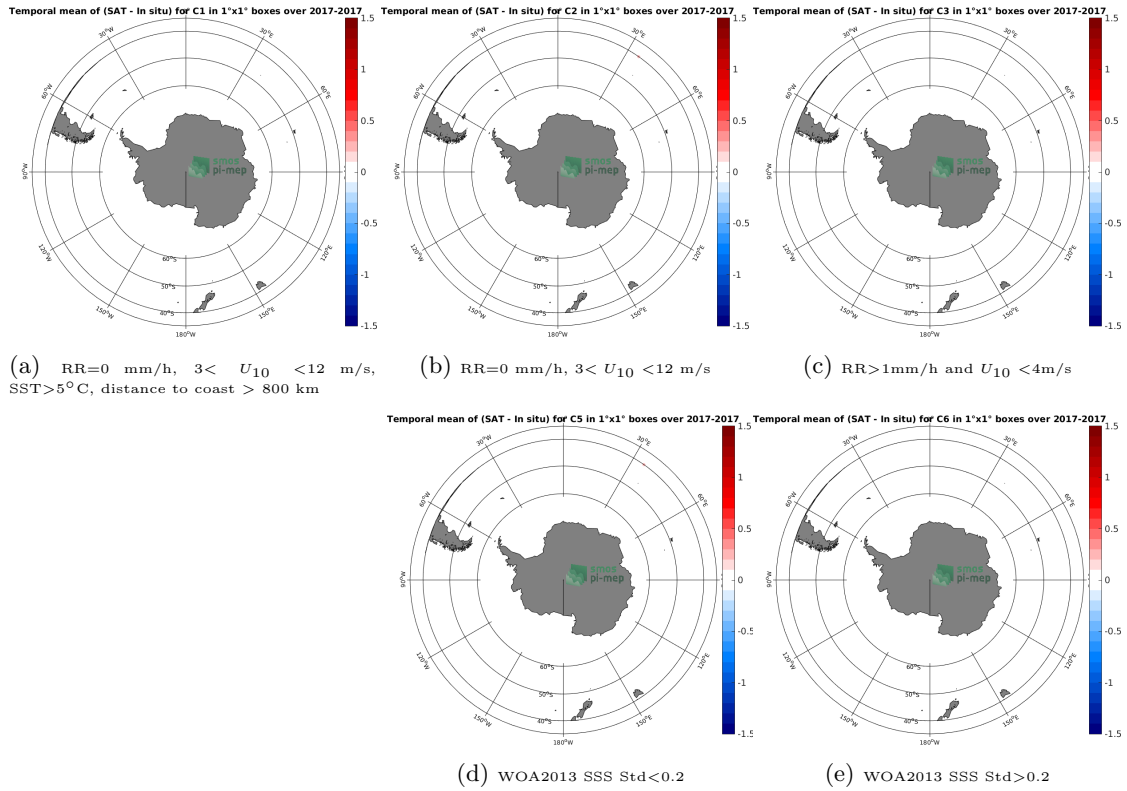
Figure 12: Temporal mean gridded over spatial boxes of size 1^\circ \times 1^\circ of \Delta SSS (SMAP SSS L3 v4 - 8-Day running (RSS) - TSG (GOSUD-Research-vessel)) for 5 different subdatasets corresponding to: RR=0 mm/h, 3 < U_{10} < 12 m/s, SST>5°C, distance to coast > 800 km (a), RR=0 mm/h, 3 < U_{10} < 12 m/s (b), RR>1mm/h and U_{10} < 4 m/s (c), WOA2013 SSS Std<0.2 (d), WOA2013 SSS Std>0.2 (e).
