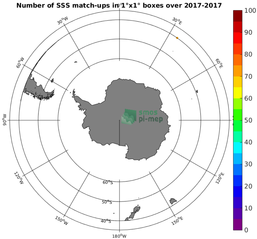
Figure 4: Number of SSS match-ups between TSG (GOSUD-Research-vessel) SSS and the SMAP SSS L3 v4 - 8-Day running (RSS) SSS product for the Roaring Forties and Furious Fifties Pi-MEP region over 1^\circ \times 1^\circ boxes and for the full satellite product period.
