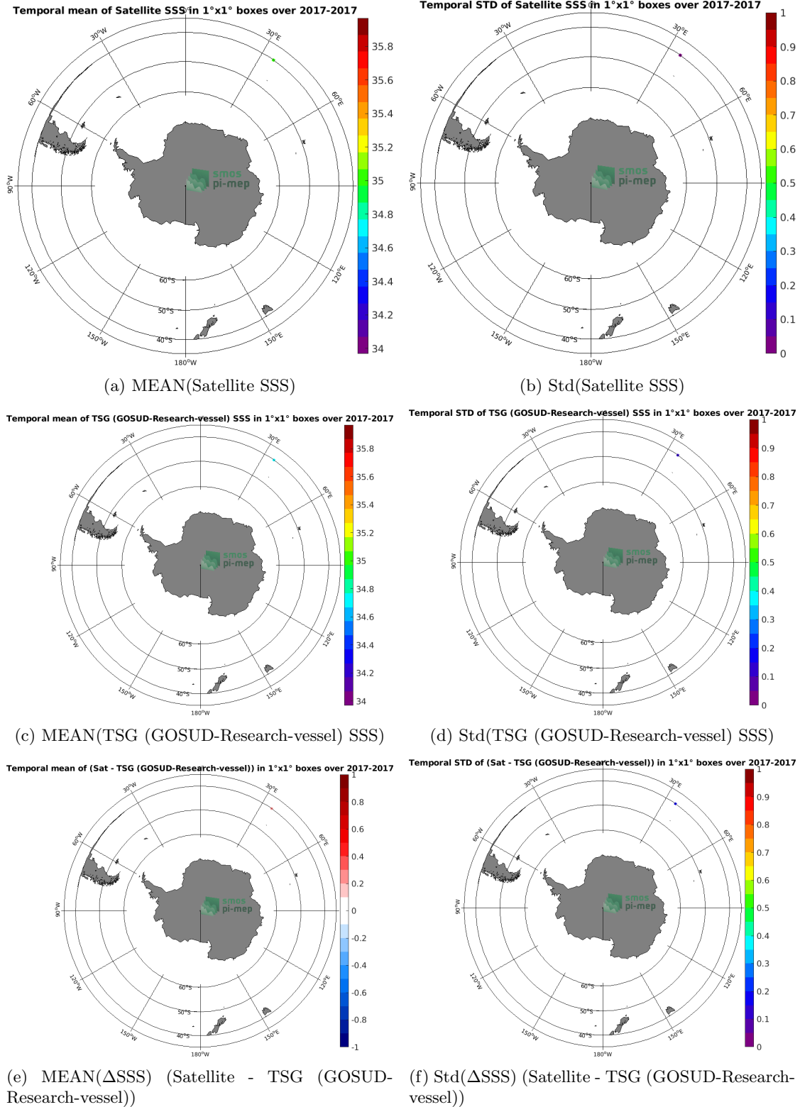
Figure 6: Temporal mean (left) and Std (right) of SSS from SMAP SSS L3 v4 - 8-Day running (RSS) (top), TSG (GOSUD-Research-vessel) (middle), and of \Delta SSS (Satellite - TSG (GOSUD-Research-vessel)). Only match-up pairs are used to generate these maps.
