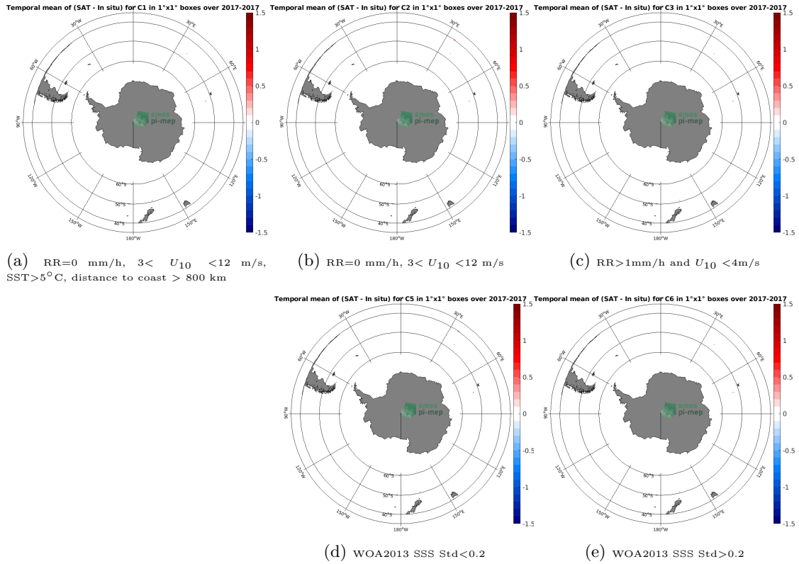
Figure 12: Temporal mean gridded over spatial boxes of size 1°x1° of \Delta SSS (SMAP SSS L3 v4 - 8-Day running (RSS) - TSG (GOSUD-Research-vessel)) for 5 different subdatasets corresponding to:RR=0 mm/h, 3 < U_{10} < 12 m/s, SST>5°C, distance to coast > 800 km (a), RR=0 mm/h, 3 < U_{10} < 12 m/s (b), RR>1mm/h and U_{10} < 4 m/s (c), WOA2013 SSS Std<0.2 (d), WOA2013 SSS Std>0.2 (e).
