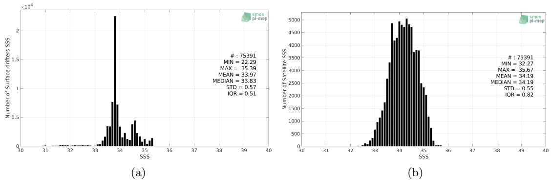
Figure 2: Histograms of SSS from Surface drifters (a) and SMAP SSS L3 v4 - 8-Day running (RSS) (b) considering all match-up pairs per bins of 0.1 over the Roaring Forties and Furious Fifties Pi-MEP region and for the full satellite product period.
