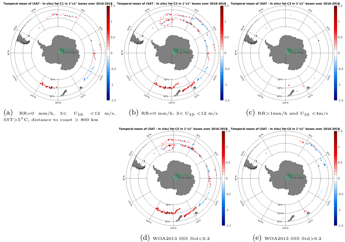
Figure 11: Temporal mean gridded over spatial boxes of size 1^{\circ}\times 1^{\circ} of \Delta\text{SSS} (SMAP SSS L3 v4 - 8-Day running (RSS) - Surface drifters) for 5 different subdatasets corresponding to:RR=0 mm/h, 3 < U_{10} < 12 m/s, SST >5^{\circ}\text{C} , distance to coast > 800 km (a), RR=0 mm/h, 3 < U_{10} < 12 m/s (b), RR >1 mm/h and U_{10} < 4 m/s (c), WOA2013 SSS Std <0.2 (d), WOA2013 SSS Std >0.2 (e).
