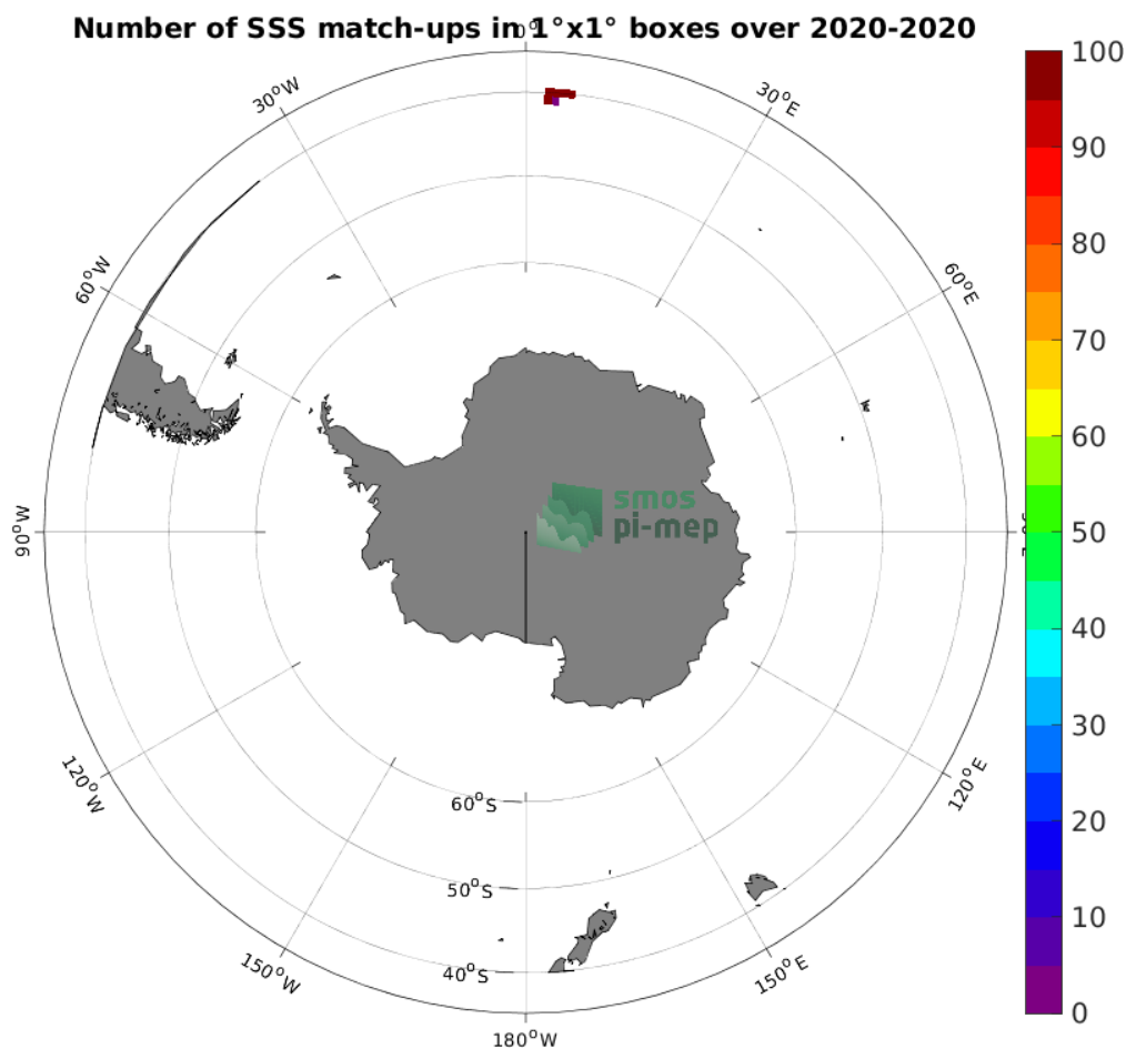
Figure 4: Number of SSS match-ups between TSG (SAMOS) SSS and the SMAP SSS L3 v4 - Monthly (RSS) SSS product for the Roaring Forties and Furious Fifties Pi-MEP region over 1^\circ \times 1^\circ boxes and for the full satellite product period.
