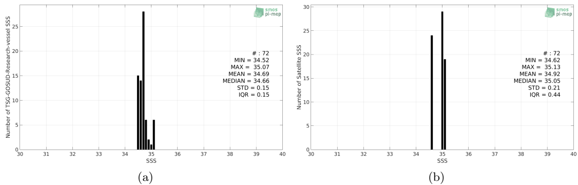
Figure 2: Histograms of SSS from TSG-GOSUD-Research-vessel (a) and SMAP-L3-RSS-V3-8DAY-RUNNING-40KM (b) considering all match-up pairs per bins of 0.1 over the Roaring Forties and Furious Fifties Pi-MEP region and for the full satellite product period.
