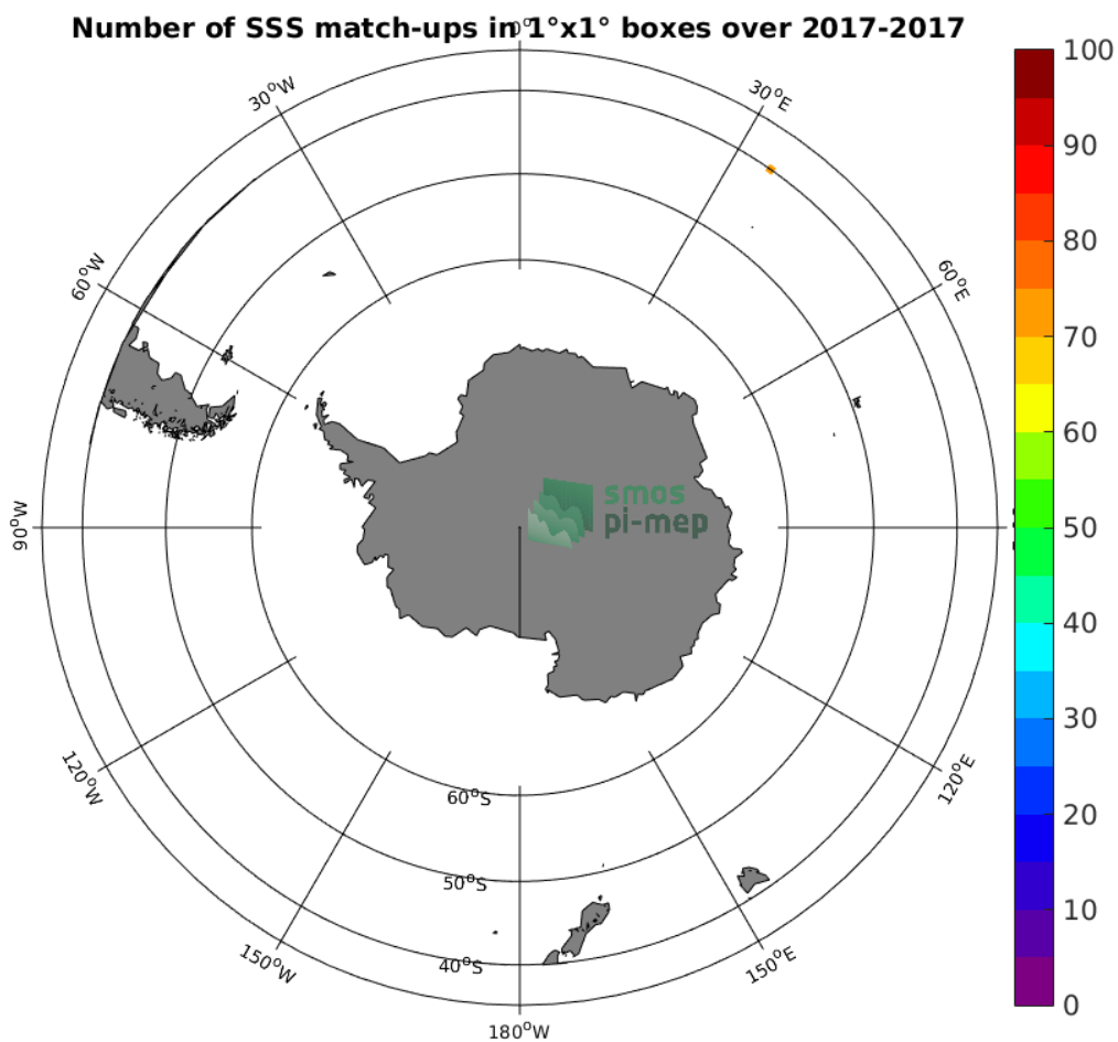
Figure 4: Number of SSS match-ups between TSG-GOSUD-Research-vessel SSS and the SMAP-L3-RSS-V3-8DAY-RUNNING-40KM SSS product for the Roaring Forties and Furious Fifties Pi-MEP region over 1^\circ \times 1^\circ boxes and for the full satellite product period.
