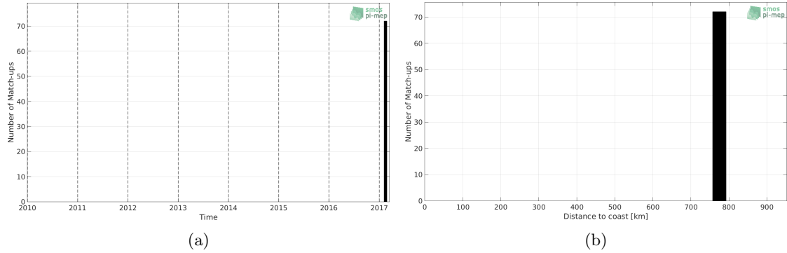
Figure 1: Number of match-ups between TSG-GOSUD-Research-vessel and SMAP-L3-RSS-V3-8DAY-RUNNING-40KM SSS as a function of time (a) and as function of the distance to coast (b) over the Roaring Forties and Furious Fifties Pi-MEP region and for the full satellite product period.
