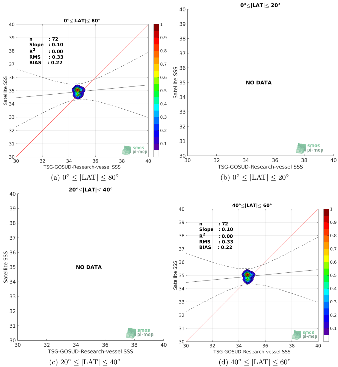
Figure 9: Contour maps of the concentration of SMAP-L3-RSS-V3-8DAY-RUNNING-40KM SSS (y-axis) versus TSG-GOSUD-Research-vessel SSS (x-axis) at match-up pairs for different latitude bands. For each plot, the red line shows x=y . The black thin and dashed lines indicate a linear fit through the data cloud and the \pm 95\% confidence levels, respectively. The number match-up pairs n , the slope and R^2 coefficient of the linear fit, the root mean square (RMS) and the mean bias between satellite and in situ data are indicated for each latitude band in each plots.
