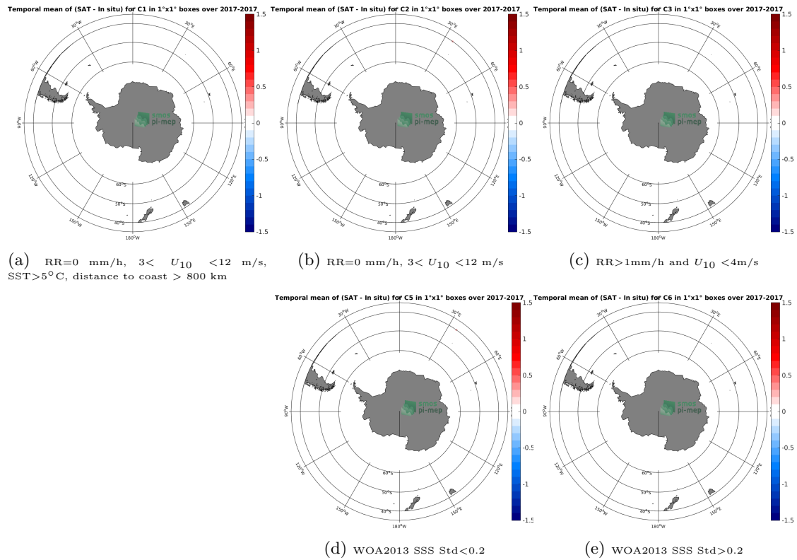
Figure 12: Temporal mean gridded over spatial boxes of size 1^\circ \times 1^\circ of \Delta SSS (SMAP-L3-RSS-V3-8DAY-RUNNING-40KM - TSG-GOSUD-Research-vessel) for 5 different subdatasets corresponding to:RR=0 mm/h, 3 < U_{10} < 12 m/s, SST >5^\circ C, distance to coast > 800 km (a), RR=0 mm/h, 3 < U_{10} < 12 m/s (b), RR >1 mm/h and U_{10} < 4 m/s (c), WOA2013 SSS Std <0.2 (d), WOA2013 SSS Std >0.2 (e).
