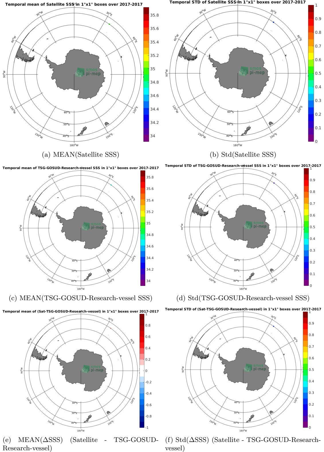
Figure 6: Temporal mean (left) and Std (right) of SSS from SMAP-L3-RSS-V3-8DAY-RUNNING-40KM (top), TSG-GOSUD-Research-vessel (middle), and of \Delta SSS (Satellite - TSG-GOSUD-Research-vessel). Only match-up pairs are used to generate these maps.
