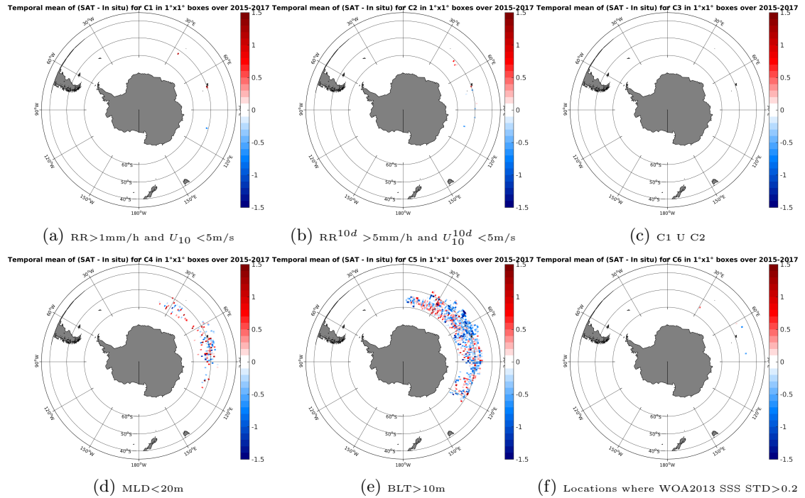
Figure 12: Temporal mean gridded over spatial boxes of size 1^\circ \times 1^\circ of \Delta SSS (SMAP-L3-RSS-V2-8DAY-RUNNING-40KM - Sea mammals) for 6 different subdatasets corresponding to: RR > 1\text{mm/h} and U_{10} < 5\text{m/s} (a), RR^{10d} > 5\text{mm/h} and U_{10}^{10d} < 5\text{m/s} (b), C1 U C2 (c), MLD < 20\text{m} (d), BLT > 10\text{m} (e), Locations where WOA2013 SSS STD > 0.2 (f).
