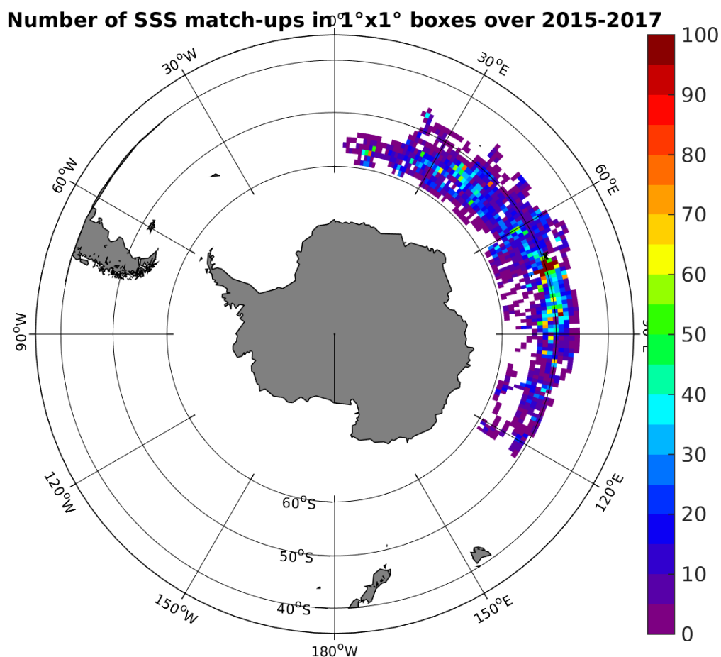
Figure 4: Number of SSS match-ups between Sea mammals SSS and the SMAP-L3-RSS-V2-8DAY-RUNNING-40KM SSS product for the Roaring Forties and Furious Fifties Pi-MEP region over 1^\circ \times 1^\circ boxes and for the full satellite product period.
