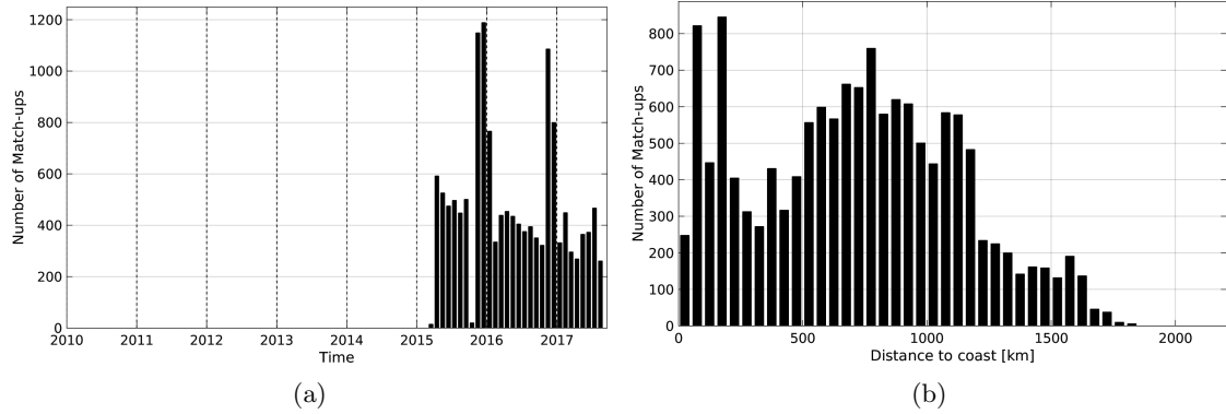
Figure 1: Number of match-ups between Sea mammals and SMAP-L3-RSS-V2-8DAY-RUNNING-40KM SSS as a function of time (a) and as function of the distance to coast (b) over the Roaring Forties and Furious Fifties Pi-MEP region and for the full satellite product period.
