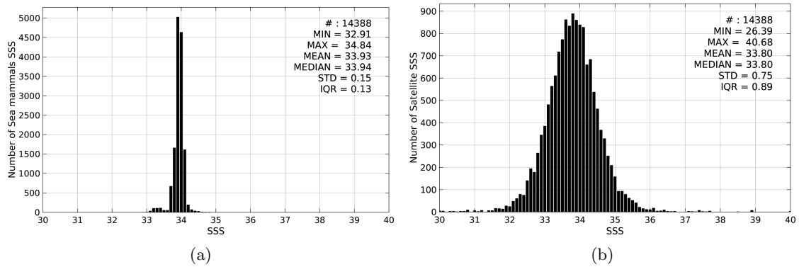
Figure 2: Histograms of SSS from Sea mammals (a) and SMAP-L3-RSS-V2-8DAY-RUNNING-40KM (b) considering all match-up pairs per bins of 0.1 over the Roaring Forties and Furious Fifties Pi-MEP region and for the full satellite product period.
