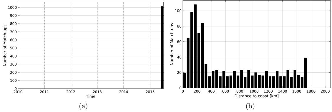
Figure 1: Number of match-ups between TSG-LEGOS-DM and SMAP-L3-RSS-V2-MONTHLY-0.25DEG-40KM SSS as a function of time (a) and as function of the distance to coast (b) over the Roaring Forties and Furious Fifties Pi-MEP region and for the full satellite product period.
