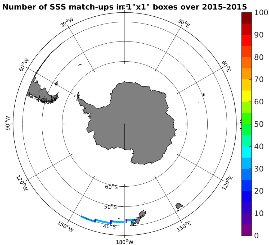
Figure 4: Number of SSS match-ups between TSG-LEGOS-DM SSS and the SMAP-L3-RSS-V2-MONTHLY-0.25DEG-40KM SSS product for the Roaring Forties and Furious Fifties Pi-MEP region over 1^\circ \times 1^\circ boxes and for the full satellite product period.
