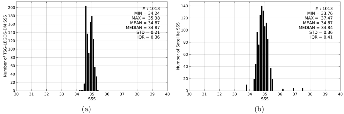
Figure 2: Histograms of SSS from TSG-LEGOS-DM (a) and SMAP-L3-RSS-V2-MONTHLY-0.25DEG-40KM (b) considering all match-up pairs per bins of 0.1 over the Roaring Forties and Furious Fifties Pi-MEP region and for the full satellite product period.
