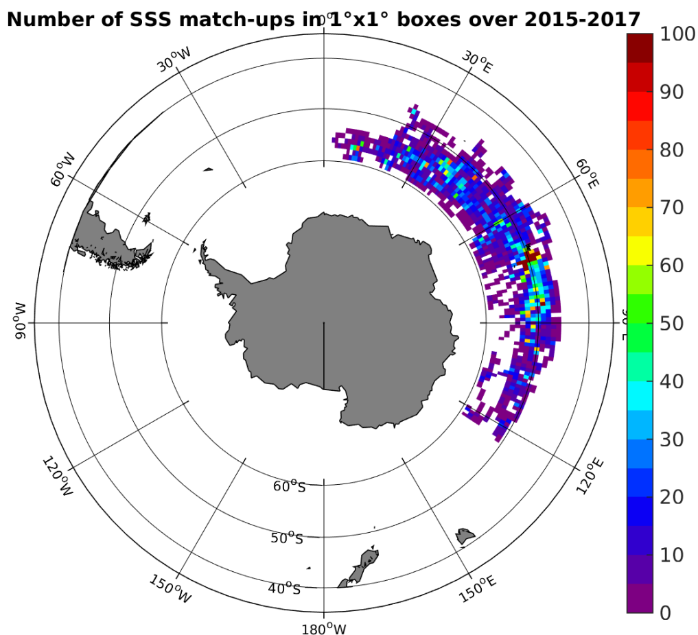
Figure 4: Number of SSS match-ups between Sea mammals SSS and the SMAP-L3-RSS-V2-MONTHLY-0.25DEG-40KM SSS product for the Roaring Forties and Furious Fifties Pi-MEP region over 1^\circ \times 1^\circ boxes and for the full satellite product period.
