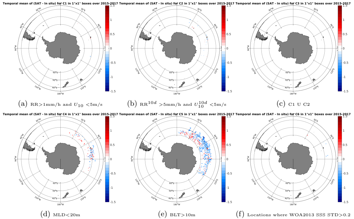
Figure 12: Temporal mean gridded over spatial boxes of size 1^\circ \times 1^\circ of \Delta SSS (SMAP-L3-RSS-V2-MONTHLY-0.25DEG-40KM - Sea mammals) for 6 different subdatasets corresponding to: RR > 1\text{mm/h} and U_{10} < 5\text{m/s} (a), RR^{10d} > 5\text{mm/h} and U_{10}^{10d} < 5\text{m/s} (b), C1 U C2 (c), MLD < 20\text{m} (d), BLT > 10\text{m} (e), Locations where WOA2013 SSS STD > 0.2 (f).
