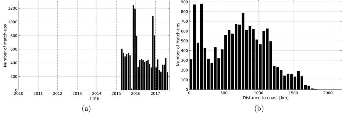
Figure 1: Number of match-ups between Sea mammals and SMAP-L3-RSS-V2-MONTHLY-0.25DEG-40KM SSS as a function of time (a) and as function of the distance to coast (b) over the Roaring Forties and Furious Fifties Pi-MEP region and for the full satellite product period.
