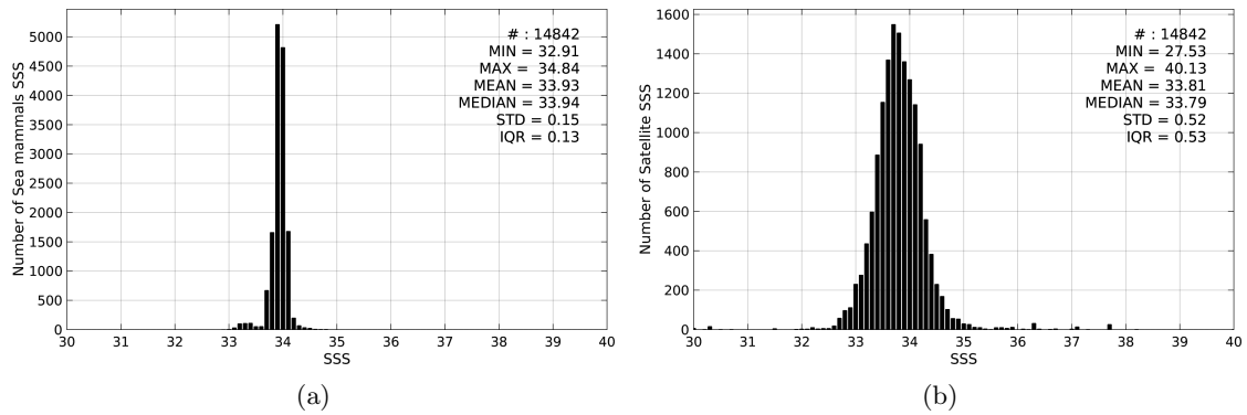
Figure 2: Histograms of SSS from Sea mammals (a) and SMAP-L3-RSS-V2-MONTHLY-0.25DEG-40KM (b) considering all match-up pairs per bins of 0.1 over the Roaring Forties and Furious Fifties Pi-MEP region and for the full satellite product period.
