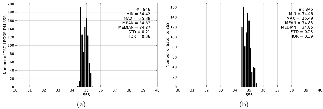
Figure 2: Histograms of SSS from TSG-LEGOS-DM (a) and SMAP-L3-RSS-V2-MONTHLY-70KM (b) considering all match-up pairs per bins of 0.1 over the Roaring Forties and Furious Fifties Pi-MEP region and for the full satellite product period.
