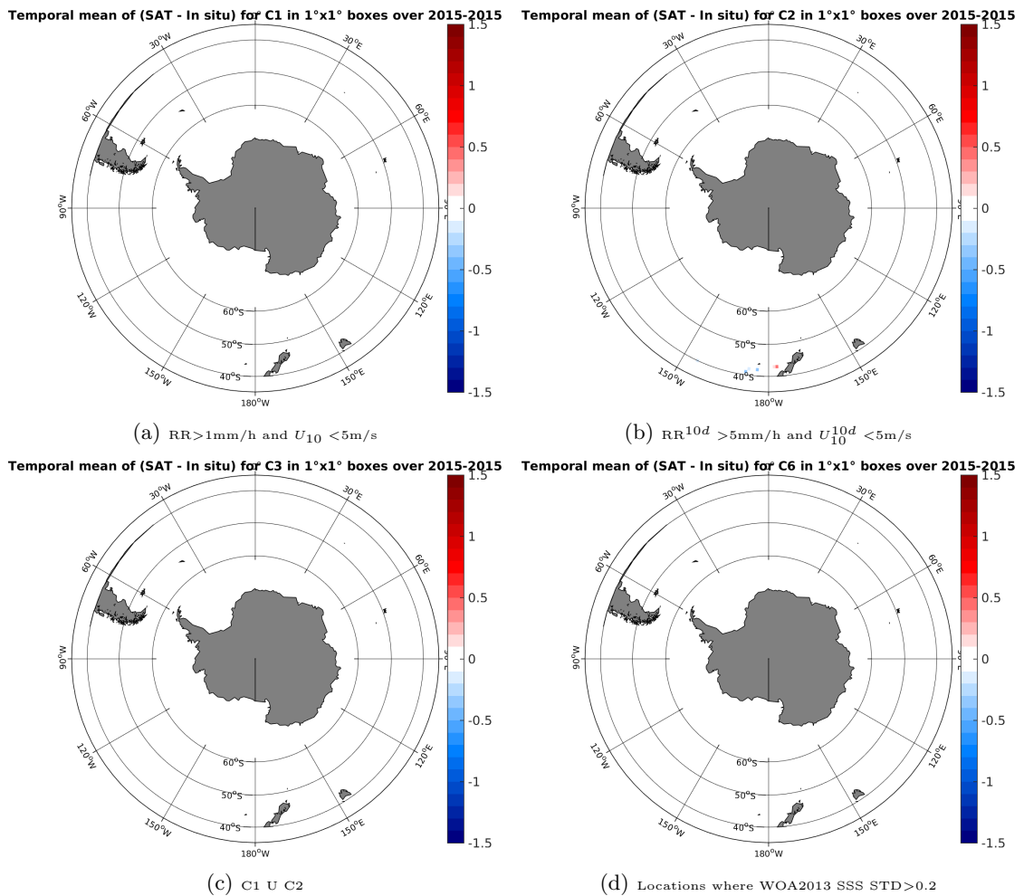
Figure 12: Temporal mean gridded over spatial boxes of size 1^\circ \times 1^\circ of \Delta SSS (SMAP-L3-RSS-V2-MONTHLY-70KM - TSG-LEGOS-DM) for 4 different subdatasets corresponding to:RR >1 mm/h and U_{10} < 5 m/s (a), RR^{10d} > 5 mm/h and U_{10}^{10d} < 5 m/s (b), C1 U C2 (c),Locations where WOA2013 SSS STD >0.2 (d).
