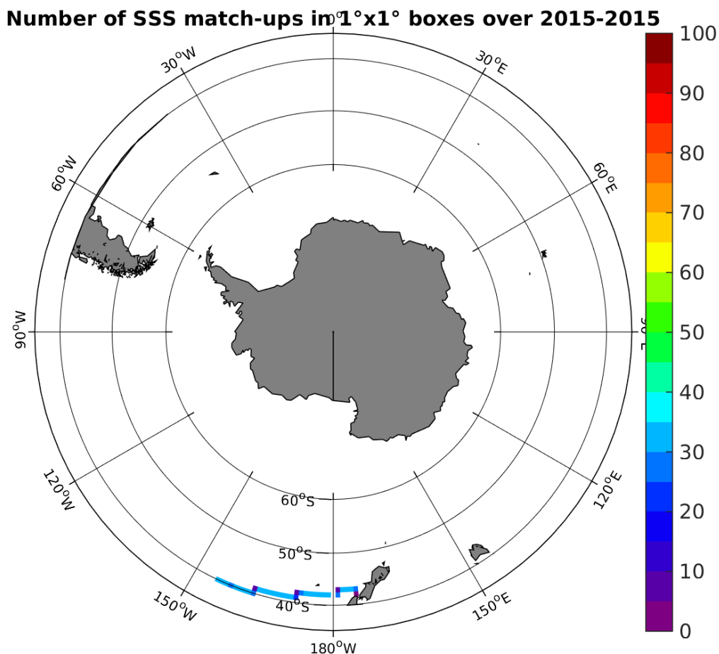
Figure 4: Number of SSS match-ups between TSG-LEGOS-DM SSS and the SMAP-L3-RSS-V2-MONTHLY-70KM SSS product for the Roaring Forties and Furious Fifties Pi-MEP region over 1°x1° boxes and for the full satellite product period.
