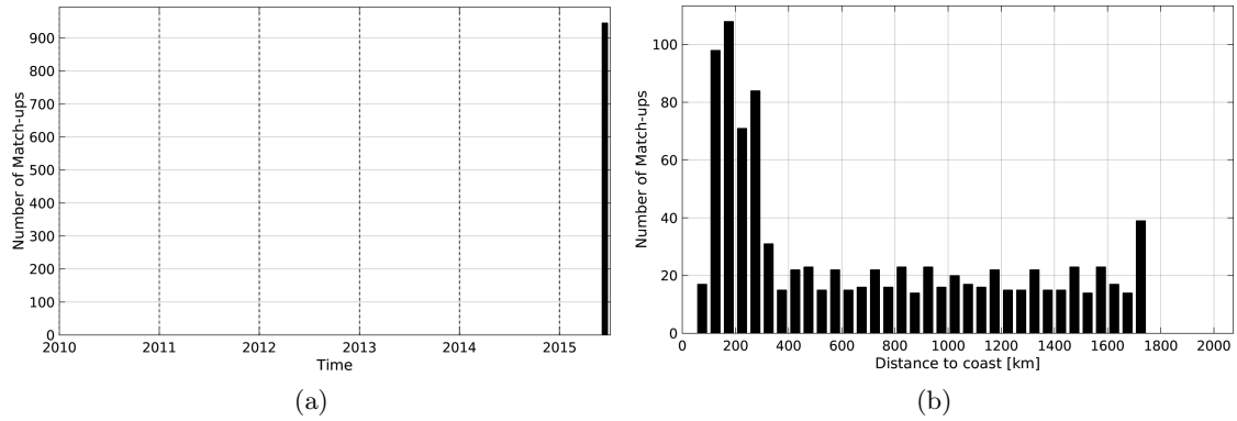
Figure 1: Number of match-ups between TSG-LEGOS-DM and SMAP-L3-RSS-V2-MONTHLY-70KM SSS as a function of time (a) and as function of the distance to coast (b) over the Roaring Forties and Furious Fifties Pi-MEP region and for the full satellite product period.
