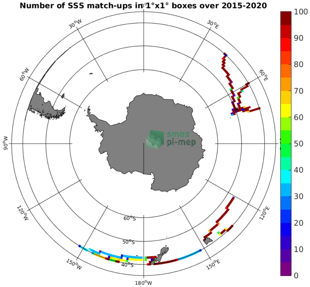
Figure 4: Number of SSS match-ups between TSG (LEGOS-DM) SSS and the SMAP SSS L3 v5.0 - 8-Day running (JPL) SSS product for the Roaring Forties and Furious Fifties Pi-MEP region over 1^\circ \times 1^\circ boxes and for the full satellite product period.
