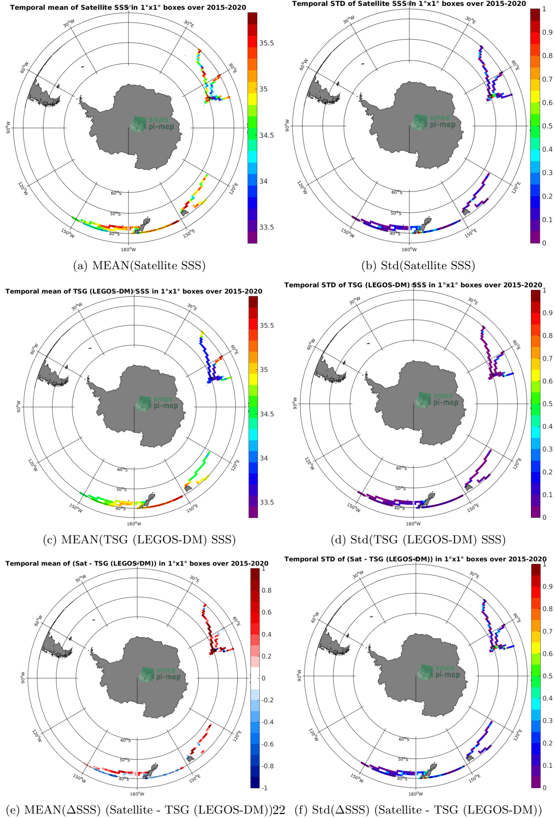
Figure 6: Temporal mean (left) and Std (right) of SSS from SMAP SSS L3 v5.0 - 8-Day running (JPL) (top), TSG (LEGOS-DM) (middle), and of \Delta SSS (Satellite - TSG (LEGOS-DM)). Only match-up pairs are used to generate these maps.
