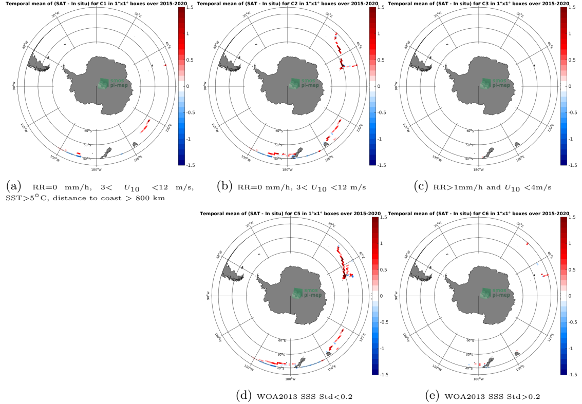
Figure 12: Temporal mean gridded over spatial boxes of size 1^{\circ} \times 1^{\circ} of \Delta\text{SSS} (SMAP SSS L3 v5.0 - 8-Day running (JPL) - TSG (LEGOS-DM)) for 5 different subdatasets corresponding to: \text{RR}=0 mm/h, 3 < U_{10} < 12 m/s, \text{SST} > 5^{\circ}\text{C} , distance to coast > 800 km (a), \text{RR}=0 mm/h, 3 < U_{10} < 12 m/s (b), \text{RR} > 1 mm/h and U_{10} < 4 m/s (c), WOA2013 SSS Std < 0.2 (d), WOA2013 SSS Std > 0.2 (e).
