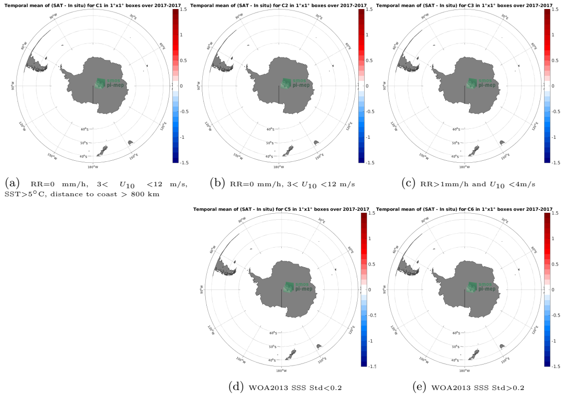
Figure 12: Temporal mean gridded over spatial boxes of size 1^\circ \times 1^\circ of \Delta\text{SSS} (SMAP SSS L3 v5.0 - 8-Day running (JPL) - TSG (GOSUD-Research-vessel)) for 5 different subdatasets corresponding to: RR=0 mm/h, 3 < U_{10} < 12 m/s, SST > 5^\circ\text{C} , distance to coast > 800 km (a), RR=0 mm/h, 3 < U_{10} < 12 m/s (b), RR > 1 mm/h and U_{10} < 4 m/s (c), WOA2013 SSS Std < 0.2 (d), WOA2013 SSS Std > 0.2 (e).
