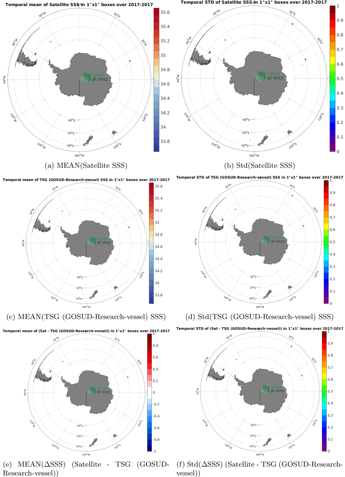
Figure 6: Temporal mean (left) and Std (right) of SSS from SMAP SSS L3 v5.0 - 8-Day running (JPL) (top), TSG (GOSUD-Research-vessel) (middle), and of \Delta SSS (Satellite - TSG (GOSUD-Research-vessel)). Only match-up pairs are used to generate these maps.
