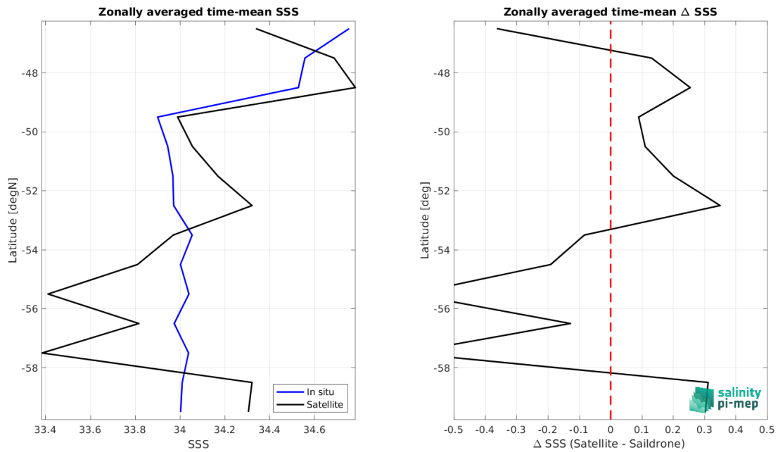
Figure 9: Left panel: Zonal mean SSS from SMAP SSS L3 v5.0 - 8-Day running (JPL) satellite product (black) and from Sailldrone (blue). Right panel: Zonal mean of \Delta SSS (Satellite - Sailldrone) for all the collected Pi-MEP match-up pairs estimated over the full satellite product period.
