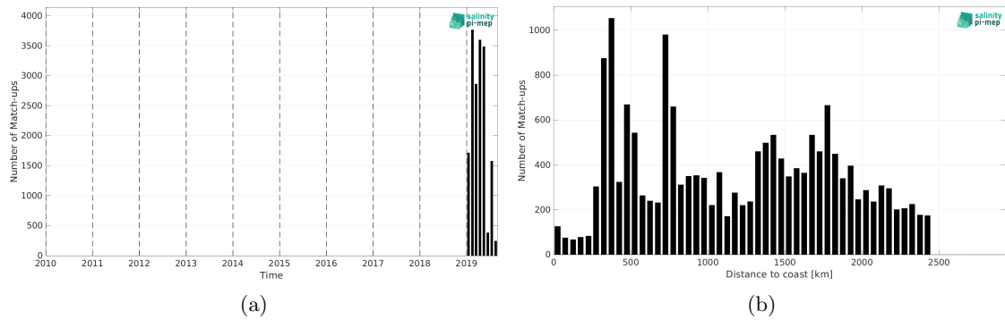
Figure 1: Number of match-ups between Saildrone and SMAP SSS L3 v5.0 - 8-Day running (JPL) SSS as a function of time (a) and as function of the distance to coast (b) over the Roaring Forties and Furious Fifties Pi-MEP region and for the full satellite product period.
