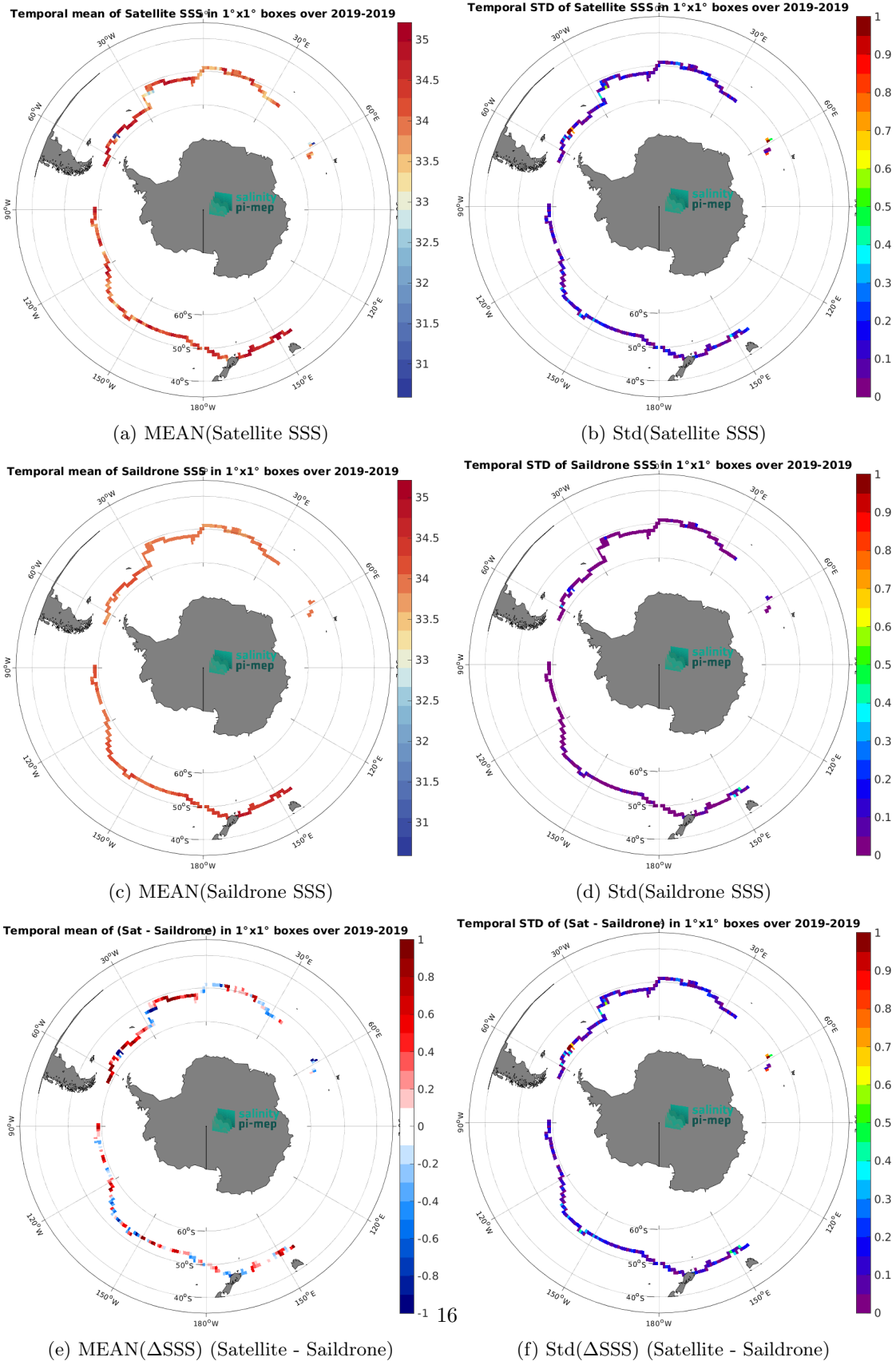
Figure 6: Temporal mean (left) and Std (right) of SSS from SMAP SSS L3 v5.0 - 8-Day running (JPL) (top), Saildrone (middle), and of \Delta SSS (Satellite - Saildrone). Only match-up pairs are used to generate these maps.
