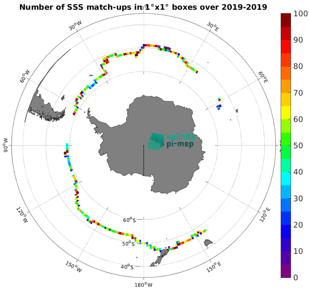
Figure 4: Number of SSS match-ups between Saildrone SSS and the SMAP SSS L3 v5.0 - 8-Day running (JPL) SSS product for the Roaring Forties and Furious Fifties Pi-MEP region over 1^\circ \times 1^\circ boxes and for the full satellite product period.
