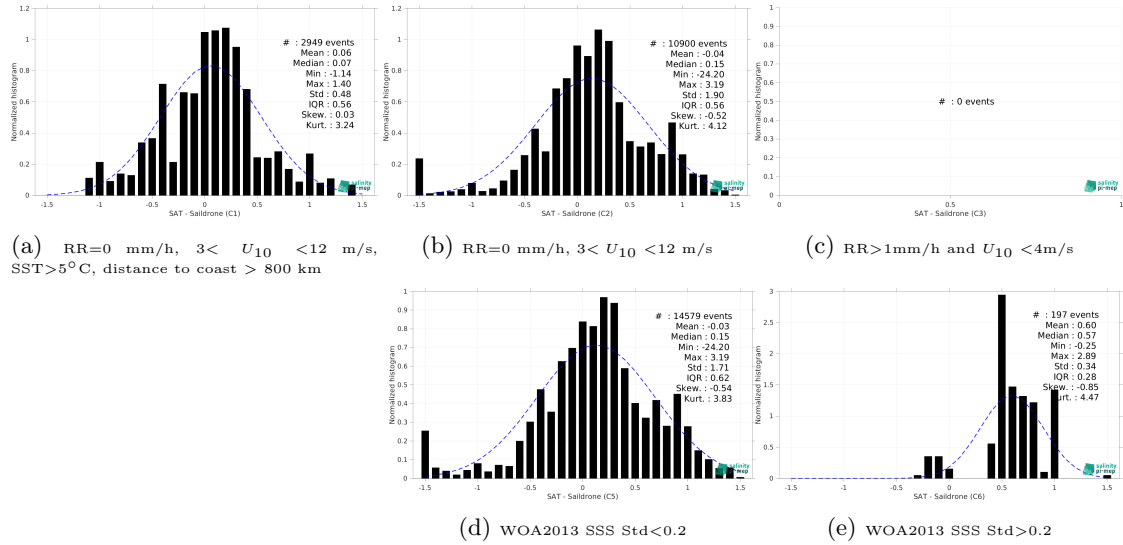
Figure 13: Normalized histogram of \Delta SSS (SMAP SSS L3 v5.0 - 8-Day running (JPL) - Saildrone) for 5 different subdatasets corresponding to: RR=0 mm/h, 3 < U_{10} < 12 m/s, SST > 5°C, distance to coast > 800 km (a), RR=0 mm/h, 3 < U_{10} < 12 m/s (b), RR > 1mm/h and U_{10} < 4 m/s (c), WOA2013 SSS Std < 0.2 (d), WOA2013 SSS Std > 0.2 (e).
