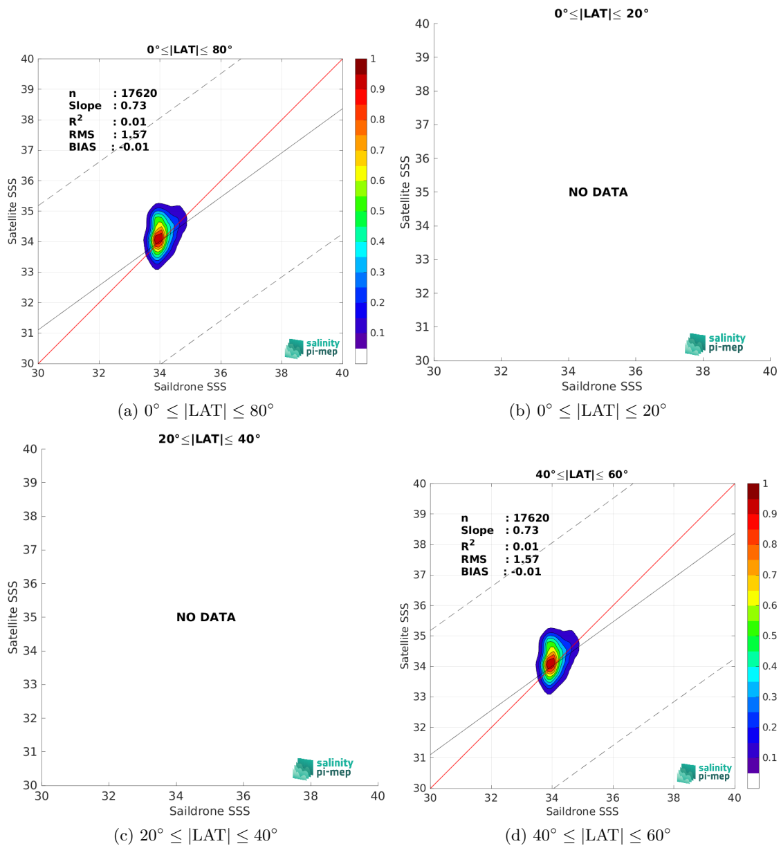
Figure 9: Contour maps of the concentration of SMAP SSS L3 v5.0 - 8-Day running (JPL) SSS (y-axis) versus Saildrone SSS (x-axis) at match-up pairs for different latitude bands. For each plot, the red line shows x=y . The black thin and dashed lines indicate a linear fit through the data cloud and the \pm 95\% confidence levels, respectively. The number match-up pairs n , the slope and R^2 coefficient of the linear fit, the root mean square (RMS) and the mean bias between satellite and in situ data are indicated for each latitude band in each plots.
