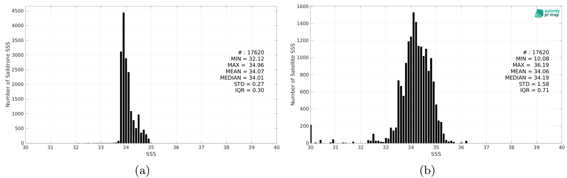
Figure 2: Histograms of SSS from Saildrone (a) and SMAP SSS L3 v5.0 - 8-Day running (JPL) (b) considering all match-up pairs per bins of 0.1 over the Roaring Forties and Furious Fifties Pi-MEP region and for the full satellite product period.
