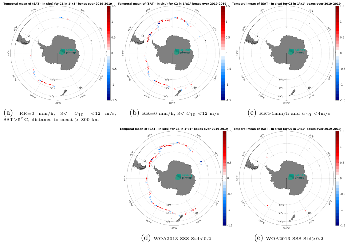
Figure 12: Temporal mean gridded over spatial boxes of size 1^{\circ}\times 1^{\circ} of \Delta\text{SSS} (SMAP SSS L3 v5.0 - 8-Day running (JPL) - Saildrone) for 5 different subdatasets corresponding to:RR=0 mm/h, 3 < U_{10} < 12 m/s, SST >5^{\circ}\text{C} , distance to coast > 800 km (a), RR=0 mm/h, 3 < U_{10} < 12 m/s (b), RR >1 mm/h and U_{10} < 4 m/s (c), WOA2013 SSS Std <0.2 (d), WOA2013 SSS Std >0.2 (e).
