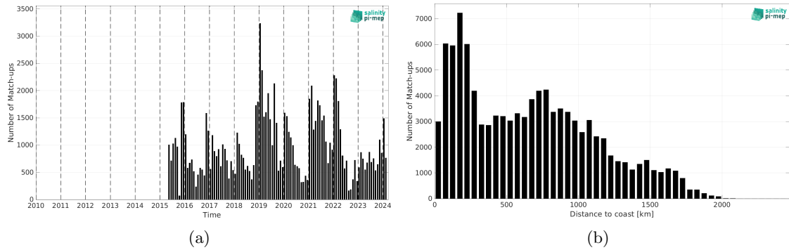
Figure 2: Number of match-ups between Marine mammals and SMAP SSS L3 v5.0 - 8-Day running (JPL) SSS as a function of time (a) and as function of the distance to coast (b) over the Roaring Forties and Furious Fifties Pi-MEP region and for the full satellite product period.
