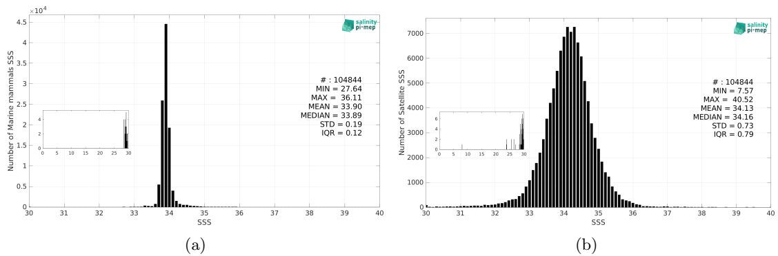
Figure 3: Histograms of SSS from Marine mammals (a) and SMAP SSS L3 v5.0 - 8-Day running (JPL) (b) considering all match-up pairs per bins of 0.1 over the Roaring Forties and Furious Fifties Pi-MEP region and for the full satellite product period.
