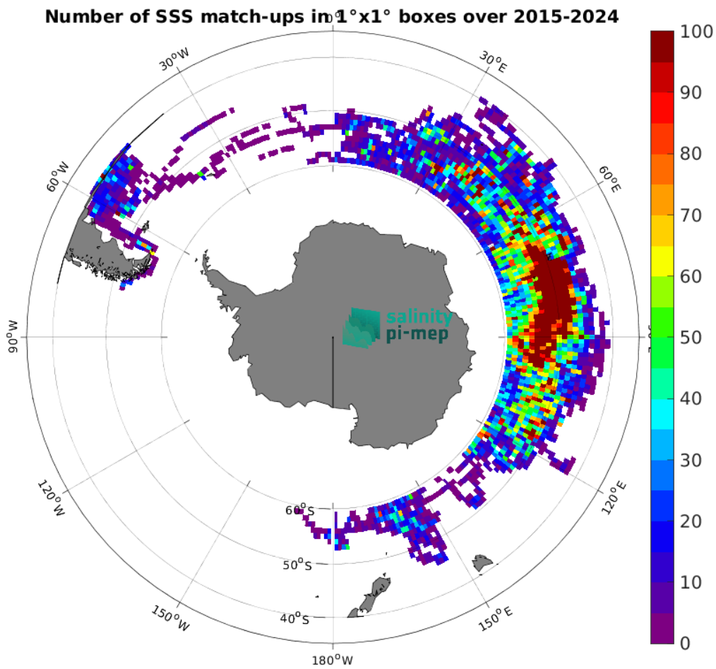
Figure 5: Number of SSS match-ups between Marine mammals SSS and the SMAP SSS L3 v5.0 - 8-Day running (JPL) SSS product for the Roaring Forties and Furious Fifties Pi-MEP region over 1^\circ \times 1^\circ boxes and for the full satellite product period.
