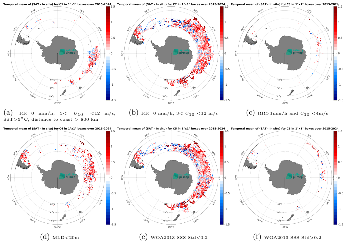
Figure 14: Temporal mean gridded over spatial boxes of size 1^\circ \times 1^\circ of \Delta SSS (SMAP SSS L3 v5.0 - 8-Day running (JPL) - Marine mammals) for 6 different subdatasets corresponding to:RR=0 mm/h, 3 < U_{10} < 12 m/s, SST>5°C, distance to coast > 800 km (a), RR=0 mm/h, 3 < U_{10} < 12 m/s (b), RR>1mm/h and U_{10} < 4 m/s (c),MLD<20m (d),WOA2013 SSS Std<0.2 (e),WOA2013 SSS Std>0.2 (f).
