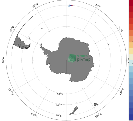
Temporal mean of Satellite SSS in 1°x1° boxes over 2020-2020
