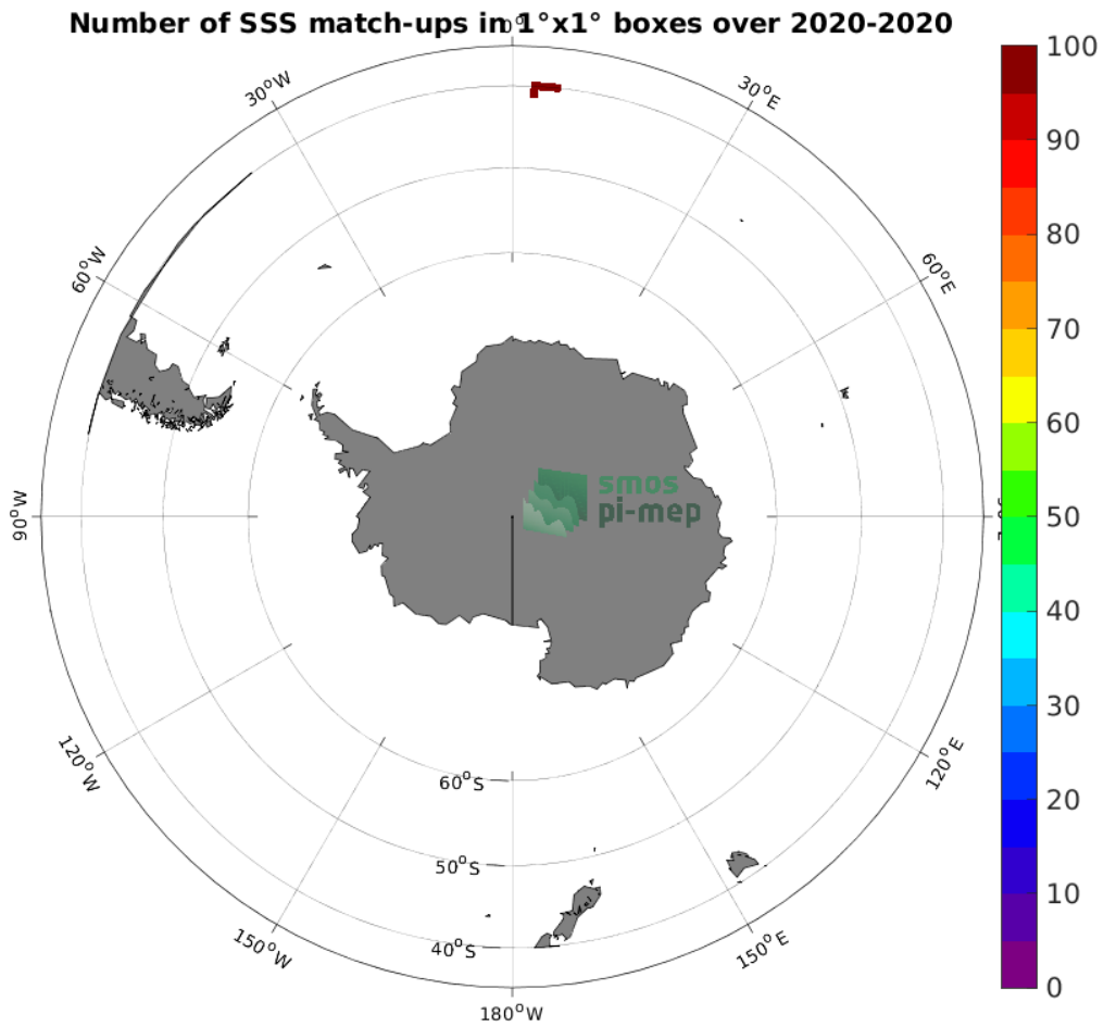
Figure 4: Number of SSS match-ups between TSG (SAMOS) SSS and the SMAP SSS L3 v5.0 - Monthly (JPL) SSS product for the Roaring Forties and Furious Fifties Pi-MEP region over 1^\circ \times 1^\circ boxes and for the full satellite product period.
