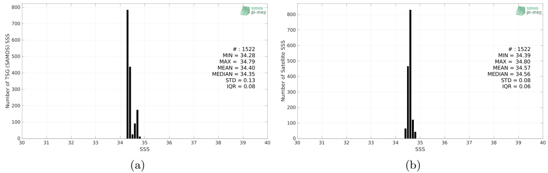
Figure 2: Histograms of SSS from TSG (SAMOS) (a) and SMAP SSS L3 v5.0 - Monthly (JPL) (b) considering all match-up pairs per bins of 0.1 over the Roaring Forties and Furious Fifties Pi-MEP region and for the full satellite product period.
