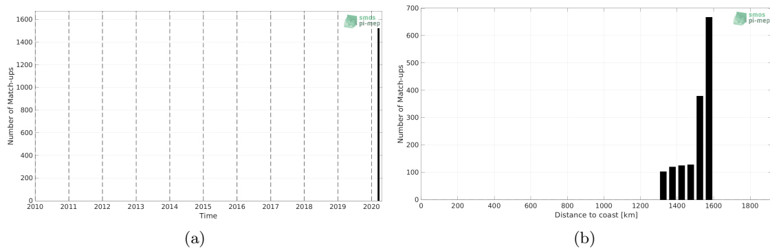
Figure 1: Number of match-ups between TSG (SAMOS) and SMAP SSS L3 v5.0 - Monthly (JPL) SSS as a function of time (a) and as function of the distance to coast (b) over the Roaring Forties and Furious Fifties Pi-MEP region and for the full satellite product period.
