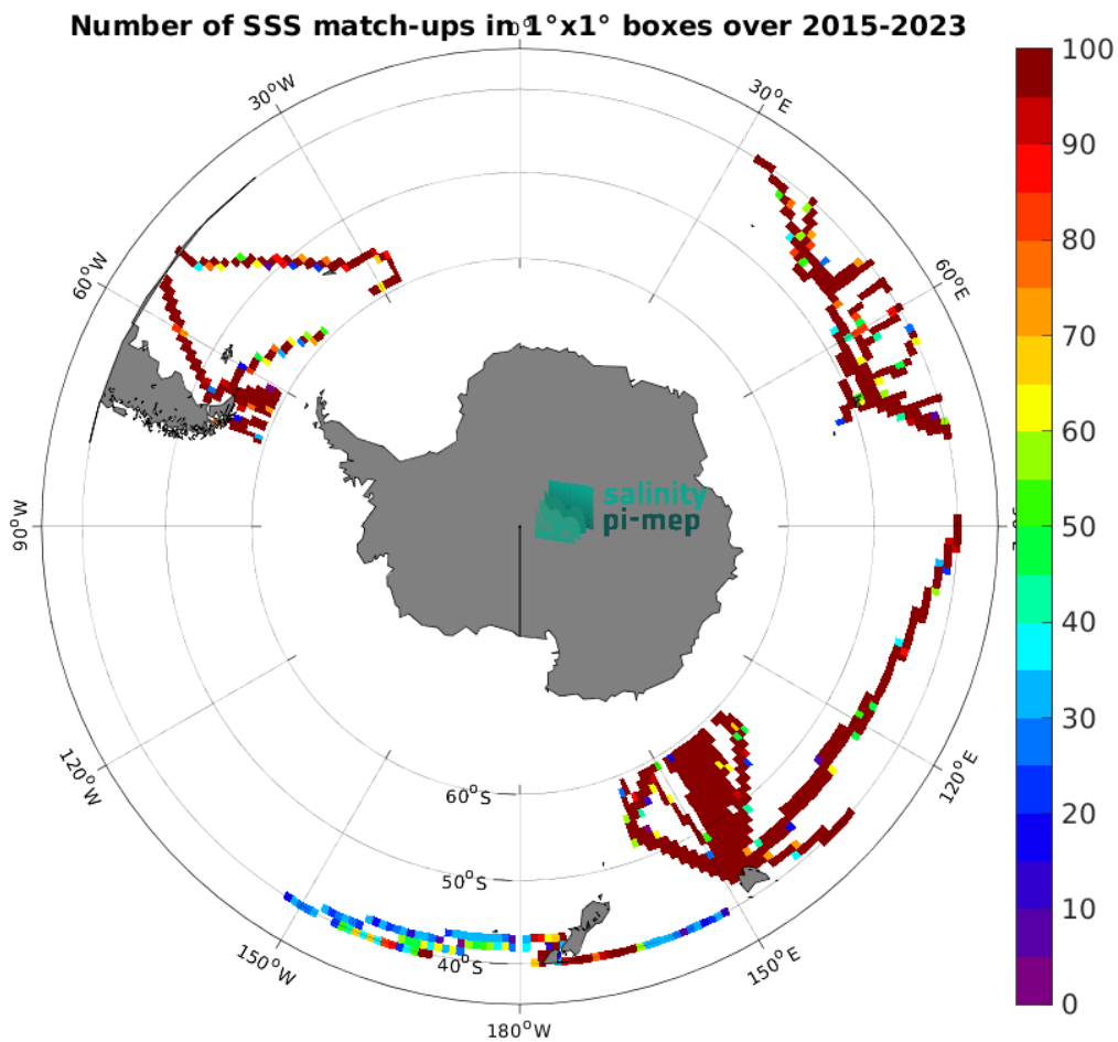
Figure 5: Number of SSS match-ups between TSG (LEGOS-DM) SSS and the SMAP SSS L3 v5.0 - Monthly (JPL) SSS product for the Roaring Forties and Furious Fifties Pi-MEP region over 1^\circ \times 1^\circ boxes and for the full satellite product period.
