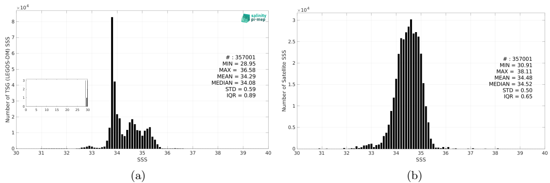
Figure 3: Histograms of SSS from TSG (LEGOS-DM) (a) and SMAP SSS L3 v5.0 - Monthly (JPL) (b) considering all match-up pairs per bins of 0.1 over the Roaring Forties and Furious Fifties Pi-MEP region and for the full satellite product period.
