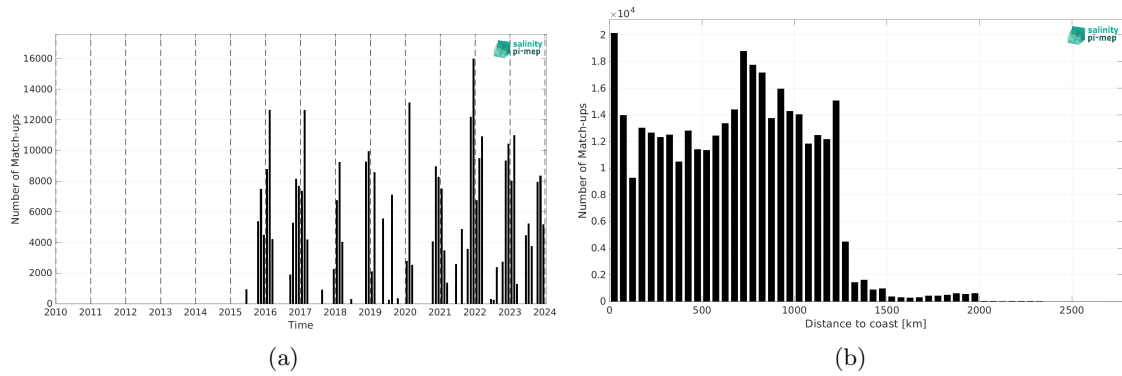
Figure 2: Number of match-ups between TSG (LEGOS-DM) and SMAP SSS L3 v5.0 - Monthly (JPL) SSS as a function of time (a) and as function of the distance to coast (b) over the Roaring Forties and Furious Fifties Pi-MEP region and for the full satellite product period.
