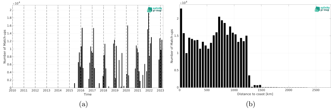
Figure 1: Number of match-ups between TSG (LEGOS-DM) and SMAP SSS L3 v5.0 - Monthly (JPL) SSS as a function of time (a) and as function of the distance to coast (b) over the Roaring Forties and Furious Fifties Pi-MEP region and for the full satellite product period.
