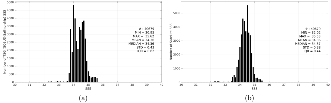
Figure 3: Histograms of SSS from TSG (GOSUD-Sailing-ship) (a) and SMAP SSS L3 v5.0 - Monthly (JPL) (b) considering all match-up pairs per bins of 0.1 over the Roaring Forties and Furious Fifties Pi-MEP region and for the full satellite product period.
