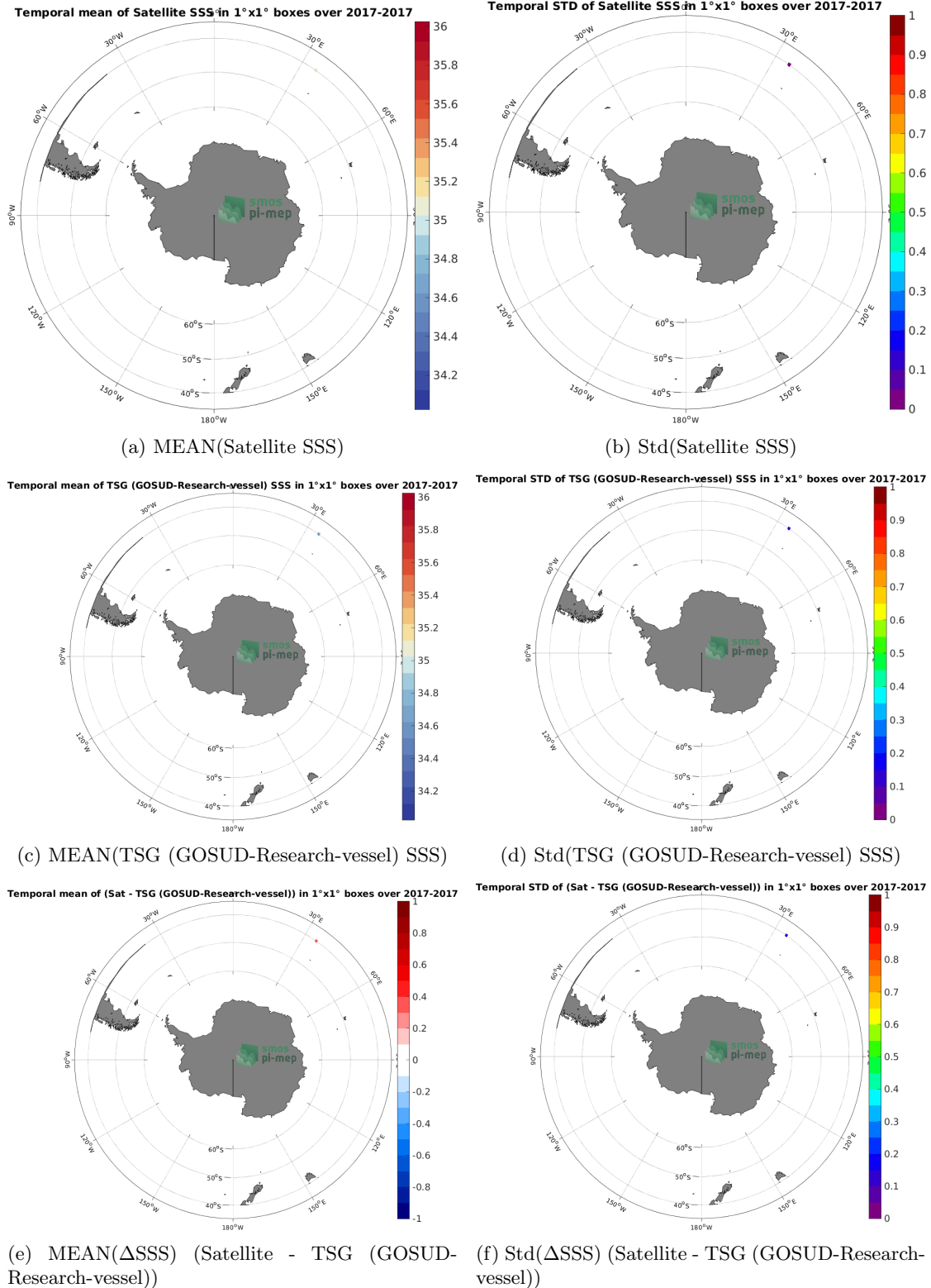
Figure 6: Temporal mean (left) and Std (right) of SSS from SMAP SSS L3 v5.0 - Monthly (JPL) (top), TSG (GOSUD-Research-vessel) (middle), and of \Delta SSS (Satellite - TSG (GOSUD-Research-vessel)). Only match-up pairs are used to generate these maps.
