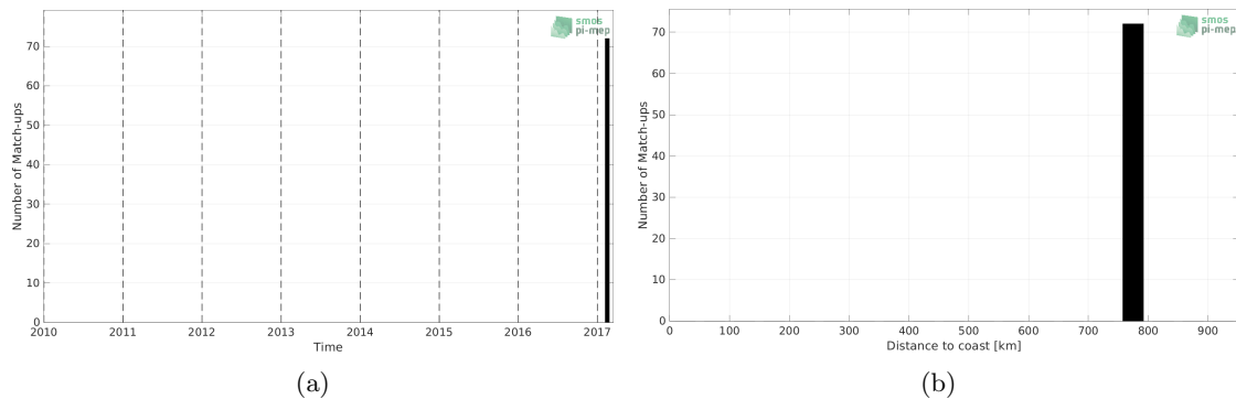
Figure 1: Number of match-ups between TSG (GOSUD-Research-vessel) and SMAP SSS L3 v5.0 - Monthly (JPL) SSS as a function of time (a) and as function of the distance to coast (b) over the Roaring Forties and Furious Fifties Pi-MEP region and for the full satellite product period.
