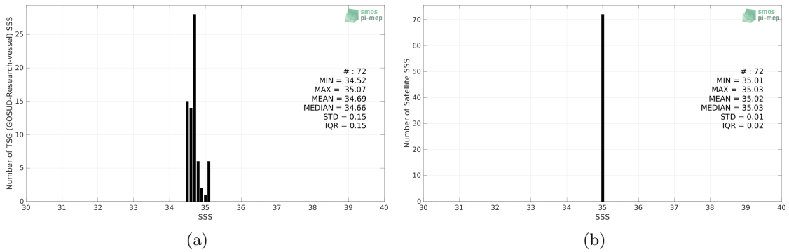
Figure 2: Histograms of SSS from TSG (GOSUD-Research-vessel) (a) and SMAP SSS L3 v5.0 - Monthly (JPL) (b) considering all match-up pairs per bins of 0.1 over the Roaring Forties and Furious Fifties Pi-MEP region and for the full satellite product period.
