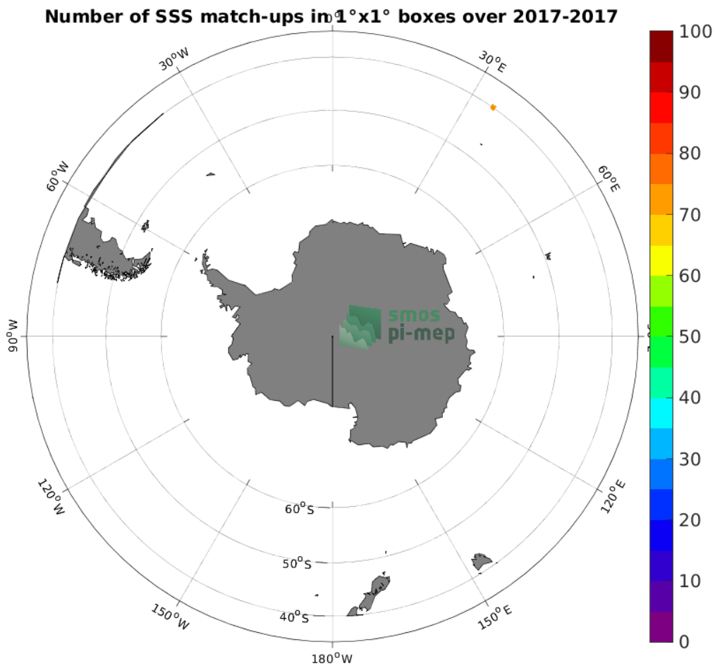
Figure 4: Number of SSS match-ups between TSG (GOSUD-Research-vessel) SSS and the SMAP SSS L3 v5.0 - Monthly (JPL) SSS product for the Roaring Forties and Furious Fifties Pi-MEP region over 1^\circ \times 1^\circ boxes and for the full satellite product period.
