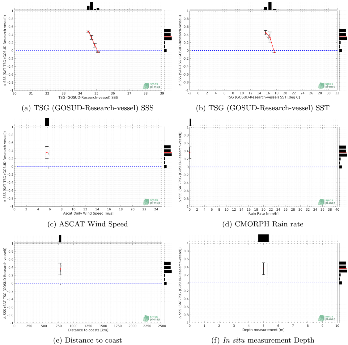
Figure 11: \Delta_{SSS} (Satellite - TSG (GOSUD-Research-vessel)) sorted as function of TSG (GOSUD-Research-vessel) SSS values a), TSG (GOSUD-Research-vessel) SST b), ASCAT Wind speed c), CMORPH rain rate d), distance to coast (e) and in situ measurement depth (f). In all plots the median and Std of \Delta_{SSS} for each bin is indicated by the red curves and black vertical thick bars ( \pm 1 Std)
