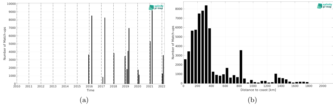
Figure 2: Number of match-ups between TSG (CSIC-UTM) and SMAP SSS L3 v5.0 - Monthly (JPL) SSS as a function of time (a) and as function of the distance to coast (b) over the Roaring Forties and Furious Fifties Pi-MEP region and for the full satellite product period.
