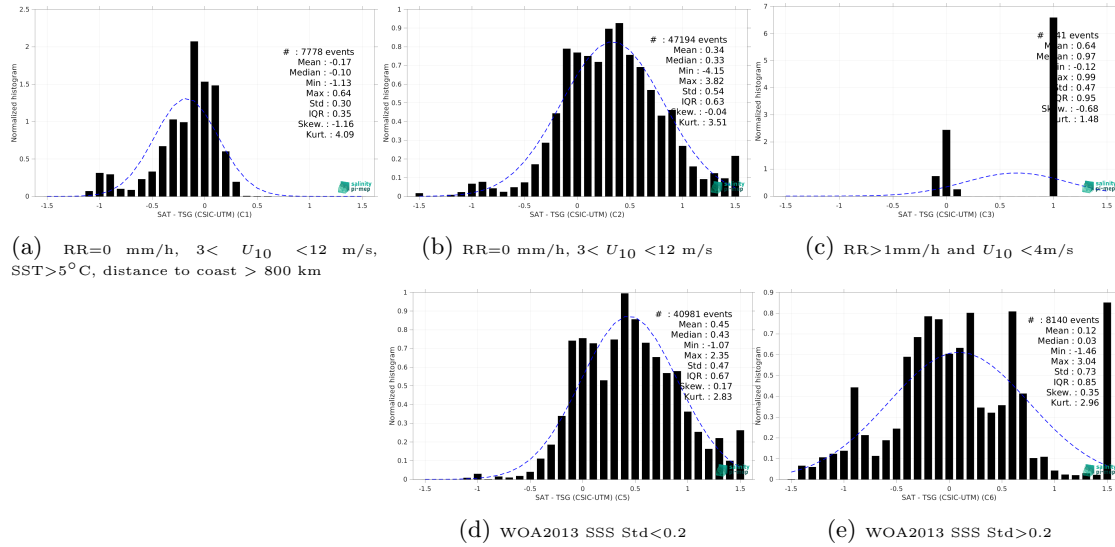
Figure 15: Normalized histogram of \Delta SSS (SMAP SSS L3 v5.0 - Monthly (JPL) - TSG (CSIC-UTM)) for 5 different subdatasets corresponding to: RR=0 mm/h, 3 < U_{10} < 12 m/s, SST > 5°C, distance to coast > 800 km (a), RR=0 mm/h, 3 < U_{10} < 12 m/s (b), RR > 1mm/h and U_{10} < 4 m/s (c), WOA2013 SSS Std < 0.2 (d), WOA2013 SSS Std > 0.2 (e).
