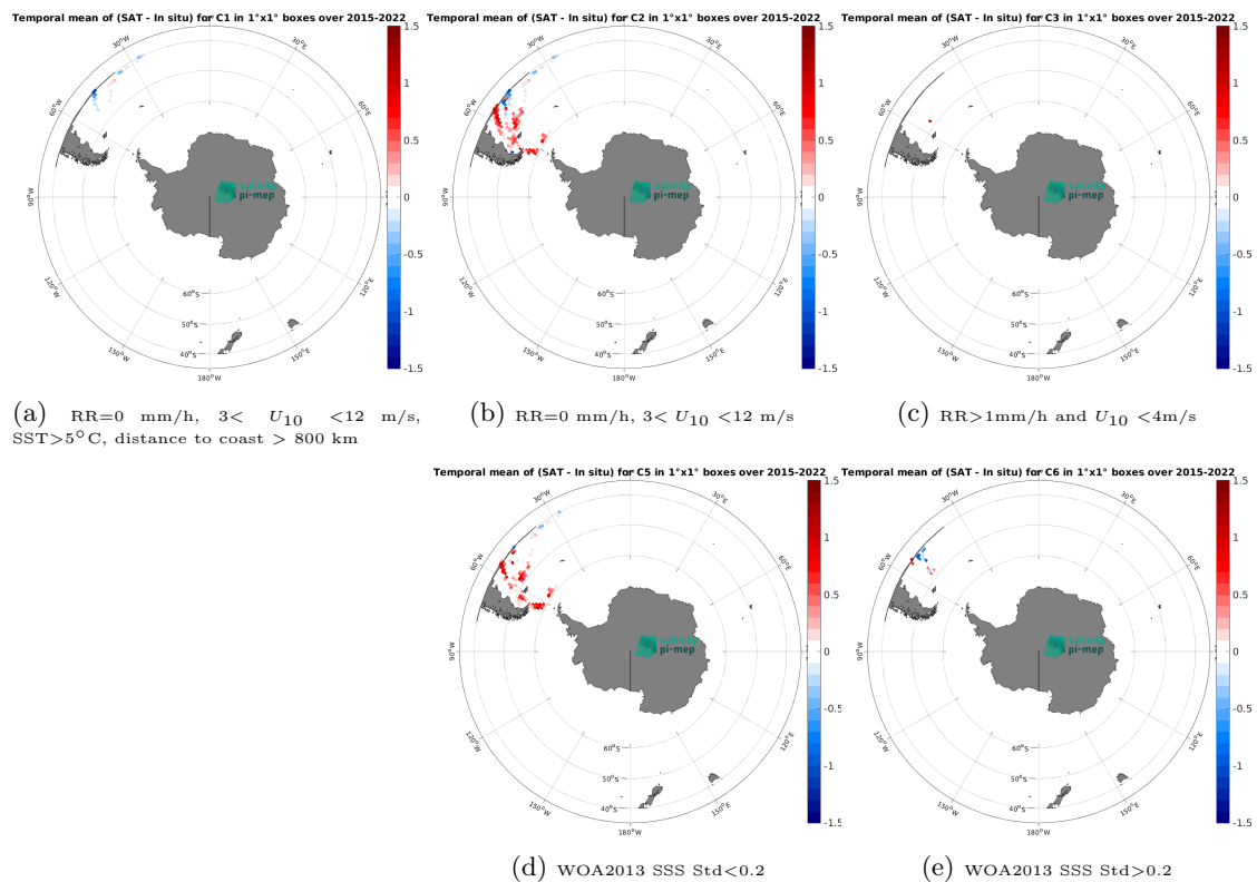
Figure 14: Temporal mean gridded over spatial boxes of size 1^\circ \times 1^\circ of \Delta\text{SSS} (SMAP SSS L3 v5.0 - Monthly (JPL) - TSG (CSIC-UTM)) for 5 different subdatasets corresponding to:RR=0 mm/h, 3 < U_{10} < 12 m/s, SST > 5°C, distance to coast > 800 km (a), RR=0 mm/h, 3 < U_{10} < 12 m/s (b), RR > 1mm/h and U_{10} < 4 m/s (c), WOA2013 SSS Std < 0.2 (d), WOA2013 SSS Std > 0.2 (e).
