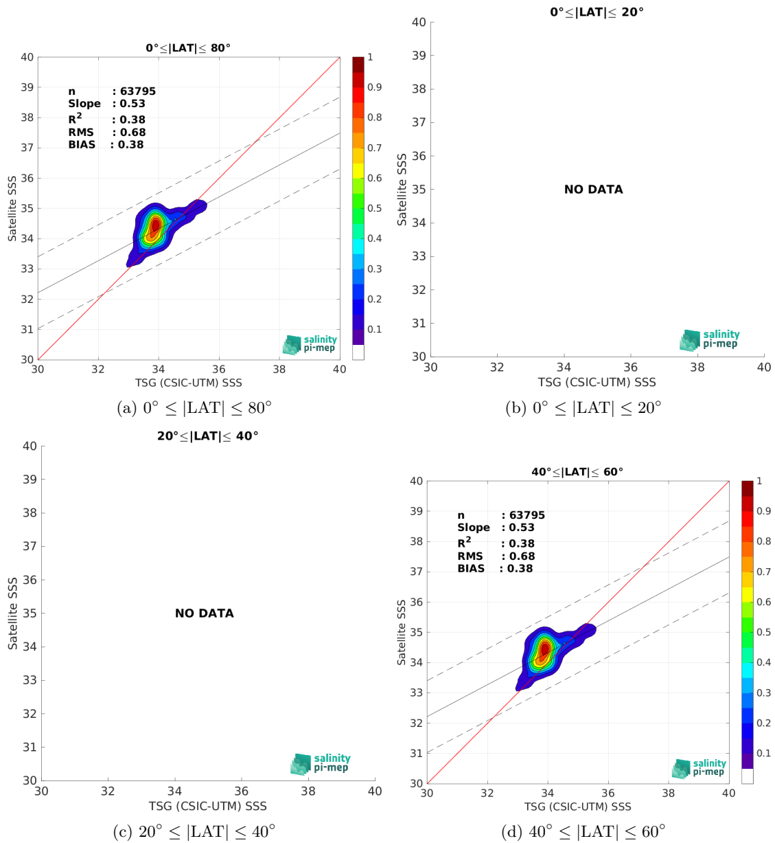
Figure 10: Contour maps of the concentration of SMAP SSS L3 v5.0 - Monthly (JPL) SSS (y-axis) versus TSG (CSIC-UTM) SSS (x-axis) at match-up pairs for different latitude bands. For each plot, the red line shows x=y . The black thin and dashed lines indicate a linear fit through the data cloud and the \pm 95\% confidence levels, respectively. The number match-up pairs n , the slope and R^2 coefficient of the linear fit, the root mean square (RMS) and the mean bias between satellite and in situ data are indicated for each latitude band in each plots.
