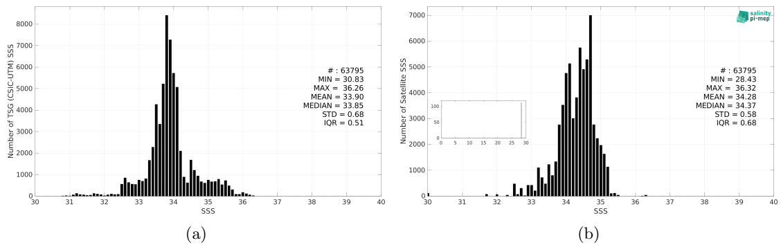
Figure 3: Histograms of SSS from TSG (CSIC-UTM) (a) and SMAP SSS L3 v5.0 - Monthly (JPL) (b) considering all match-up pairs per bins of 0.1 over the Roaring Forties and Furious Fifties Pi-MEP region and for the full satellite product period.
