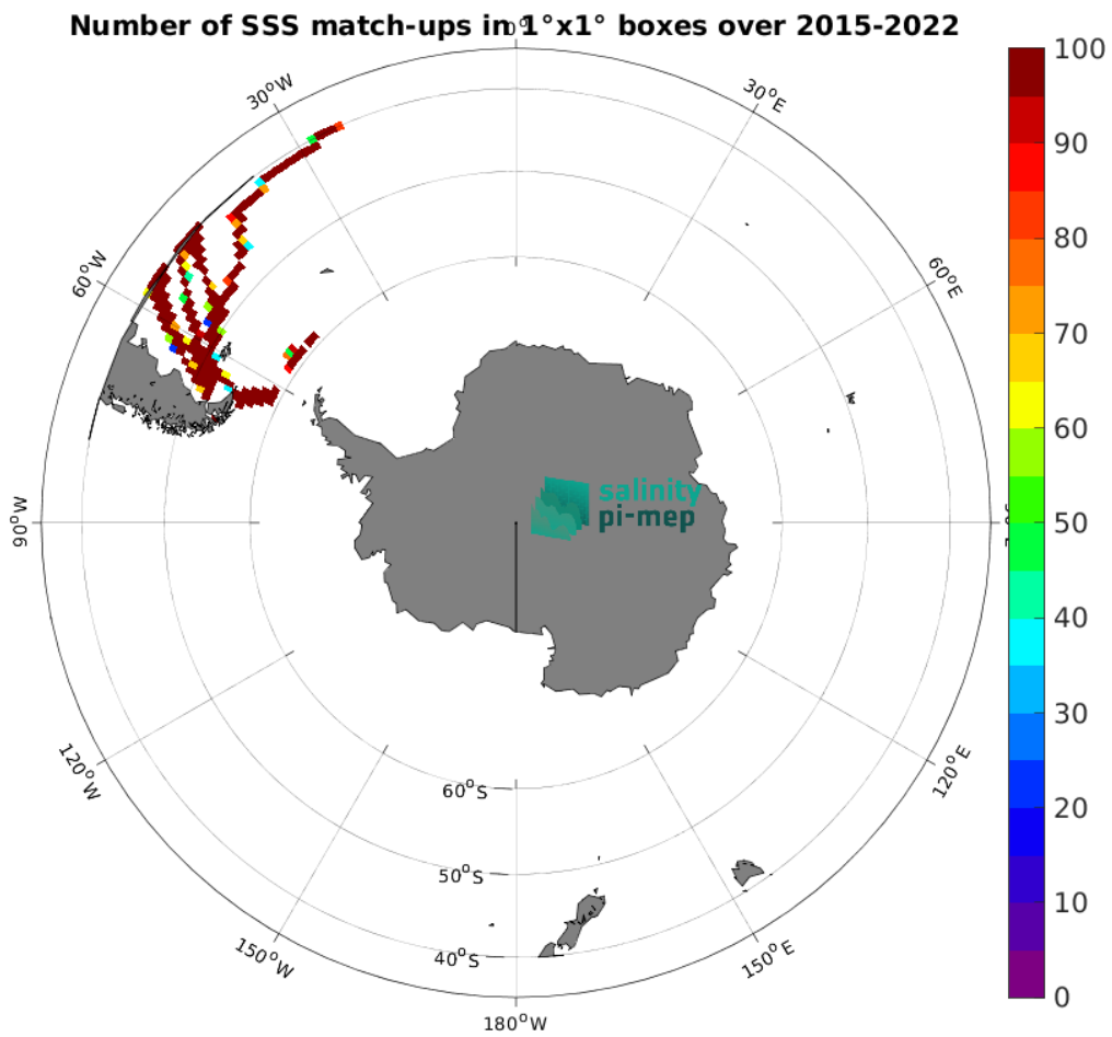
Figure 5: Number of SSS match-ups between TSG (CSIC-UTM) SSS and the SMAP SSS L3 v5.0 - Monthly (JPL) SSS product for the Roaring Forties and Furious Fifties Pi-MEP region over 1^\circ \times 1^\circ boxes and for the full satellite product period.
