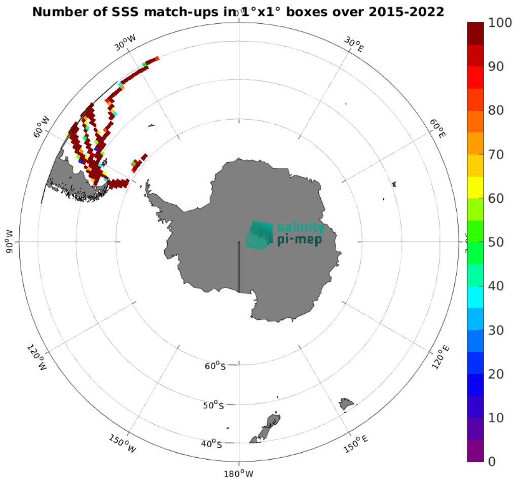
Figure 5: Number of SSS match-ups between TSG (CSIC-UTM) SSS and the SMAP SSS L3 v5.0 - Monthly (JPL) SSS product for the Roaring Forties and Furious Fifties Pi-MEP region over 1^{\circ} \times 1^{\circ} boxes and for the full satellite product period.
