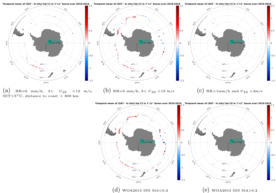
Figure 14: Temporal mean gridded over spatial boxes of size 1^\circ \times 1^\circ of \Delta\text{SSS} (SMAP SSS L3 v5.0 - Monthly (JPL) - Saildrone) for 5 different subdatasets corresponding to:RR=0 mm/h, 3 < U_{10} < 12 m/s, SST>5°C, distance to coast > 800 km (a), RR=0 mm/h, 3 < U_{10} < 12 m/s (b), RR>1mm/h and U_{10} < 4 m/s (c), WOA2013 SSS Std<0.2 (d), WOA2013 SSS Std>0.2 (e).
