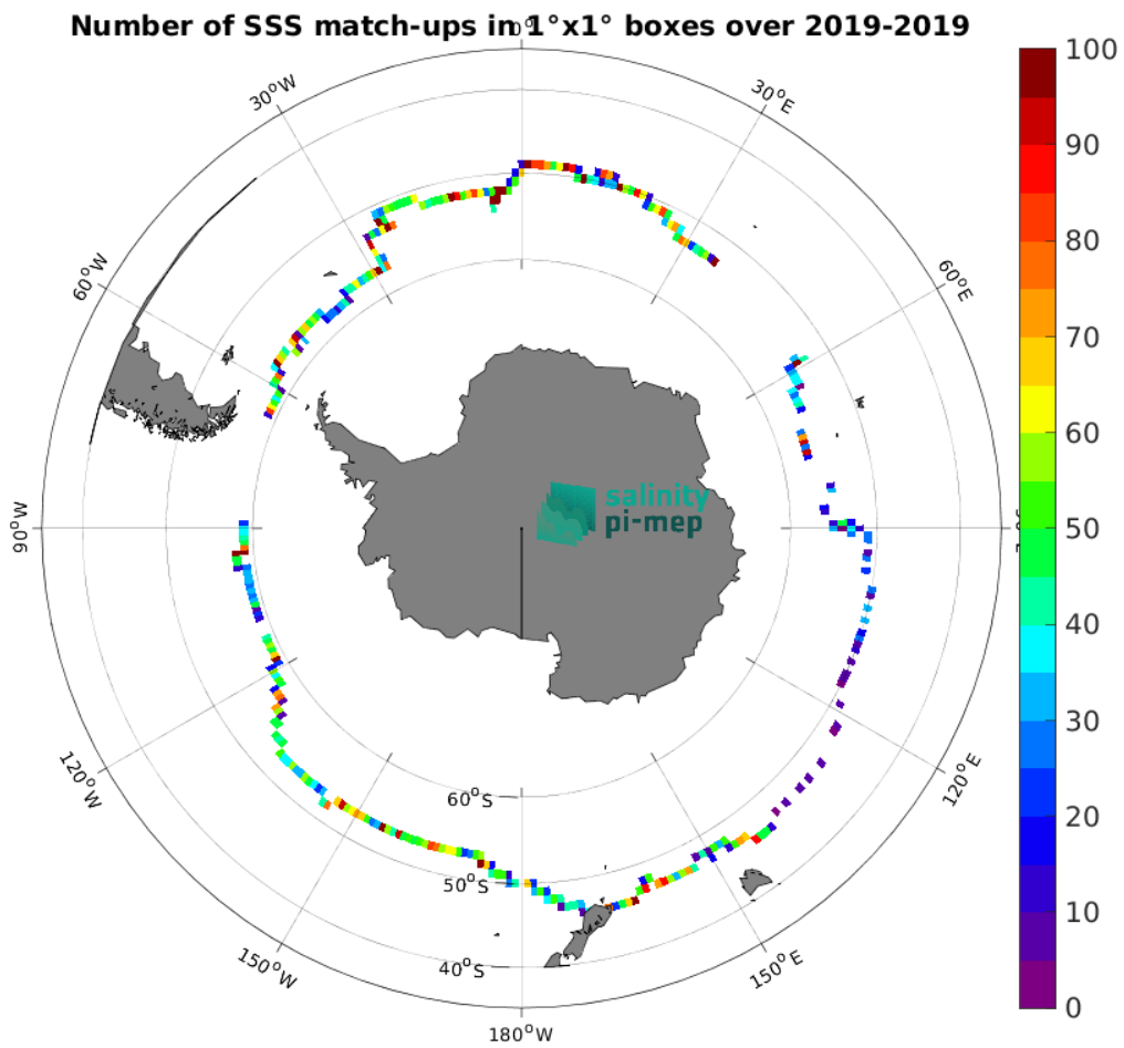
Figure 5: Number of SSS match-ups between Saildrone SSS and the SMAP SSS L3 v5.0 - Monthly (JPL) SSS product for the Roaring Forties and Furious Fifties Pi-MEP region over 1^\circ \times 1^\circ boxes and for the full satellite product period.
