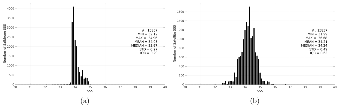
Figure 3: Histograms of SSS from Saildrone (a) and SMAP SSS L3 v5.0 - Monthly (JPL) (b) considering all match-up pairs per bins of 0.1 over the Roaring Forties and Furious Fifties Pi-MEP region and for the full satellite product period.
