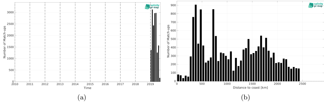
Figure 2: Number of match-ups between Saildrone and SMAP SSS L3 v5.0 - Monthly (JPL) SSS as a function of time (a) and as function of the distance to coast (b) over the Roaring Forties and Furious Fifties Pi-MEP region and for the full satellite product period.
