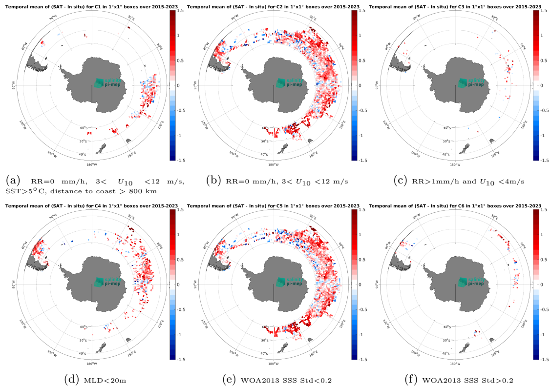
Figure 14: Temporal mean gridded over spatial boxes of size 1^\circ \times 1^\circ of \Delta\text{SSS} (SMAP SSS L3 v5.0 - Monthly (JPL) - Marine mammals) for 6 different subdatasets corresponding to:RR=0 mm/h, 3 < U_{10} < 12 m/s, SST>5°C, distance to coast > 800 km (a), RR=0 mm/h, 3 < U_{10} < 12 m/s (b), RR>1mm/h and U_{10} < 4 m/s (c),MLD<20m (d),WOA2013 SSS Std<0.2 (e),WOA2013 SSS Std>0.2 (f).
