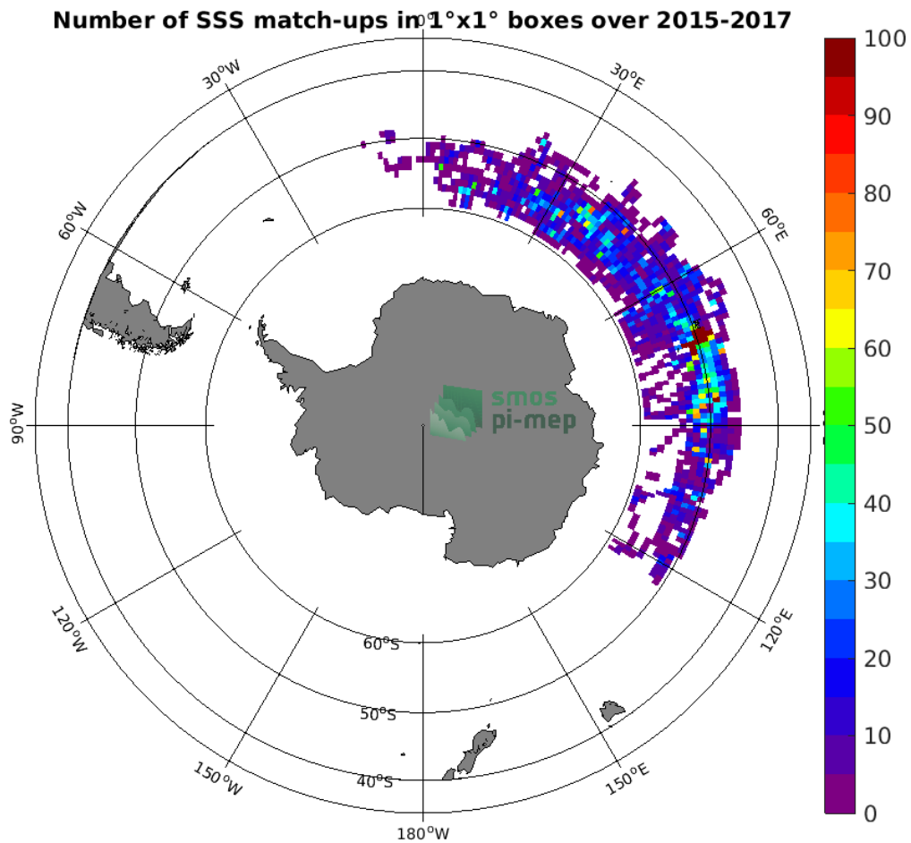
Figure 4: Number of SSS match-ups between Sea mammals SSS and the SMAP SSS L3 v5.0 - Monthly (JPL) SSS product for the Roaring Forties and Furious Fifties Pi-MEP region over 1^\circ \times 1^\circ boxes and for the full satellite product period.
