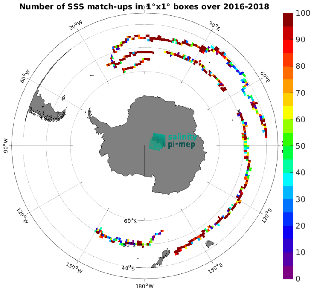
Figure 4: Number of SSS match-ups between Surface drifters SSS and the SMAP SSS L3 v5.0 - Monthly (JPL) SSS product for the Roaring Forties and Furious Fifties Pi-MEP region over 1^\circ \times 1^\circ boxes and for the full satellite product period.
