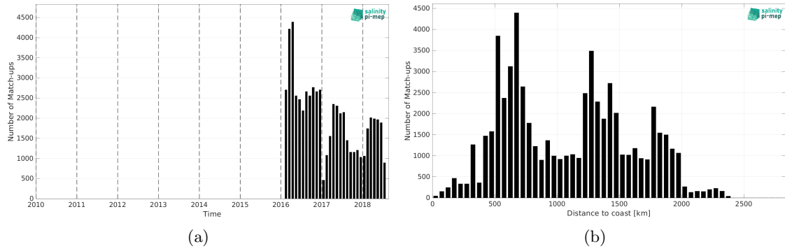
Figure 2: Number of match-ups between Surface drifters and SMAP SSS L3 v5.0 - Monthly (JPL) SSS as a function of time (a) and as function of the distance to coast (b) over the Roaring Forties and Furious Fifties Pi-MEP region and for the full satellite product period.
