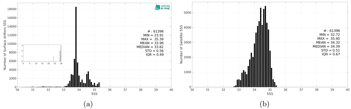
Figure 3: Histograms of SSS from Surface drifters (a) and SMAP SSS L3 v5.0 - Monthly (JPL) (b) considering all match-up pairs per bins of 0.1 over the Roaring Forties and Furious Fifties Pi-MEP region and for the full satellite product period.
