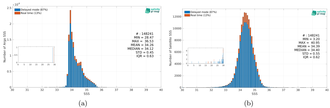
Figure 3: Histograms of SSS from Argo (a) and SMAP SSS L3 v5.0 - Monthly (JPL) (b) considering all match-up pairs per bins of 0.1 over the Roaring Forties and Furious Fifties Pi-MEP region and for the full satellite product period.
