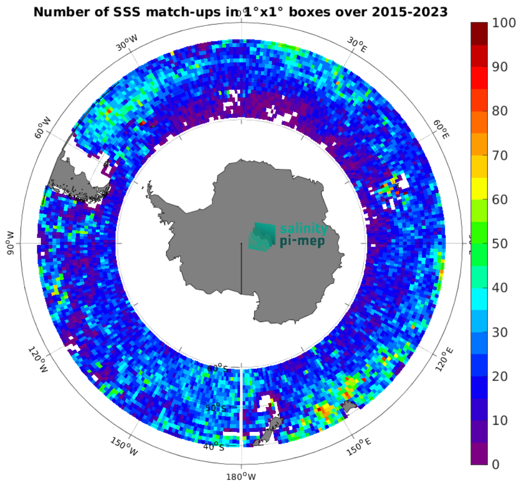
Figure 5: Number of SSS match-ups between Argo SSS and the SMAP SSS L3 v5.0 - Monthly (JPL) SSS product for the Roaring Forties and Furious Fifties Pi-MEP region over 1^\circ \times 1^\circ boxes and for the full satellite product period.
