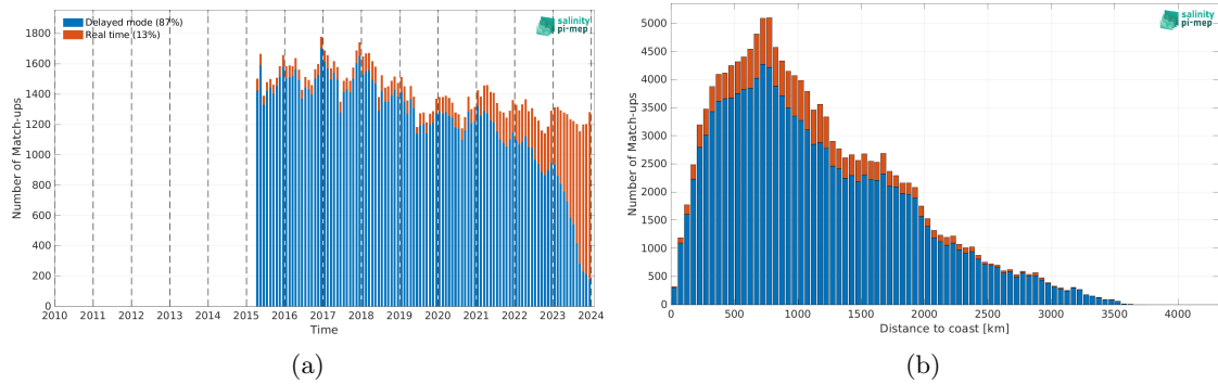
Figure 2: Number of match-ups between Argo and SMAP SSS L3 v5.0 - Monthly (JPL) SSS as a function of time (a) and as function of the distance to coast (b) over the Roaring Forties and Furious Fifties Pi-MEP region and for the full satellite product period.
