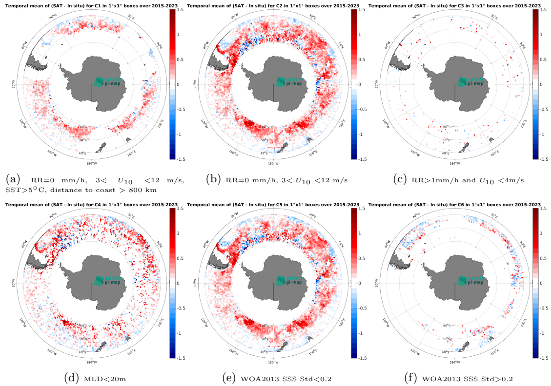
Figure 14: Temporal mean gridded over spatial boxes of size 1^\circ \times 1^\circ of \Delta SSS (SMAP SSS L3 v5.0 - Monthly (JPL) - Argo) for 6 different subdatasets corresponding to:RR=0 mm/h, 3 < U_{10} < 12 m/s, SST >5^\circ C, distance to coast > 800 km (a), RR=0 mm/h, 3 < U_{10} < 12 m/s (b), RR >1 mm/h and U_{10} < 4 m/s (c),MLD <20 m (d),WOA2013 SSS Std <0.2 (e),WOA2013 SSS Std >0.2 (f).
