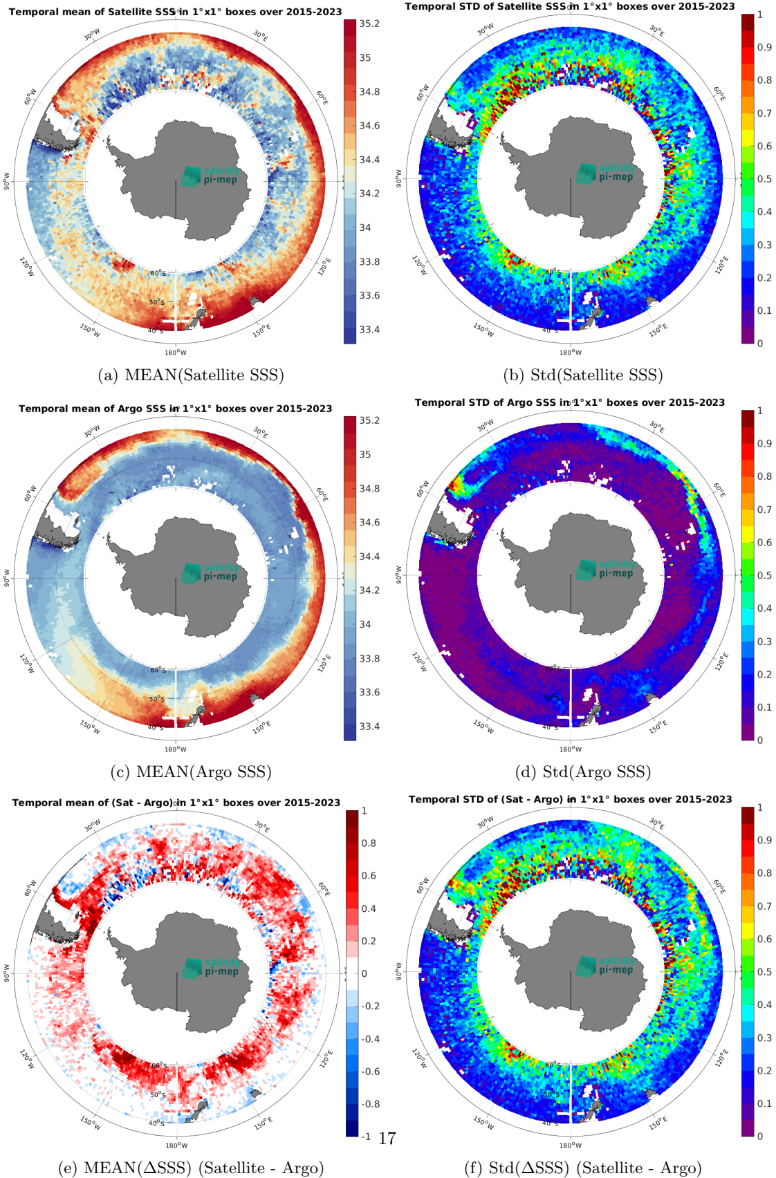
Figure 7: Temporal mean (left) and Std (right) of SSS from SMAP SSS L3 v5.0 - Monthly (JPL) (top), Argo (middle), and of \Delta SSS (Satellite - Argo). Only match-up pairs are used to generate these maps.
