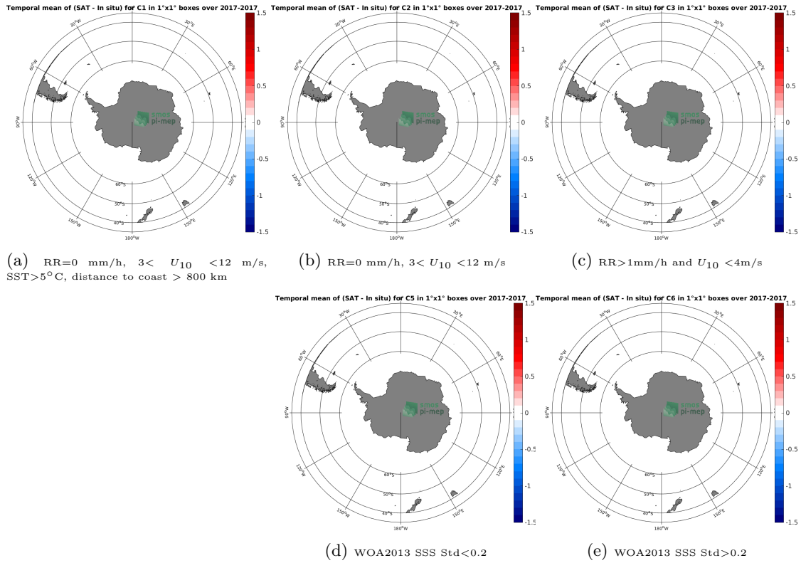
Figure 12: Temporal mean gridded over spatial boxes of size 1°x1° of \Delta SSS (SMAP-L3-JPL-V4.3-8DAY-RUNNING-60KM - TSG-GOSUD-Research-vessel) for 5 different subdatasets corresponding to:RR=0 mm/h, 3 < U_{10} < 12 m/s, SST>5°C, distance to coast > 800 km (a), RR=0 mm/h, 3 < U_{10} < 12 m/s (b), RR>1mm/h and U_{10} < 4 m/s (c), WOA2013 SSS Std<0.2 (d), WOA2013 SSS Std>0.2 (e).
