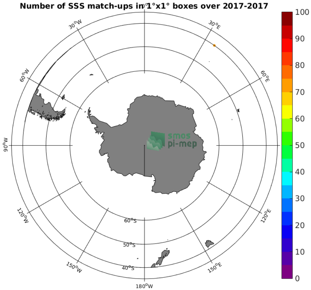
Figure 4: Number of SSS match-ups between TSG-GOSUD-Research-vessel SSS and the SMAP-L3-JPL-V4.3-MONTHLY-60KM SSS product for the Roaring Forties and Furious Fifties Pi-MEP region over 1°x1° boxes and for the full satellite product period.
