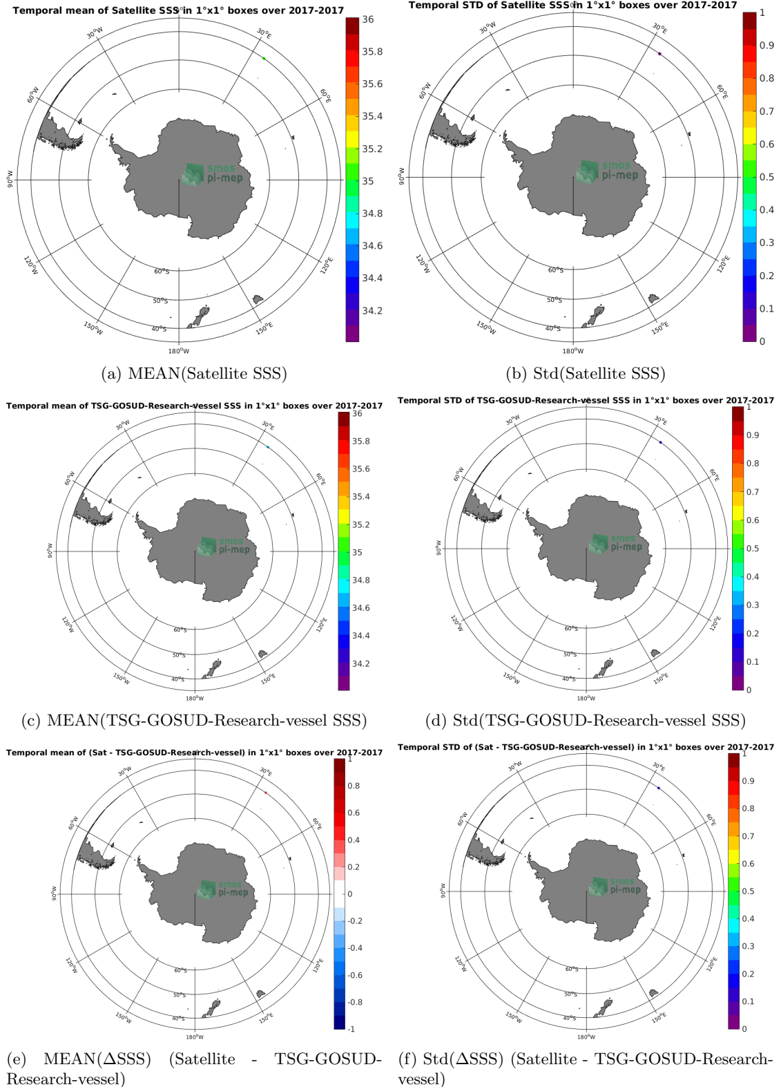
Figure 6: Temporal mean (left) and Std (right) of SSS from SMAP-L3-JPL-V4.3-MONTHLY-60KM (top), TSG-GOSUD-Research-vessel (middle), and of \Delta SSS (Satellite - TSG-GOSUD-Research-vessel). Only match-up pairs are used to generate these maps.
