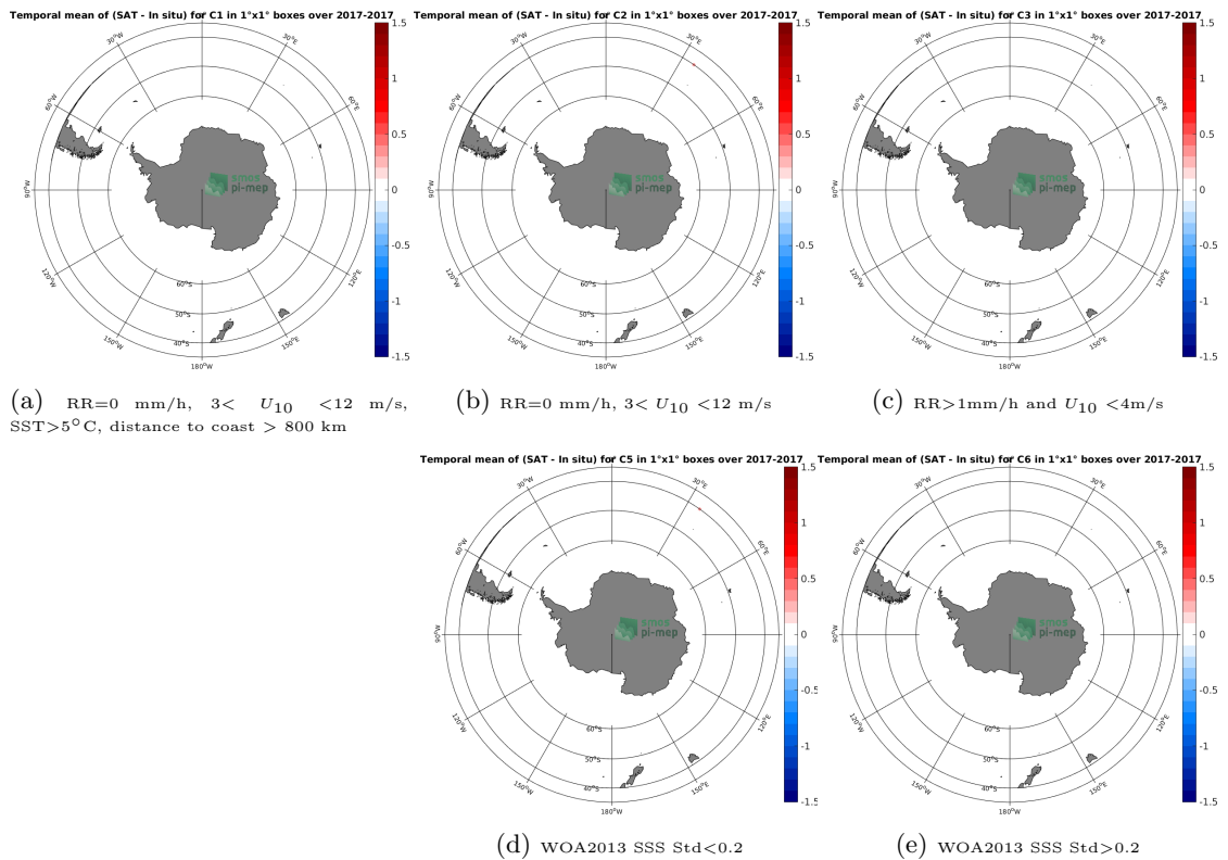
Figure 12: Temporal mean gridded over spatial boxes of size 1^\circ \times 1^\circ of \Delta SSS (SMAP-L3-JPL-V4.3-MONTHLY-60KM - TSG-GOSUD-Research-vessel) for 5 different subdatasets corresponding to:RR=0 mm/h, 3 < U_{10} < 12 m/s, SST>5°C, distance to coast > 800 km (a), RR=0 mm/h, 3 < U_{10} < 12 m/s (b), RR>1mm/h and U_{10} < 4 m/s (c), WOA2013 SSS Std<0.2 (d), WOA2013 SSS Std>0.2 (e).
