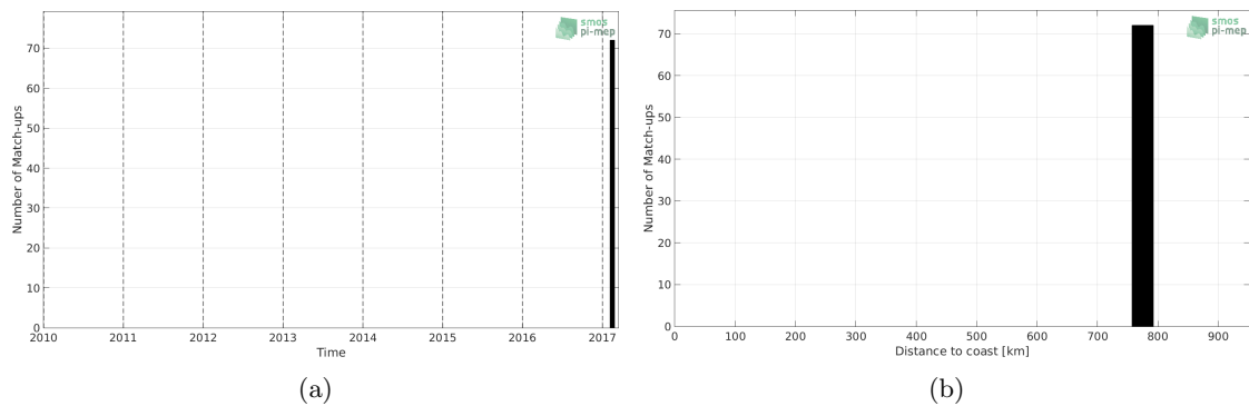
Figure 1: Number of match-ups between TSG-GOSUD-Research-vessel and SMAP-L3-JPL-V4.3-MONTHLY-60KM SSS as a function of time (a) and as function of the distance to coast (b) over the Roaring Forties and Furious Fifties Pi-MEP region and for the full satellite product period.
