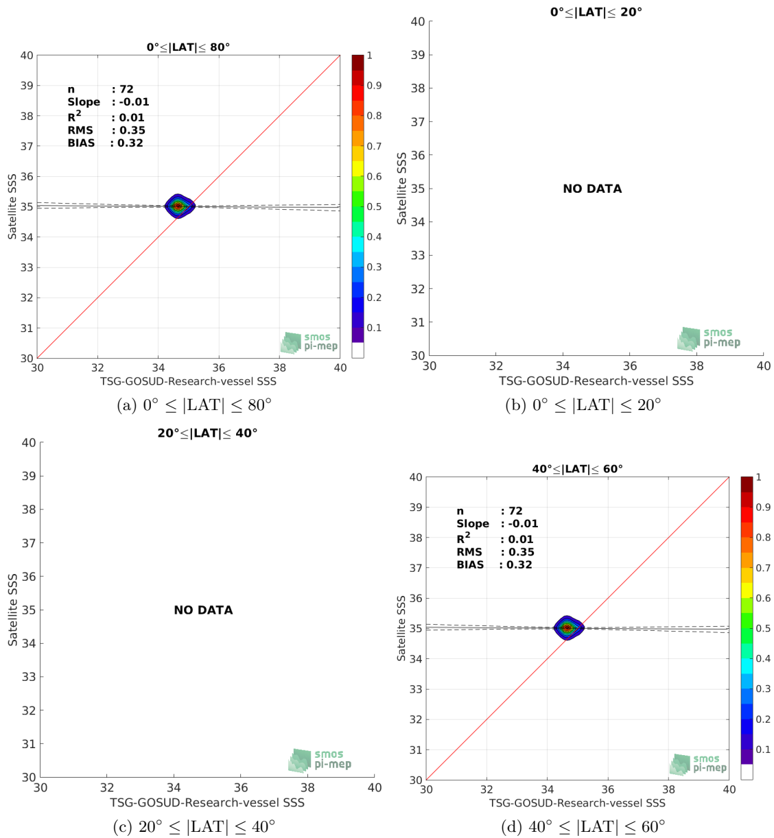
Figure 9: Contour maps of the concentration of SMAP-L3-JPL-V4.3-MONTHLY-60KM SSS (y-axis) versus TSG-GOSUD-Research-vessel SSS (x-axis) at match-up pairs for different latitude bands. For each plot, the red line shows x=y . The black thin and dashed lines indicate a linear fit through the data cloud and the \pm 95\% confidence levels, respectively. The number match-up pairs n , the slope and R^2 coefficient of the linear fit, the root mean square (RMS) and the mean bias between satellite and in situ data are indicated for each latitude band in each plots.
