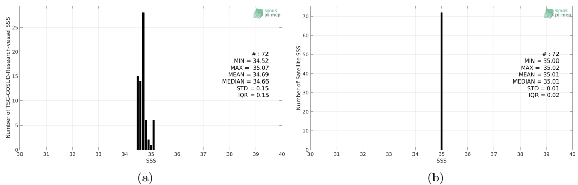
Figure 2: Histograms of SSS from TSG-GOSUD-Research-vessel (a) and SMAP-L3-JPL-V4.3-MONTHLY-60KM (b) considering all match-up pairs per bins of 0.1 over the Roaring Forties and Furious Fifties Pi-MEP region and for the full satellite product period.
