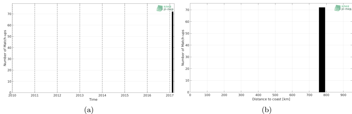
Figure 1: Number of match-ups between TSG-GOSUD-Research-vessel and SMAP-L3-JPL-V4.2-8DAY-RUNNING-60KM SSS as a function of time (a) and as function of the distance to coast (b) over the Roaring Forties and Furious Fifties Pi-MEP region and for the full satellite product period.
