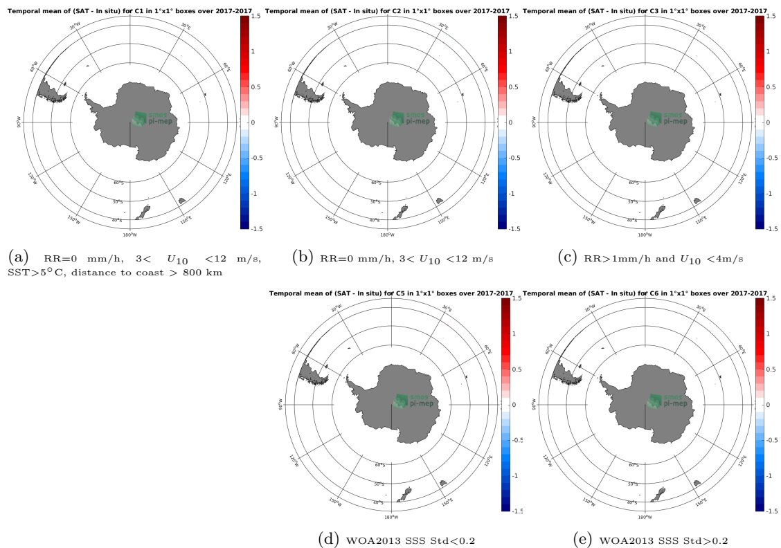
Figure 12: Temporal mean gridded over spatial boxes of size 1^\circ \times 1^\circ of \Delta SSS (SMAP-L3-JPL-V4.2-8DAY-RUNNING-60KM - TSG-GOSUD-Research-vessel) for 5 different subdatasets corresponding to: RR=0 mm/h, 3 < U_{10} < 12 m/s, SST > 5^\circ\text{C} , distance to coast > 800 km (a), RR=0 mm/h, 3 < U_{10} < 12 m/s (b), RR > 1 mm/h and U_{10} < 4 m/s (c), WOA2013 SSS Std < 0.2 (d), WOA2013 SSS Std > 0.2 (e).
