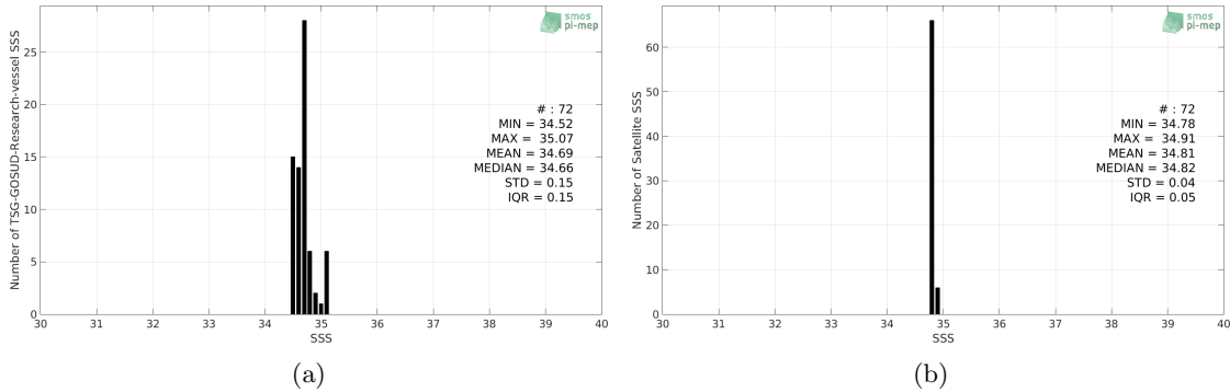
Figure 2: Histograms of SSS from TSG-GOSUD-Research-vessel (a) and SMAP-L3-JPL-V4.2-8DAY-RUNNING-60KM (b) considering all match-up pairs per bins of 0.1 over the Roaring Forties and Furious Fifties Pi-MEP region and for the full satellite product period.
