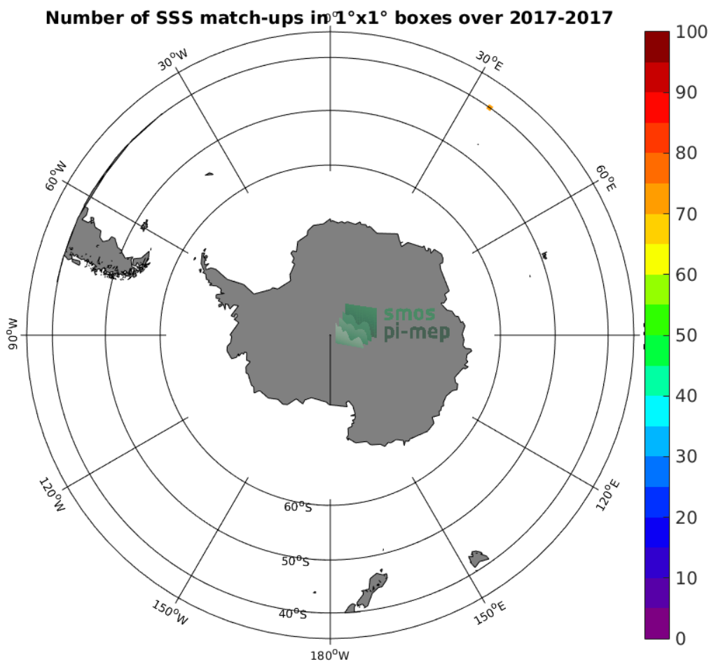
Figure 4: Number of SSS match-ups between TSG-GOSUD-Research-vessel SSS and the SMAP-L3-JPL-V4.2-8DAY-RUNNING-60KM SSS product for the Roaring Forties and Furious Fifties Pi-MEP region over 1°x1° boxes and for the full satellite product period.
