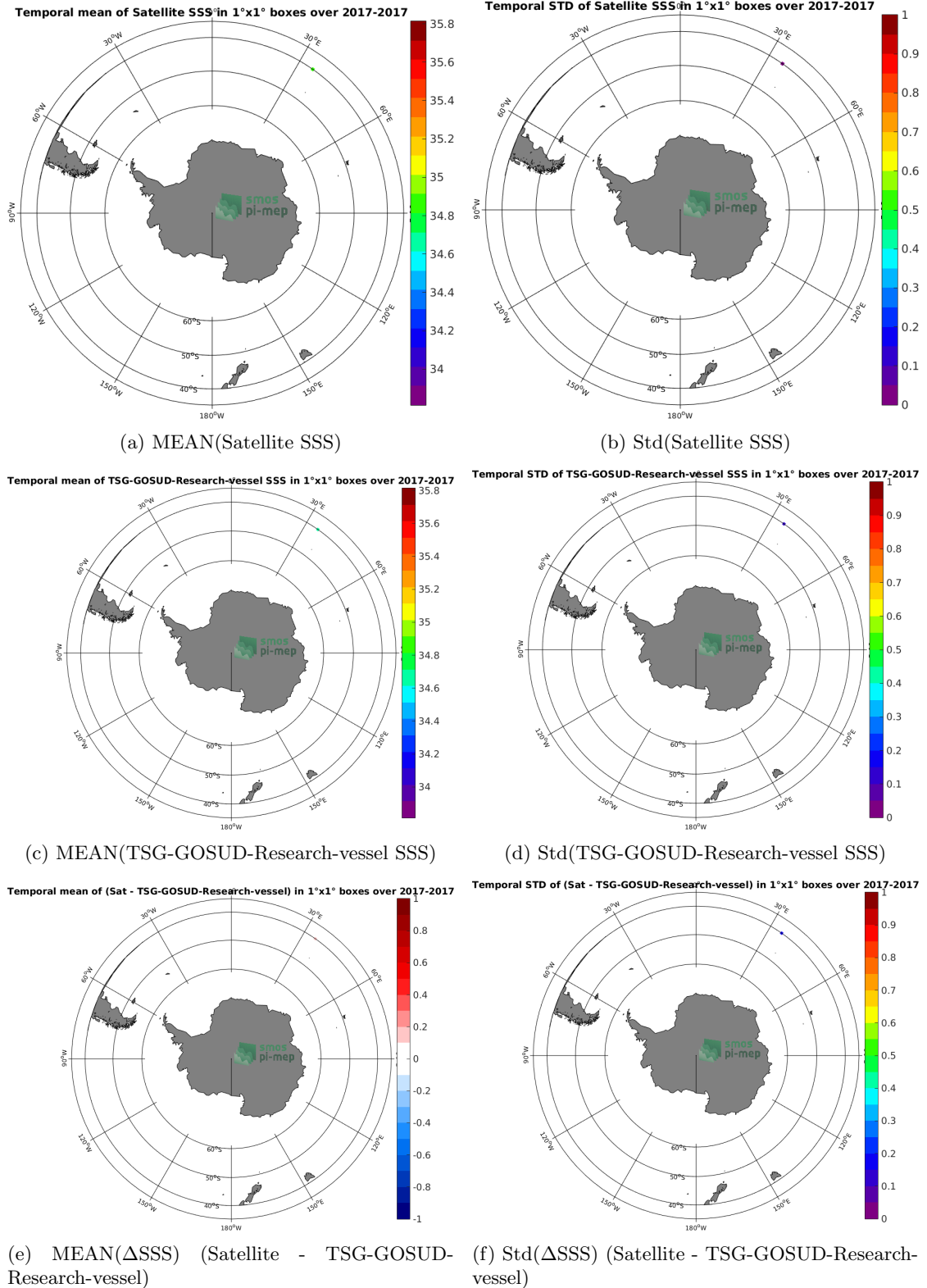
Figure 6: Temporal mean (left) and Std (right) of SSS from SMAP-L3-JPL-V4.2-8DAY-RUNNING-60KM (top), TSG-GOSUD-Research-vessel (middle), and of \Delta SSS (Satellite - TSG-GOSUD-Research-vessel). Only match-up pairs are used to generate these maps.
