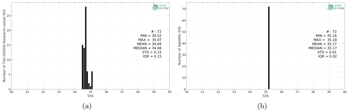
Figure 2: Histograms of SSS from TSG-GOSUD-Research-vessel (a) and SMAP-L3-JPL-V4.2-MONTHLY-60KM (b) considering all match-up pairs per bins of 0.1 over the Roaring Forties and Furious Fifties Pi-MEP region and for the full satellite product period.
