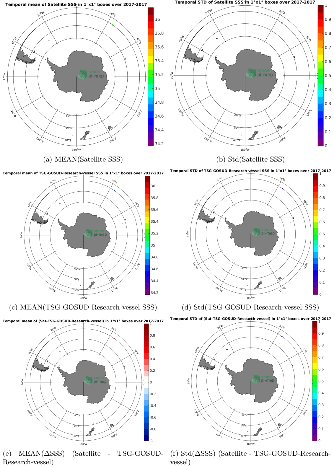
Figure 6: Temporal mean (left) and Std (right) of SSS from SMAP-L3-JPL-V4.2-MONTHLY-60KM (top), TSG-GOSUD-Research-vessel (middle), and of \Delta SSS (Satellite - TSG-GOSUD-Research-vessel). Only match-up pairs are used to generate these maps.
