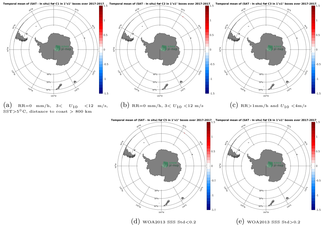
Figure 12: Temporal mean gridded over spatial boxes of size 1^\circ \times 1^\circ of \Delta SSS (SMAP-L3-JPL-V4.2-MONTHLY-60KM - TSG-GOSUD-Research-vessel) for 5 different subdatasets corresponding to: RR=0 mm/h, 3 < U_{10} < 12 m/s, SST > 5^\circ\text{C} , distance to coast > 800 km (a), RR=0 mm/h, 3 < U_{10} < 12 m/s (b), RR > 1 mm/h and U_{10} < 4 m/s (c), WOA2013 SSS Std < 0.2 (d), WOA2013 SSS Std > 0.2 (e).
