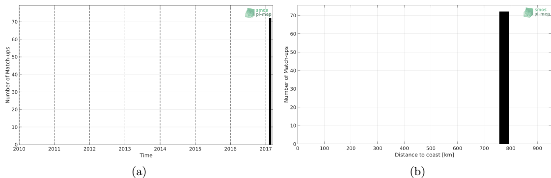
Figure 1: Number of match-ups between TSG-GOSUD-Research-vessel and SMAP-L3-JPL-V4.2-MONTHLY-60KM SSS as a function of time (a) and as function of the distance to coast (b) over the Roaring Forties and Furious Fifties Pi-MEP region and for the full satellite product period.
