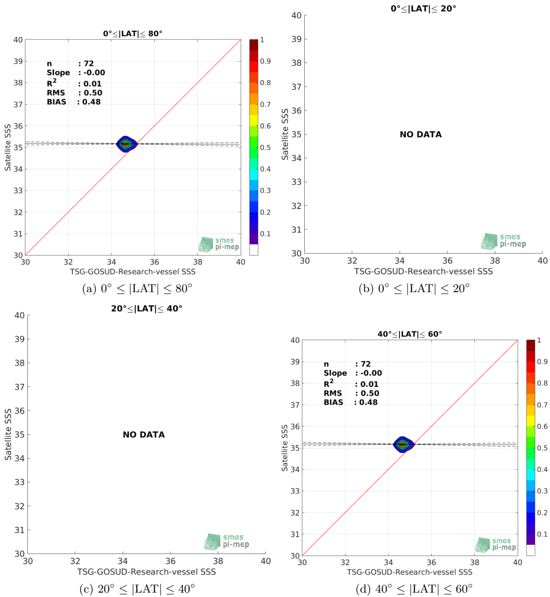
Figure 9: Contour maps of the concentration of SMAP-L3-JPL-V4.2-MONTHLY-60KM SSS (y-axis) versus TSG-GOSUD-Research-vessel SSS (x-axis) at match-up pairs for different latitude bands. For each plot, the red line shows x=y . The black thin and dashed lines indicate a linear fit through the data cloud and the \pm 95\% confidence levels, respectively. The number match-up pairs n , the slope and R^2 coefficient of the linear fit, the root mean square (RMS) and the mean bias between satellite and in situ data are indicated for each latitude band in each plots.
