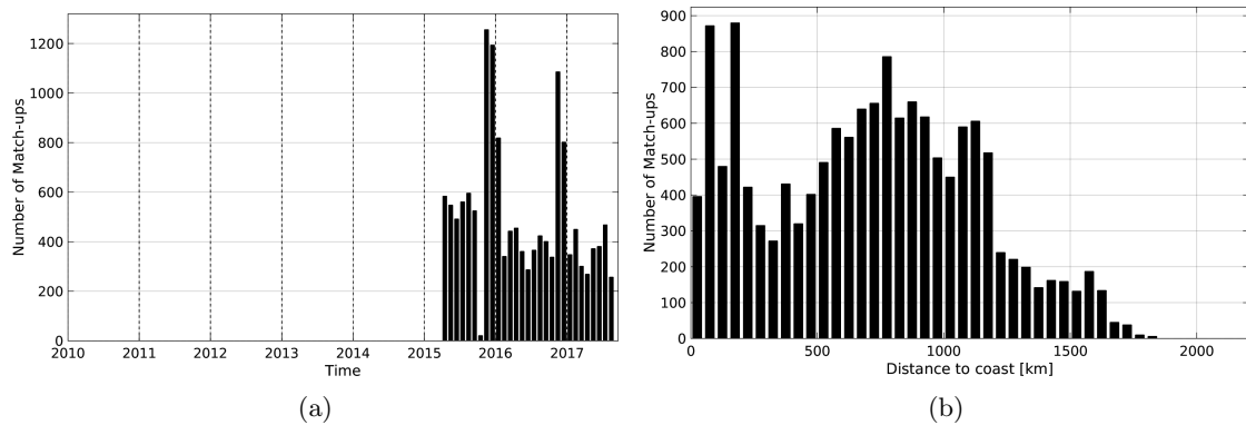
Figure 1: Number of match-ups between Sea mammals and SMAP-L3-JPL-V4-8DAY-RUNNING-60KM SSS as a function of time (a) and as function of the distance to coast (b) over the Roaring Forties and Furious Fifties Pi-MEP region and for the full satellite product period.
