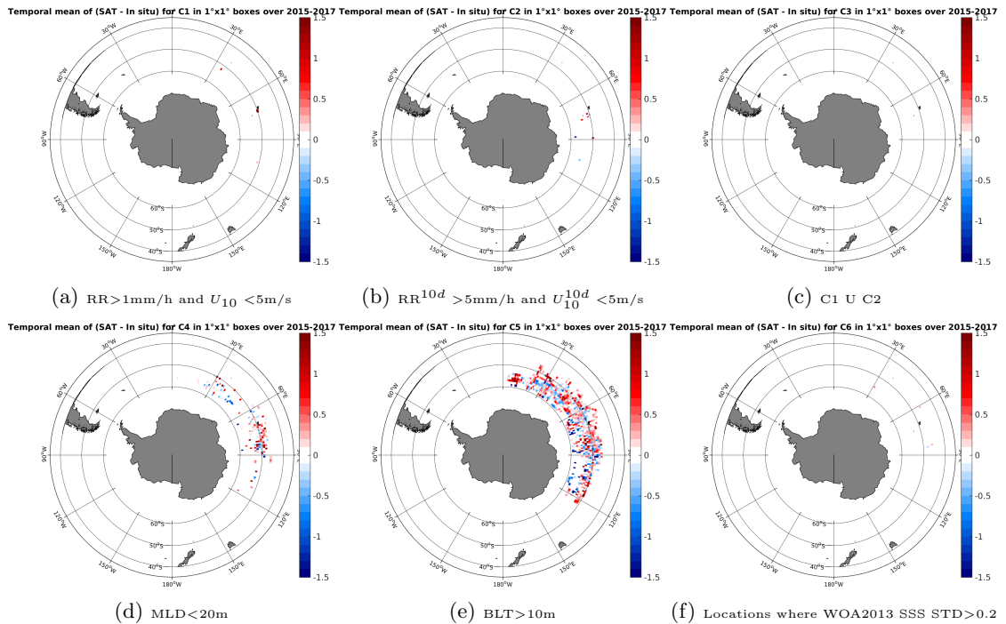
Figure 12: Temporal mean gridded over spatial boxes of size 1^\circ \times 1^\circ of \Delta SSS (SMAP-L3-JPL-V4-8DAY-RUNNING-60KM - Sea mammals) for 6 different subdatasets corresponding to: RR > 1\text{mm/h} and U_{10} < 5\text{m/s} (a), RR^{10d} > 5\text{mm/h} and U_{10}^{10d} < 5\text{m/s} (b), C1 U C2 (c), MLD < 20\text{m} (d), BLT > 10\text{m} (e), Locations where WOA2013 SSS STD > 0.2 (f).
