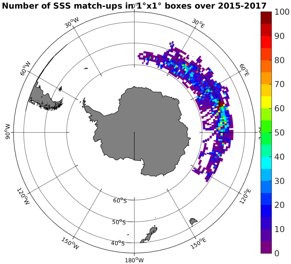
Figure 4: Number of SSS match-ups between Sea mammals SSS and the SMAP-L3-JPL-V4-8DAY-RUNNING-60KM SSS product for the Roaring Forties and Furious Fifties Pi-MEP region over 1°x1° boxes and for the full satellite product period.
