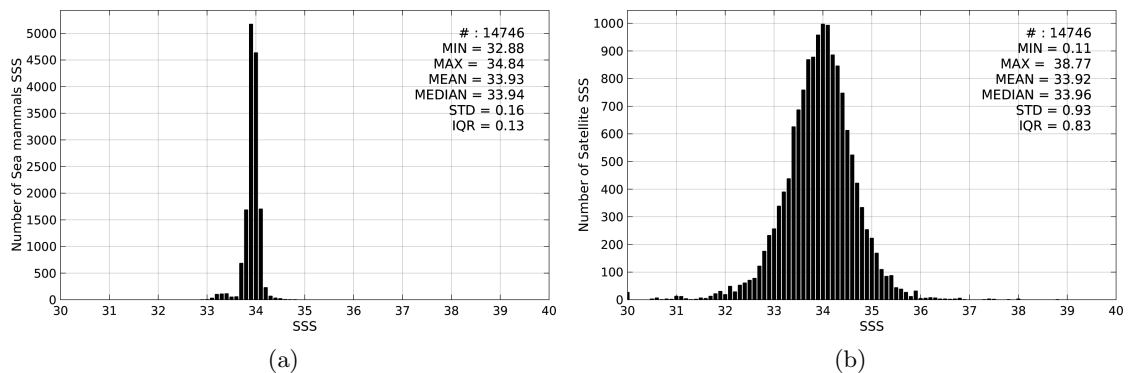
Figure 2: Histograms of SSS from Sea mammals (a) and SMAP-L3-JPL-V4-8DAY-RUNNING-60KM (b) considering all match-up pairs per bins of 0.1 over the Roaring Forties and Furious Fifties Pi-MEP region and for the full satellite product period.
