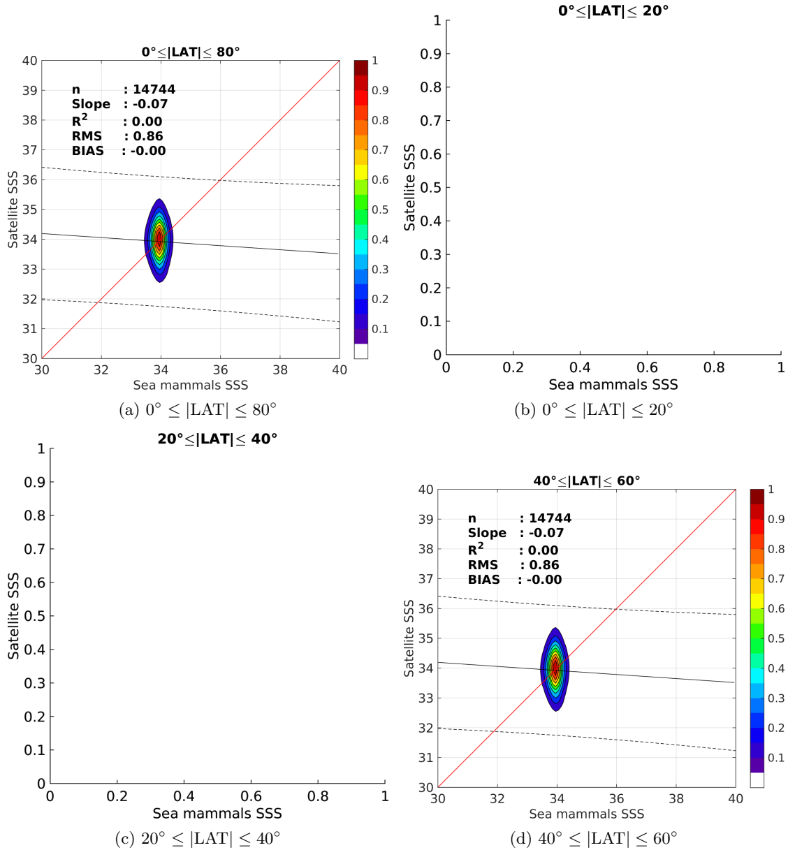
Figure 9: Contour maps of the concentration of SMAP-L3-JPL-V4-8DAY-RUNNING-60KM SSS (y-axis) versus Sea mammals SSS (x-axis) at match-up pairs for different latitude bands. For each plot, the red line shows x=y . The black thin and dashed lines indicate a linear fit through the data cloud and the \pm 95\% confidence levels, respectively. The number match-up pairs n , the slope and R^2 coefficient of the linear fit, the root mean square (RMS) and the mean bias between satellite and in situ data are indicated for each latitude band in each plots.
