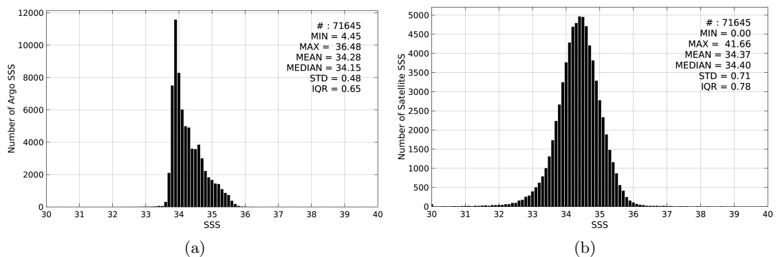
Figure 2: Histograms of SSS from Argo (a) and SMAP-L3-JPL-V4-8DAY-RUNNING-60KM (b) considering all match-up pairs per bins of 0.1 over the Roaring Forties and Furious Fifties Pi-MEP region and for the full satellite product period.
