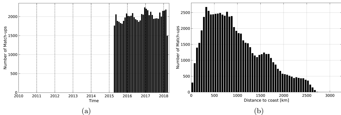
Figure 1: Number of match-ups between Argo and SMAP-L3-JPL-V4-8DAY-RUNNING-60KM SSS as a function of time (a) and as function of the distance to coast (b) over the Roaring Forties and Furious Fifties Pi-MEP region and for the full satellite product period.
