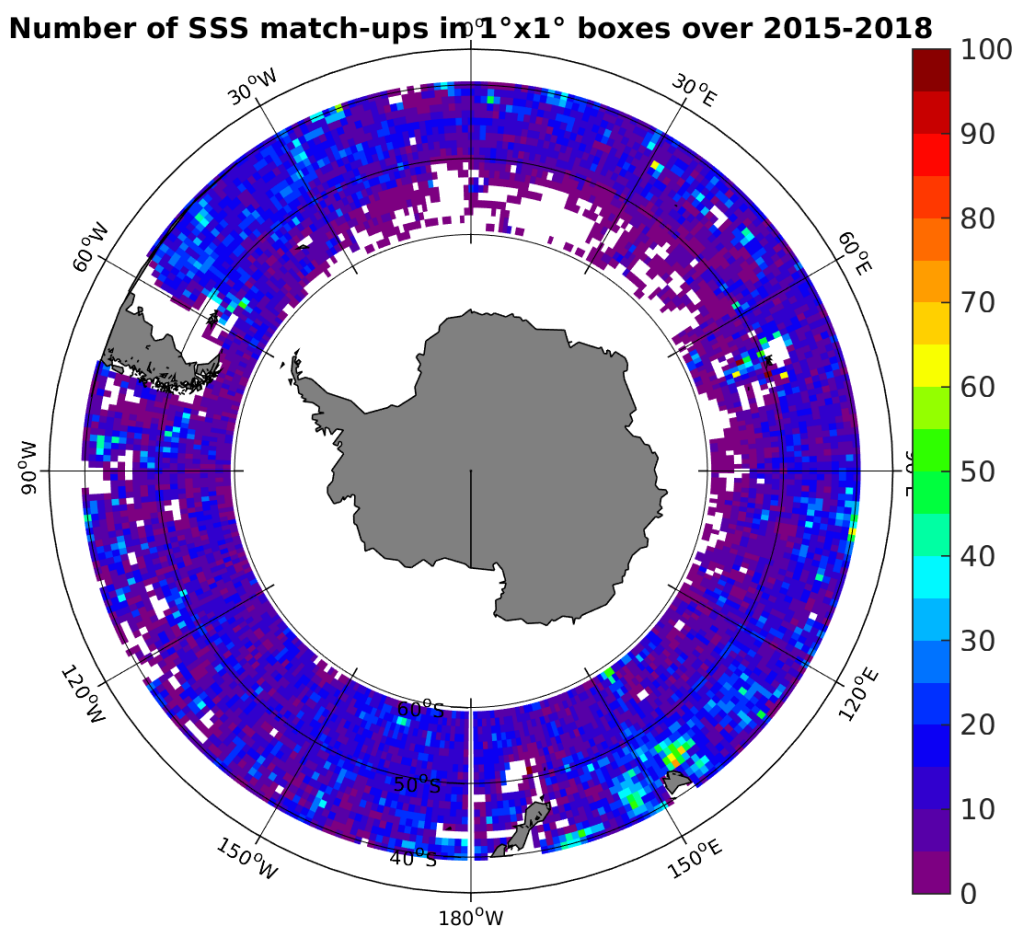
Figure 4: Number of SSS match-ups between Argo SSS and the SMAP-L3-JPL-V4-8DAY-RUNNING-60KM SSS product for the Roaring Forties and Furious Fifties Pi-MEP region over 1^\circ \times 1^\circ boxes and for the full satellite product period.
