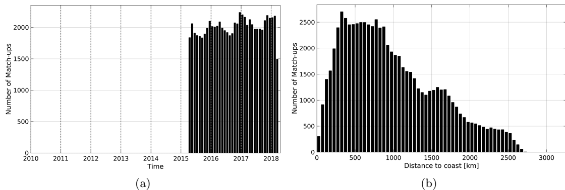
Figure 1: Number of match-ups between Argo and SMAP-L3-JPL-V4-MONTHLY-60KM SSS as a function of time (a) and as function of the distance to coast (b) over the Roaring Forties and Furious Fifties Pi-MEP region and for the full satellite product period.
