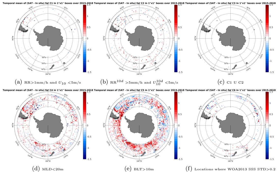
Figure 12: Temporal mean gridded over spatial boxes of size 1^\circ \times 1^\circ of \Delta SSS (SMAP-L3-JPL-V4-MONTHLY-60KM - Argo) for 6 different subdatasets corresponding to: RR > 1\text{mm/h} and U_{10} < 5\text{m/s} (a), RR^{10d} > 5\text{mm/h} and U_{10}^{10d} < 5\text{m/s} (b), C1 U C2 (c), MLD < 20\text{m} (d), BLT > 10\text{m} (e), Locations where WOA2013 SSS STD > 0.2 (f).
