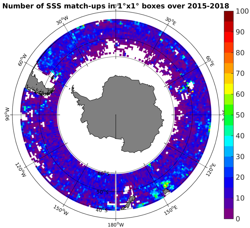
Figure 4: Number of SSS match-ups between Argo SSS and the SMAP-L3-JPL-V4-MONTHLY-60KM SSS product for the Roaring Forties and Furious Fifties Pi-MEP region over 1^\circ \times 1^\circ boxes and for the full satellite product period.
