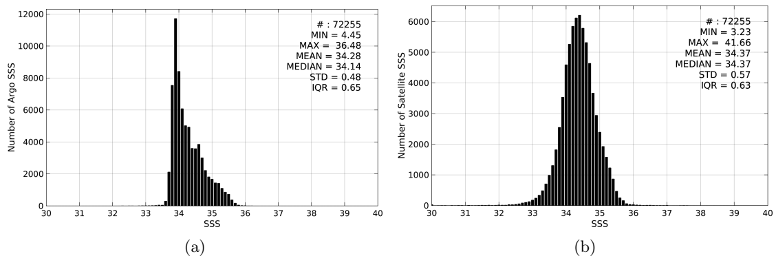
Figure 2: Histograms of SSS from Argo (a) and SMAP-L3-JPL-V4-MONTHLY-60KM (b) considering all match-up pairs per bins of 0.1 over the Roaring Forties and Furious Fifties Pi-MEP region and for the full satellite product period.
