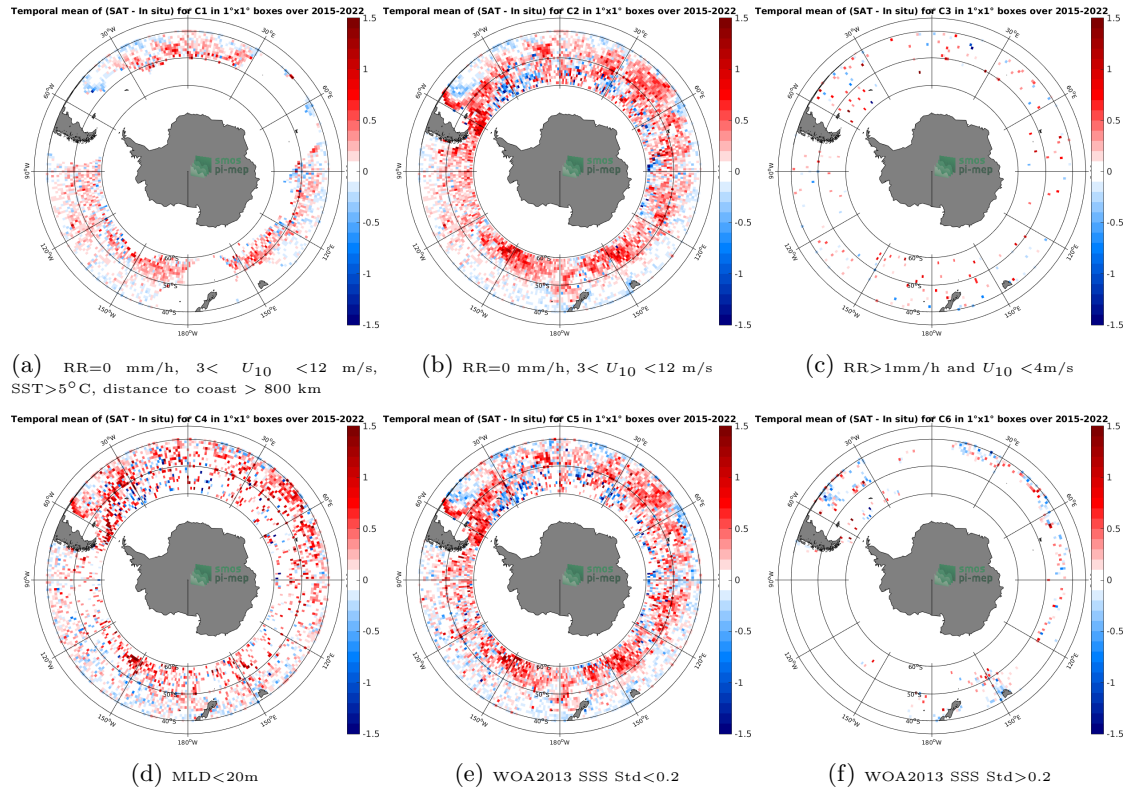
Figure 12: Temporal mean gridded over spatial boxes of size 1^{\circ}\times 1^{\circ} of \Delta\text{SSS} (SMAP SSS L2-AVERAGED v5.0 (JPL) - Argo) for 6 different subdatasets corresponding to:RR=0 mm/h, 3 < U_{10} < 12 m/s, SST >5^{\circ}\text{C} , distance to coast > 800 km (a), RR=0 mm/h, 3 < U_{10} < 12 m/s (b), RR >1 mm/h and U_{10} < 4 m/s (c),MLD <20 m (d),WOA2013 SSS Std <0.2 (e),WOA2013 SSS Std >0.2 (f).
