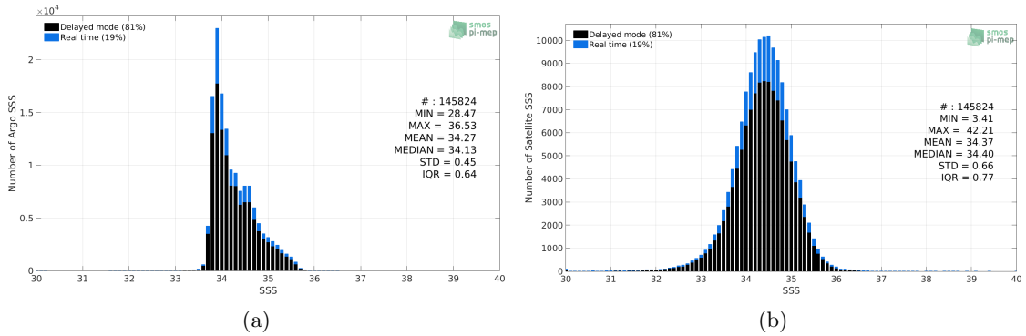
Figure 2: Histograms of SSS from Argo (a) and SMAP SSS L2-AVERAGED v5.0 (JPL) (b) considering all match-up pairs per bins of 0.1 over the Roaring Forties and Furious Fifties Pi-MEP region and for the full satellite product period.
