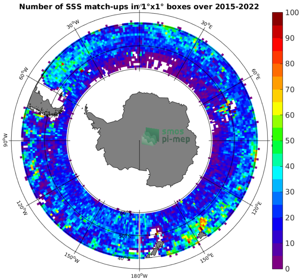
Figure 4: Number of SSS match-ups between Argo SSS and the SMAP SSS L2-AVERAGED v5.0 (JPL) SSS product for the Roaring Forties and Furious Fifties Pi-MEP region over 1^\circ \times 1^\circ boxes and for the full satellite product period.
