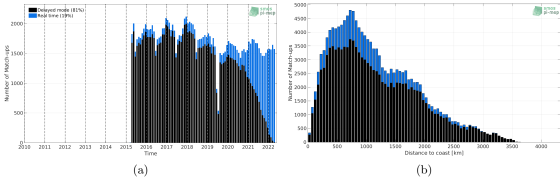
Figure 1: Number of match-ups between Argo and SMAP SSS L2-AVERAGED v5.0 (JPL) SSS as a function of time (a) and as function of the distance to coast (b) over the Roaring Forties and Furious Fifties Pi-MEP region and for the full satellite product period.
