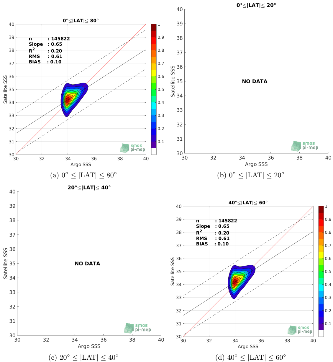
Figure 9: Contour maps of the concentration of SMAP SSS L2-AVERAGED v5.0 (JPL) SSS (y-axis) versus Argo SSS (x-axis) at match-up pairs for different latitude bands. For each plot, the red line shows x=y . The black thin and dashed lines indicate a linear fit through the data cloud and the \pm 95\% confidence levels, respectively. The number match-up pairs n , the slope and R^2 coefficient of the linear fit, the root mean square (RMS) and the mean bias between satellite and in situ data are indicated for each latitude band in each plots.
