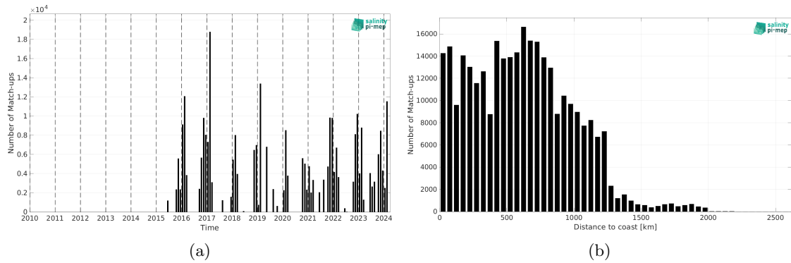
Figure 2: Number of match-ups between TSG (LEGOS-DM) and SMAP SSS L2 v6 (RSS) SSS as a function of time (a) and as function of the distance to coast (b) over the Roaring Forties and Furious Fifties Pi-MEP region and for the full satellite product period.
