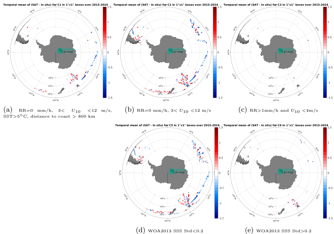
Figure 14: Temporal mean gridded over spatial boxes of size 1^\circ \times 1^\circ of \Delta SSS (SMAP SSS L2 v6 (RSS) - TSG (LEGOS-DM)) for 5 different subdatasets corresponding to: RR=0 mm/h, 3 < U_{10} < 12 m/s, SST > 5^\circ C , distance to coast > 800 km (a), RR=0 mm/h, 3 < U_{10} < 12 m/s (b), RR > 1 mm/h and U_{10} < 4 m/s (c), WOA2013 SSS Std < 0.2 (d), WOA2013 SSS Std > 0.2 (e).
