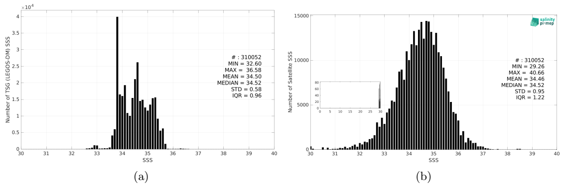
Figure 3: Histograms of SSS from TSG (LEGOS-DM) (a) and SMAP SSS L2 v6 (RSS) (b) considering all match-up pairs per bins of 0.1 over the Roaring Forties and Furious Fifties Pi-MEP region and for the full satellite product period.
