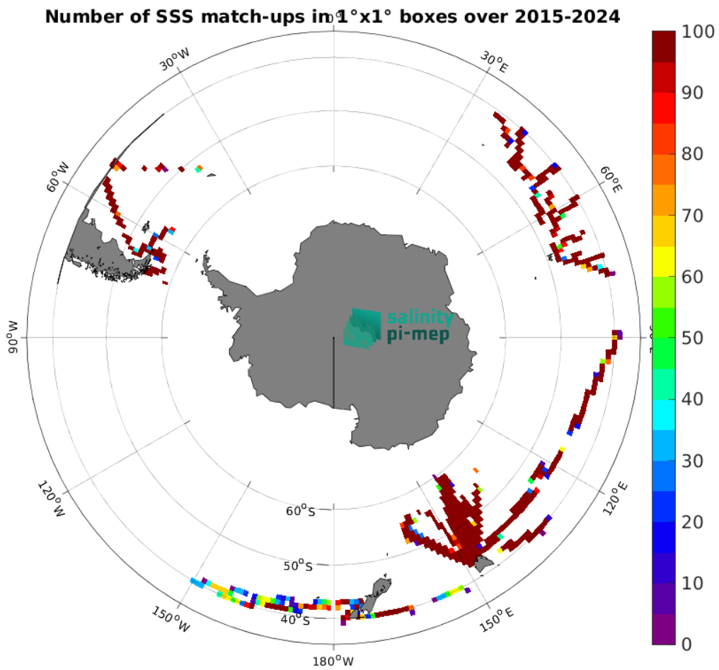
Figure 5: Number of SSS match-ups between TSG (LEGOS-DM) SSS and the SMAP SSS L2 v6 (RSS) SSS product for the Roaring Forties and Furious Fifties Pi-MEP region over 1^\circ \times 1^\circ boxes and for the full satellite product period.
