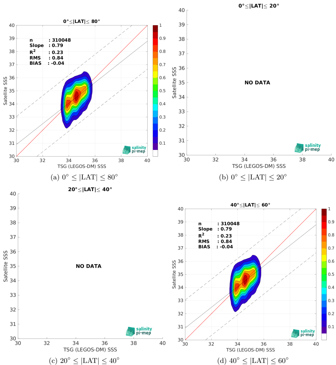
Figure 10: Contour maps of the concentration of SMAP SSS L2 v6 (RSS) SSS (y-axis) versus TSG (LEGOS-DM) SSS (x-axis) at match-up pairs for different latitude bands. For each plot, the red line shows x=y . The black thin and dashed lines indicate a linear fit through the data cloud and the \pm 95\% confidence levels, respectively. The number match-up pairs n , the slope and R^2 coefficient of the linear fit, the root mean square (RMS) and the mean bias between satellite and in situ data are indicated for each latitude band in each plot.
