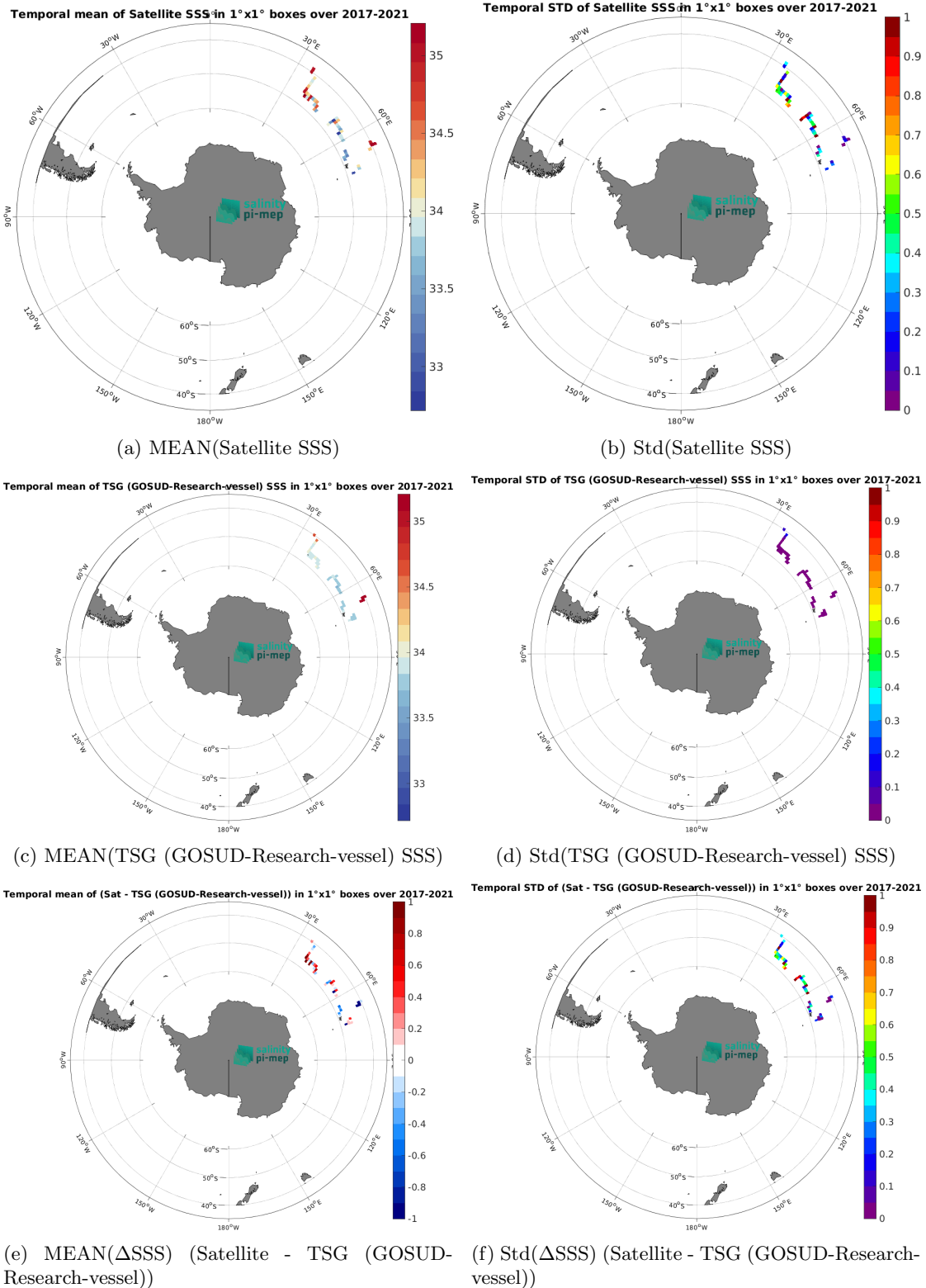
Figure 7: Temporal mean (left) and Std (right) of SSS from SMAP SSS L2 v6 (RSS) (top), TSG (GOSUD-Research-vessel) (middle), and of \Delta SSS (Satellite - TSG (GOSUD-Research-vessel)). Only match-up pairs are used to generate these 17 maps.
