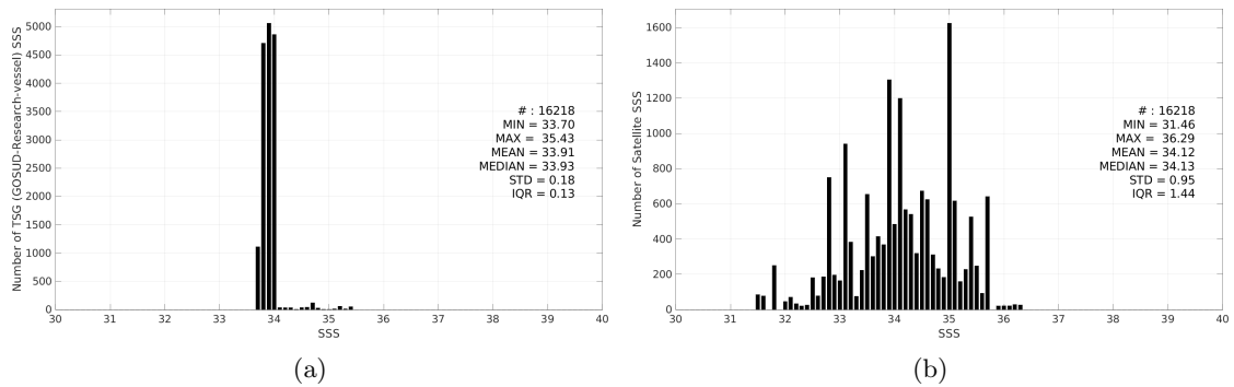
Figure 3: Histograms of SSS from TSG (GOSUD-Research-vessel) (a) and SMAP SSS L2 v6 (RSS) (b) considering all match-up pairs per bins of 0.1 over the Roaring Forties and Furious Fifties Pi-MEP region and for the full satellite product period.
