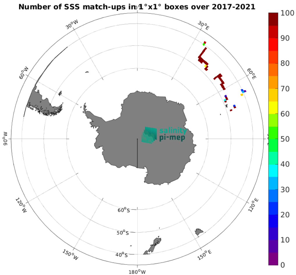
Figure 5: Number of SSS match-ups between TSG (GOSUD-Research-vessel) SSS and the SMAP SSS L2 v6 (RSS) SSS product for the Roaring Forties and Furious Fifties Pi-MEP region over 1^\circ \times 1^\circ boxes and for the full satellite product period.
